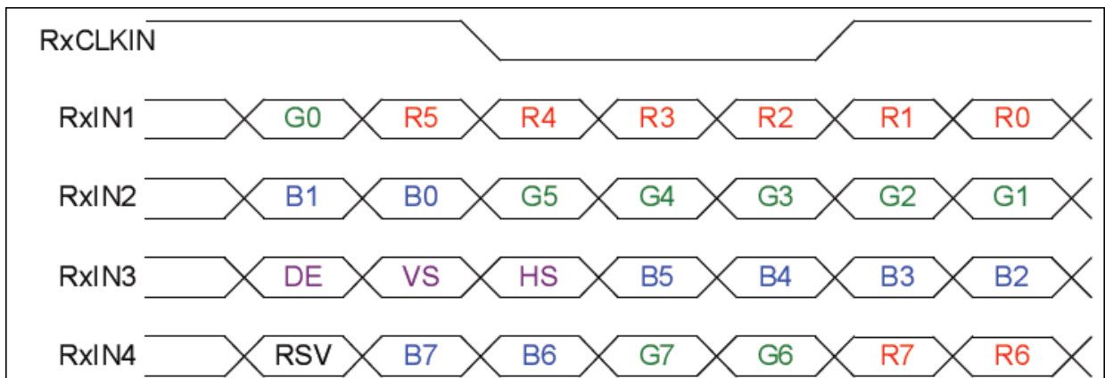
Figure 8 Timing Characteristics
