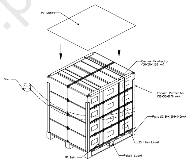
Figure. 7-2 Packing method
