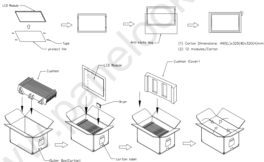
Figure. 7-1 Packing method
