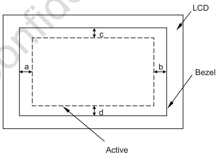
Figure 21 Module Dimension
