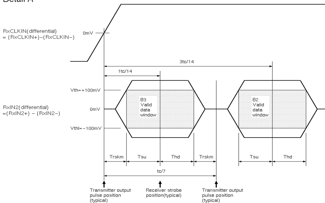
Figure 14 Timing Definition
