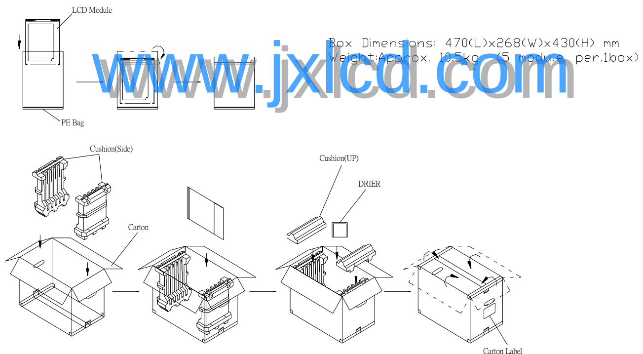
Figure. 8-1 Packing method
