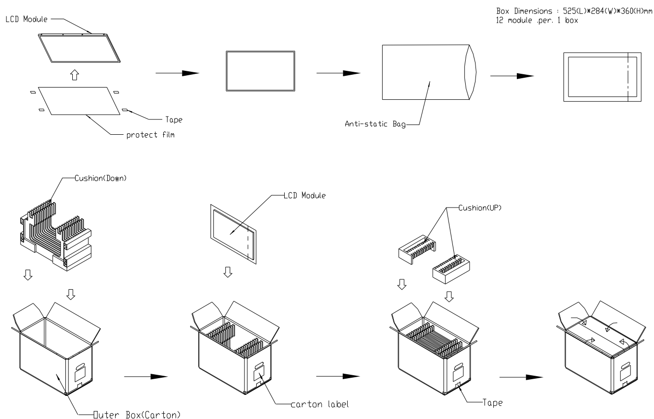
Figure. 7-1 Packing method
