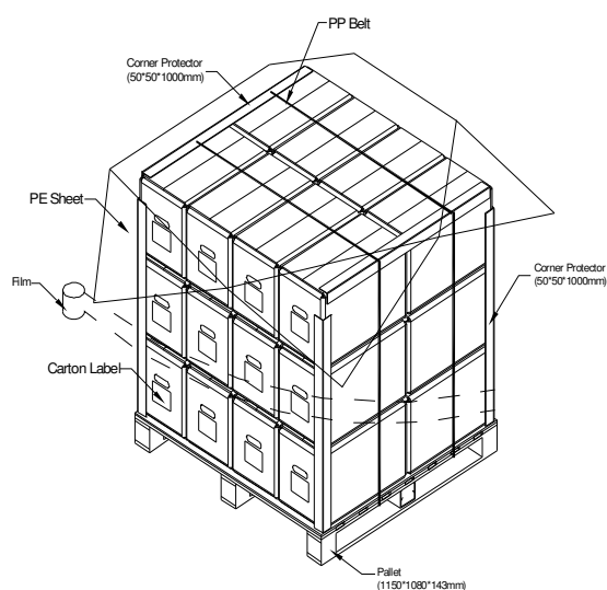
Figure. 7-2 Packing method
