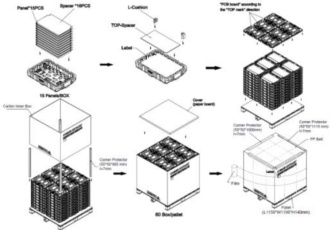
Figure. 8-1 Packing method
