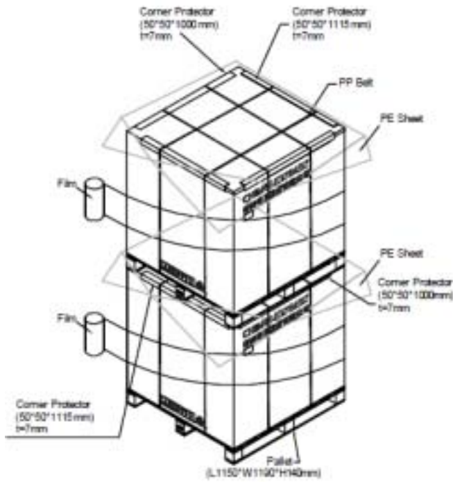
Figure. 8-2 Packing method
