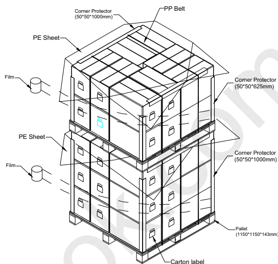
Figure. 8-2 Packing method
