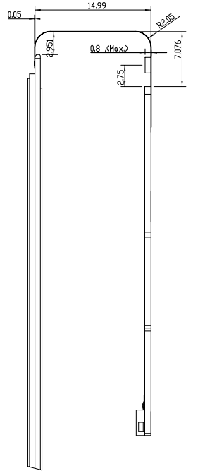
DETAIL B SCALE 4:1
