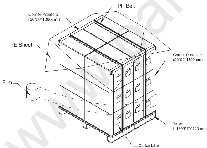
Figure. 8-3 Packing method
