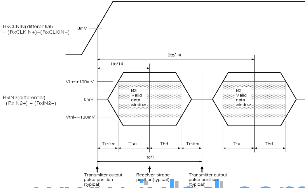
Figure 11 Timing Definition
