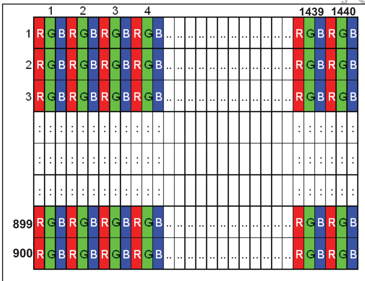
Figure 2 Pixel Format
