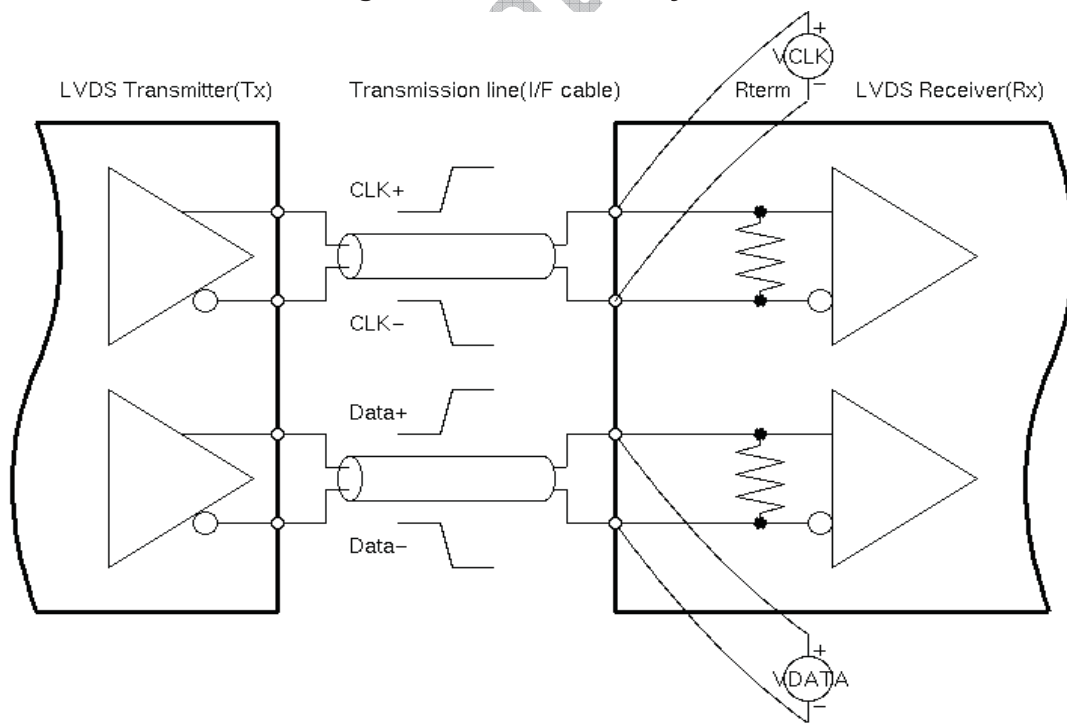
Figure 9 Measurement System
