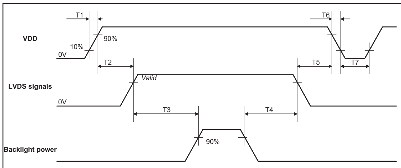
Figure 14 Power sequence
