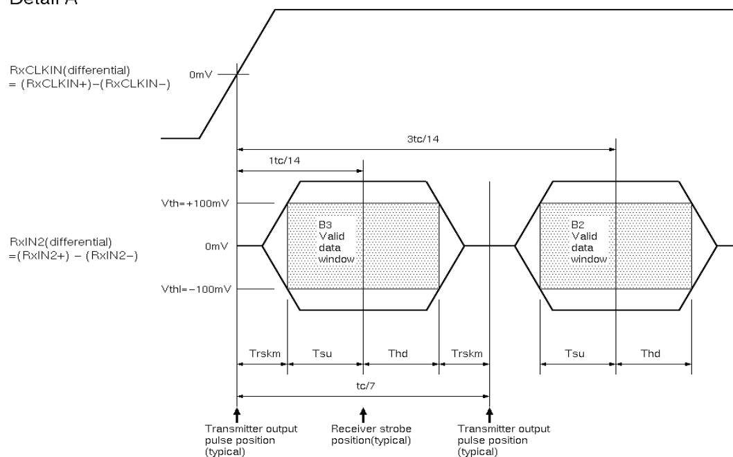
Figure 11 Timing Definition
