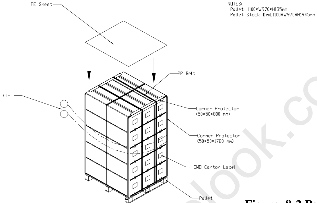
Figure. 8-2 Packing method
