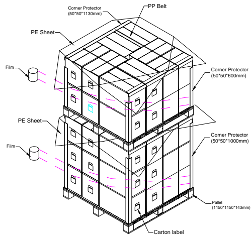
Figure. 8-2 Packing method
