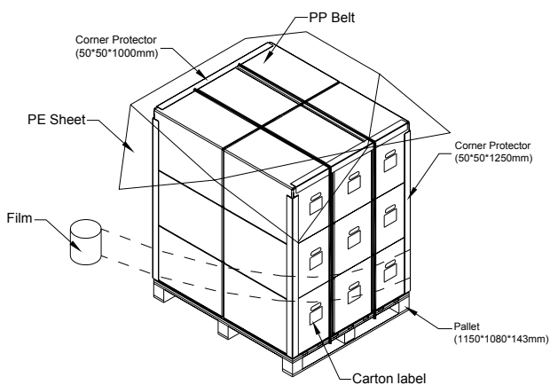
Figure. 8-3 Packing method
