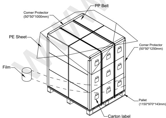
Figure. 8-3 Packing method
