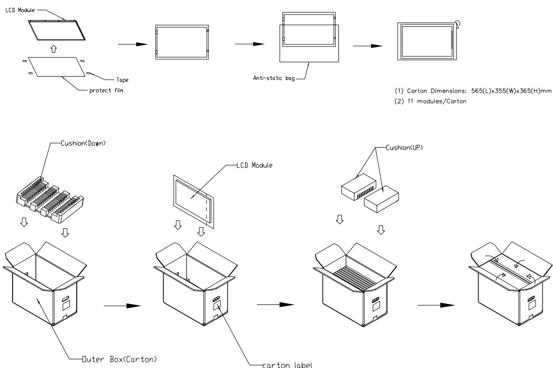
Figure. 7-1 Packing method
