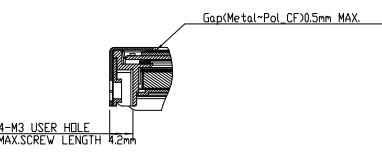
SECTION USER_HOLE_H-USER_HOLE_H SCALE 2:1
