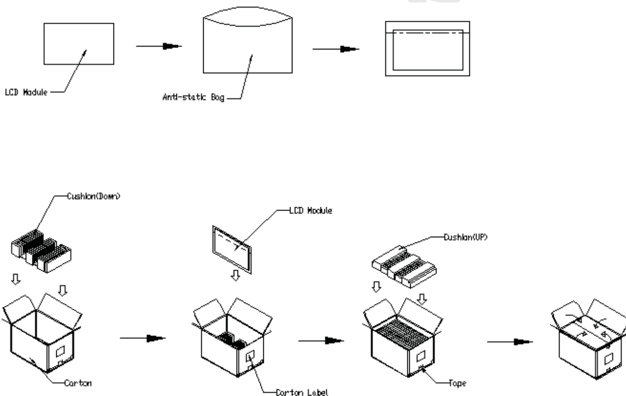
Figure. 7-1 Packing method
