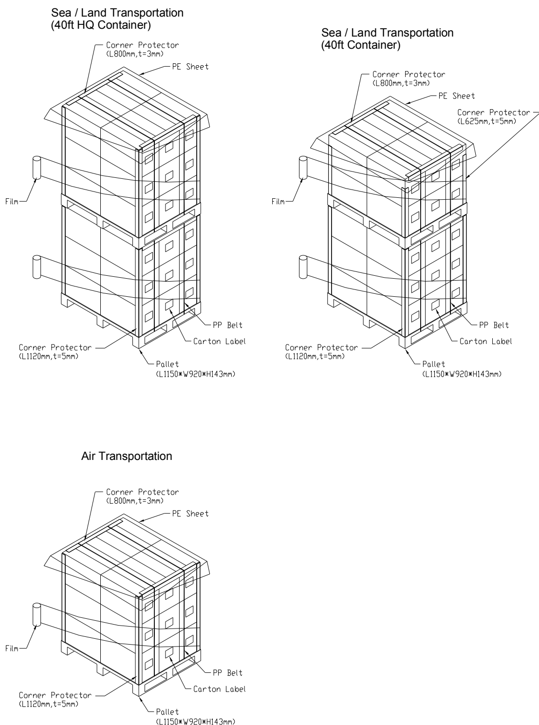
Figure. 8-2 Packing method
