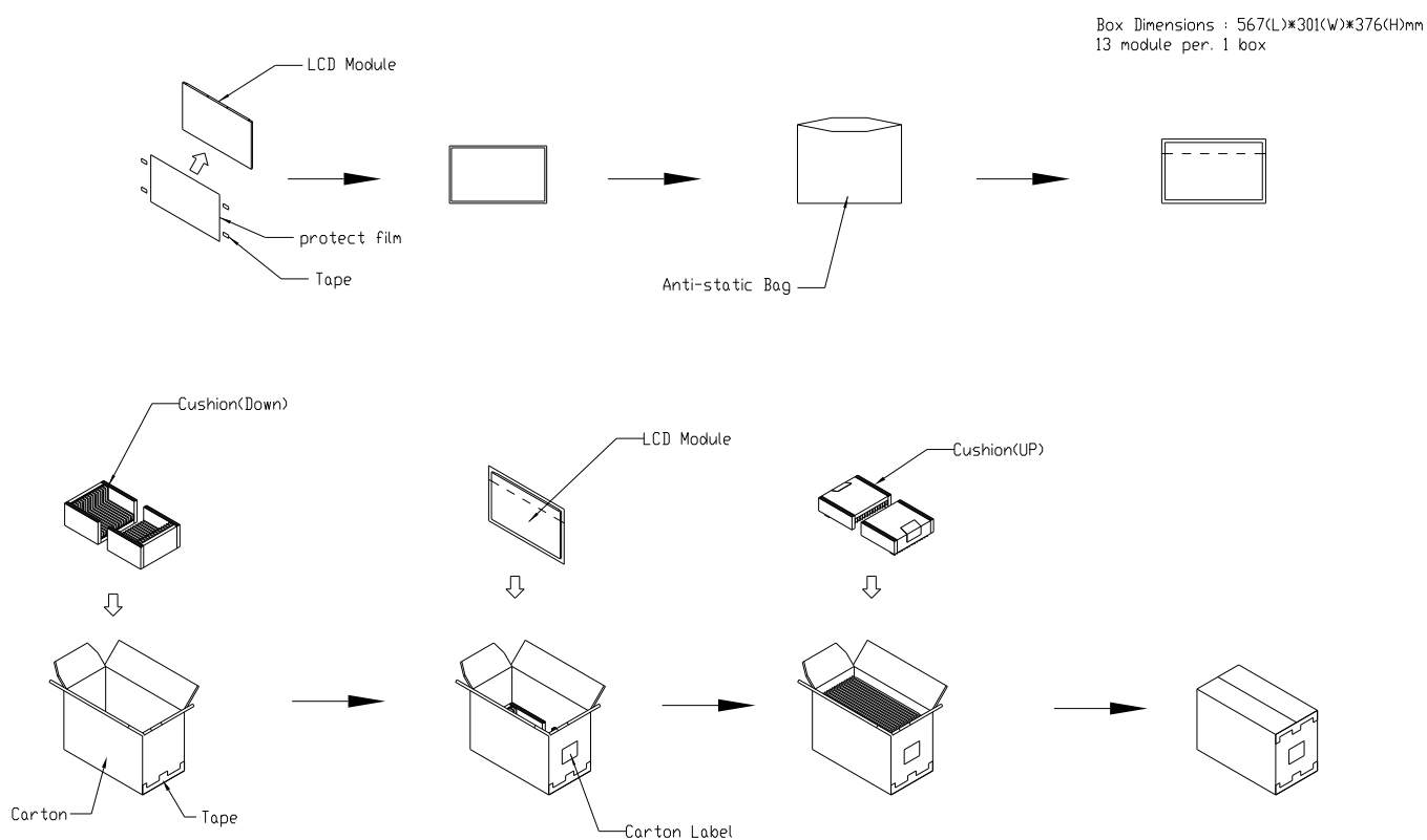
Figure. 8-1 Packing method
