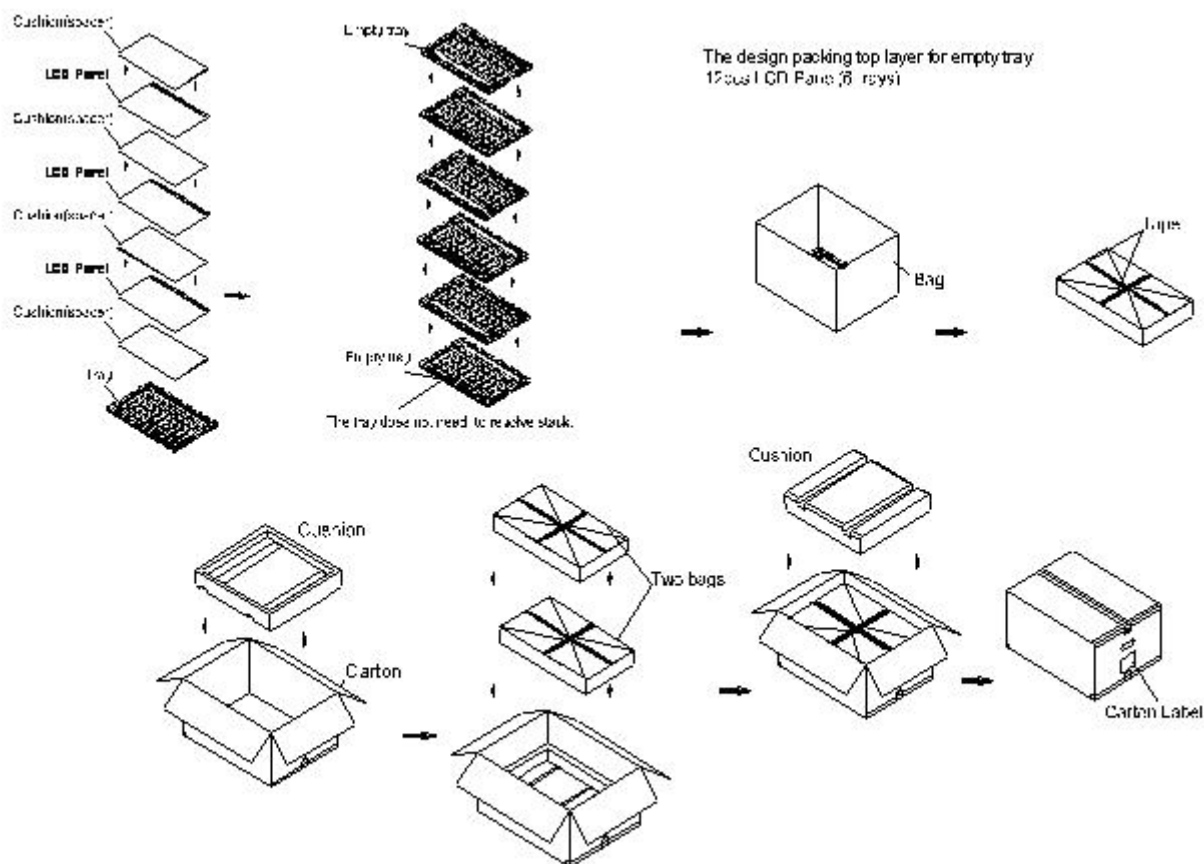
Figure. 8-1 Packing method
