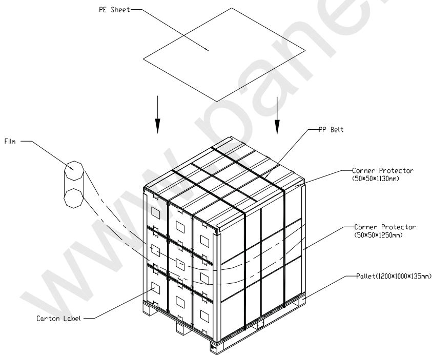
Figure. 8-3 Packing method
