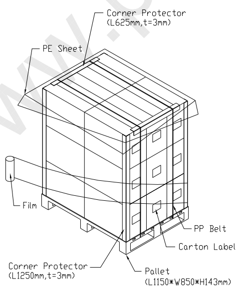
Figure. 7-2 Packing method
