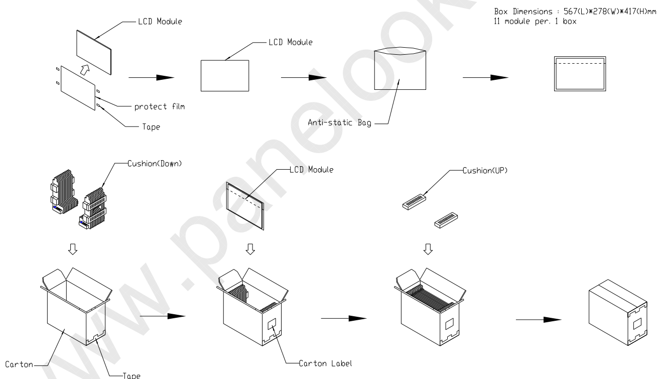
Figure. 7-1 Packing method
