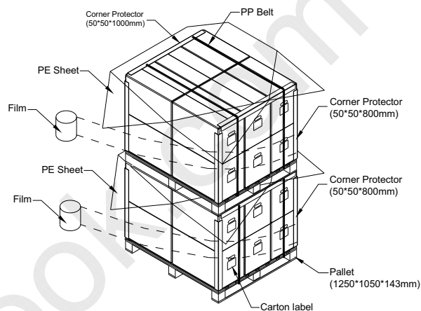
Figure 8-2 Packing method
