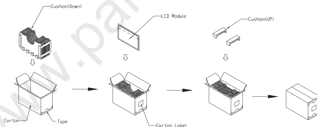
Figure. 7-1 Packing method
