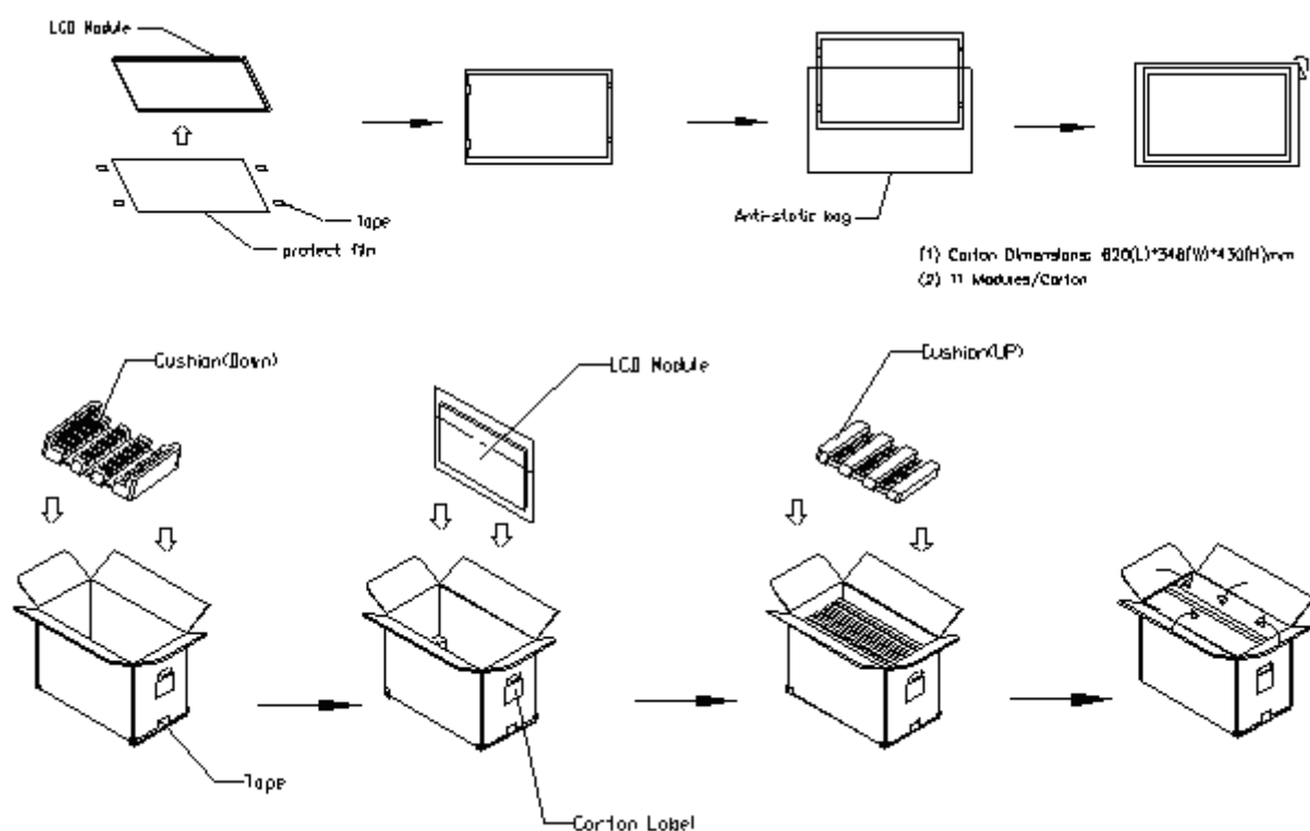
Figure. 7-1 Packing method
