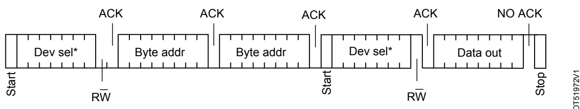
Figure 13. Random read DTI register
