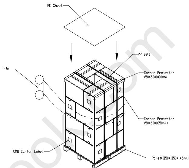
Figure. 8-2 Packing method
