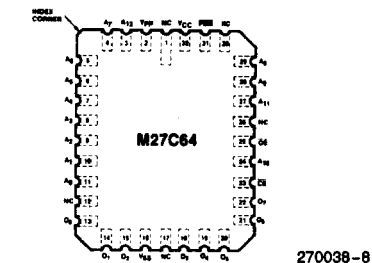
Figure 2. Pin Configurations
