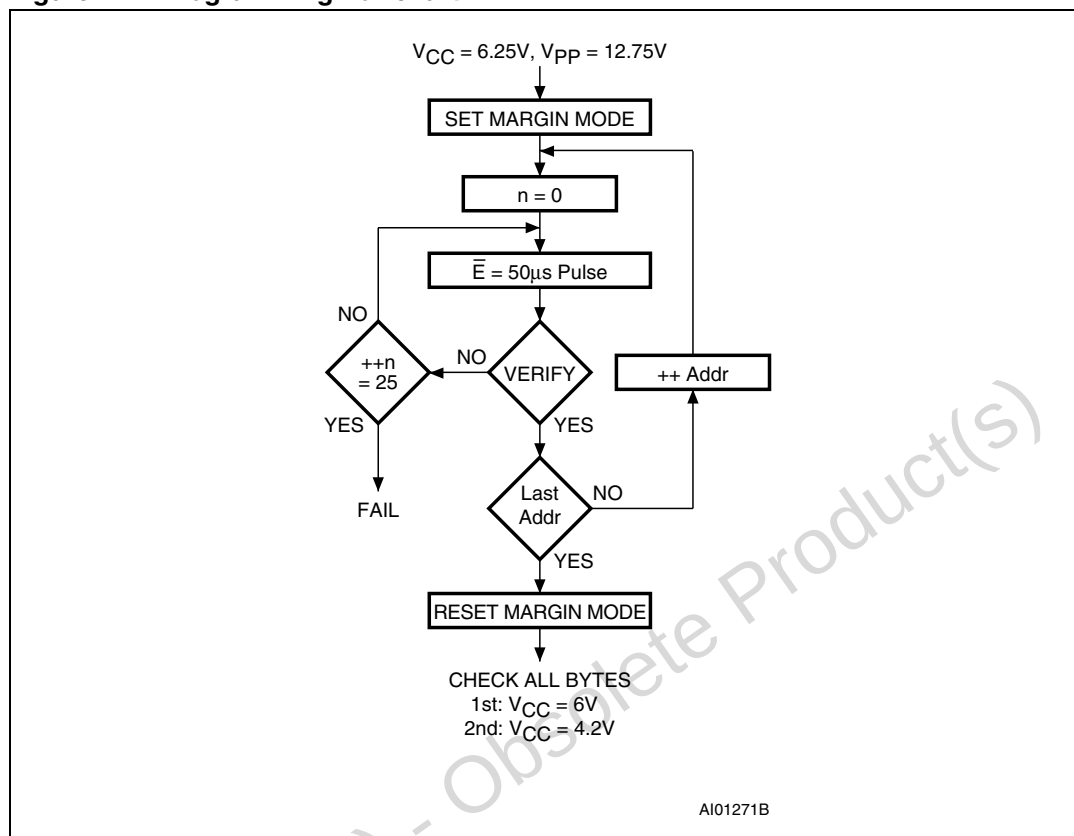
Figure 4. Programming flowchart
