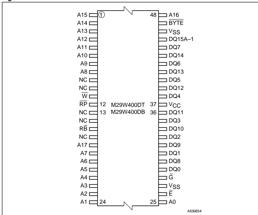
Figure 3. TSOP connections
