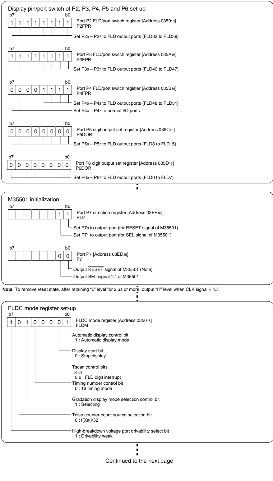
Figure 2.7.20. Set-up procedure for FLD automatic display (1)
