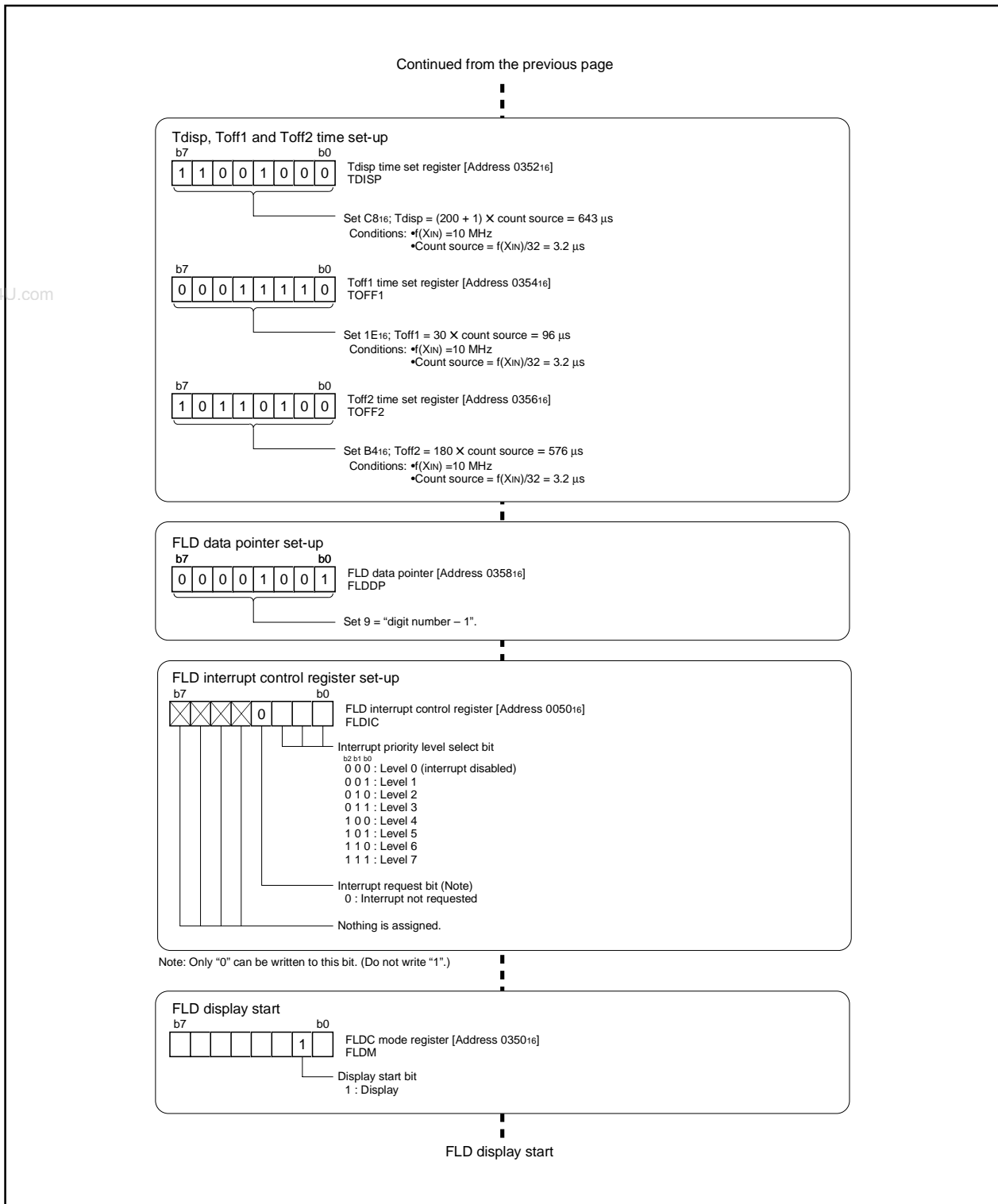
Figure 2.7.13. Set-up procedure for FLD automatic display (2)
