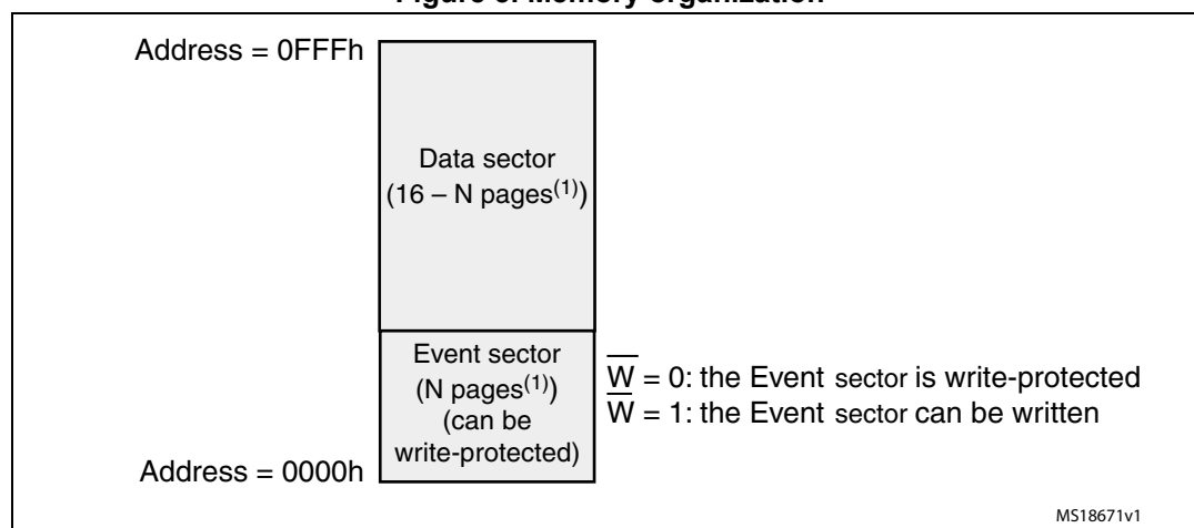
Figure 5. Memory organization
