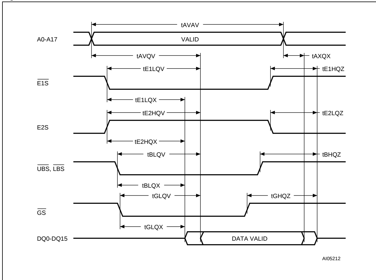
Figure 14. SRAM Read AC Waveforms, \overline{\text{E1S}} , \overline{\text{E2S}} or \overline{\text{GS}} Controlled
