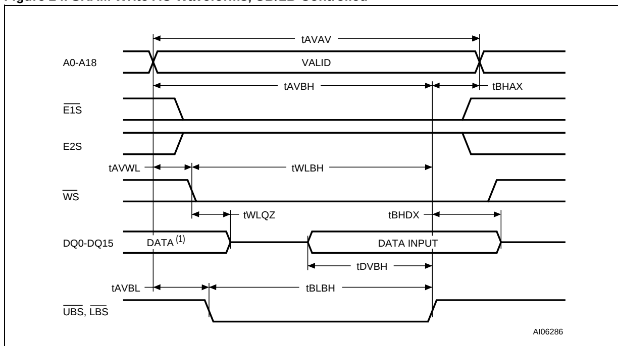
Figure 24. SRAM Write AC Waveforms, \overline{UB/LB} Controlled
