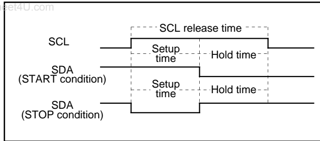
Fig. 23. START condition/STOP condition detecting timing diagram
