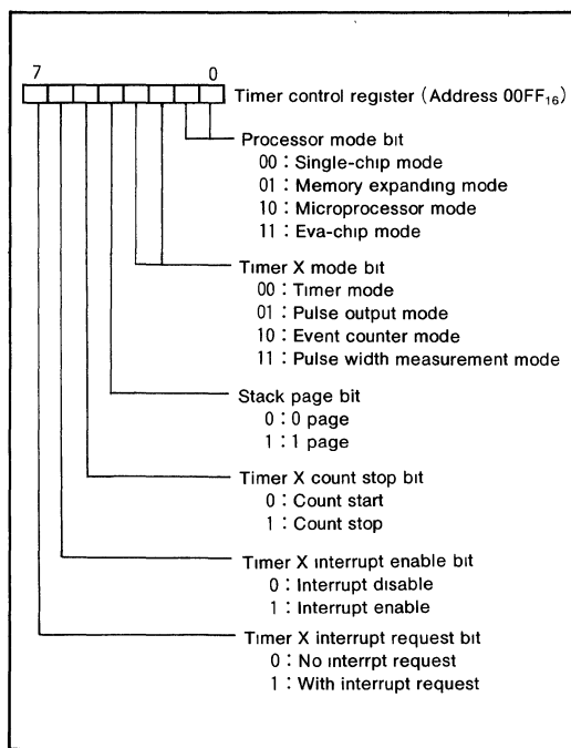
Fig.1 Structure of timer control register
