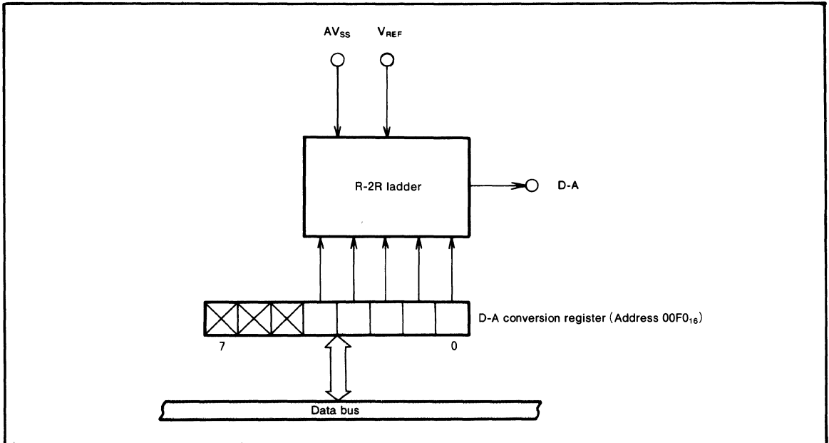
Fig.13 Block diagram of D-A converter
