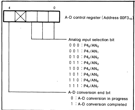
Fig.12 Structure of A-D control register
