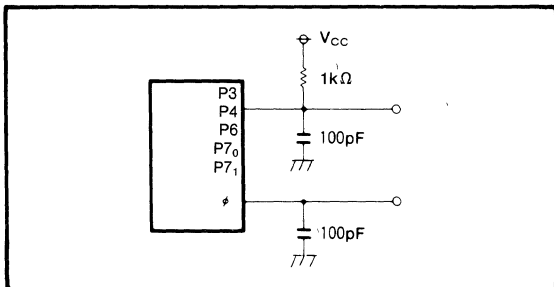
Fig.24 Ports P3, P4, P6, P7 0 , P7 1 test circuit
