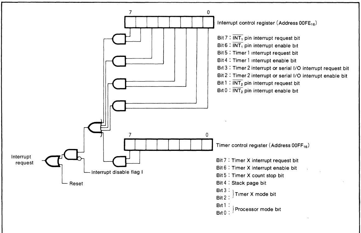
Fig.4 Interrupt control
