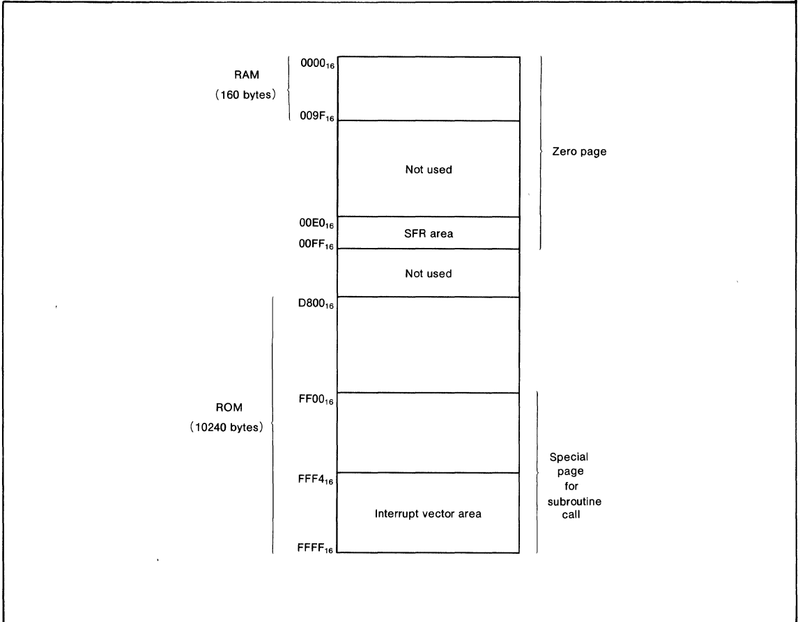
Fig.2 Memory map
