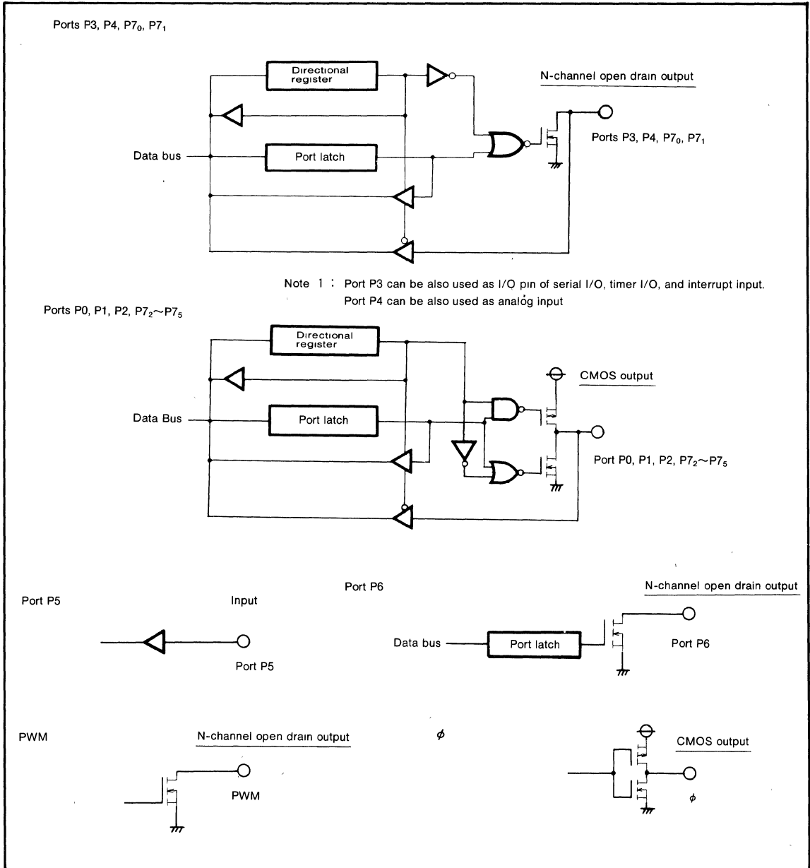
Fig.18 Block diagram of ports P0~P7 (single-chip mode), and output format of \phi .
