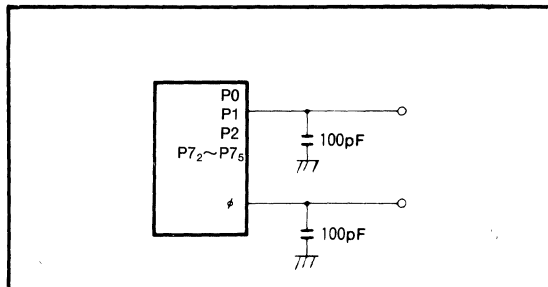
Fig.25 Port P0, P1, P2, P7 2 ~P7 5 test circuit
