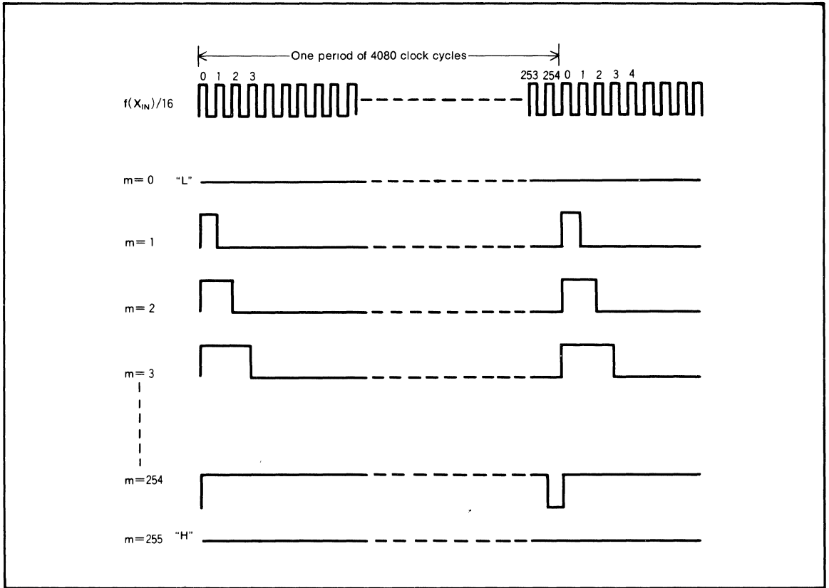
Fig.14 Relation between m and PWM output
