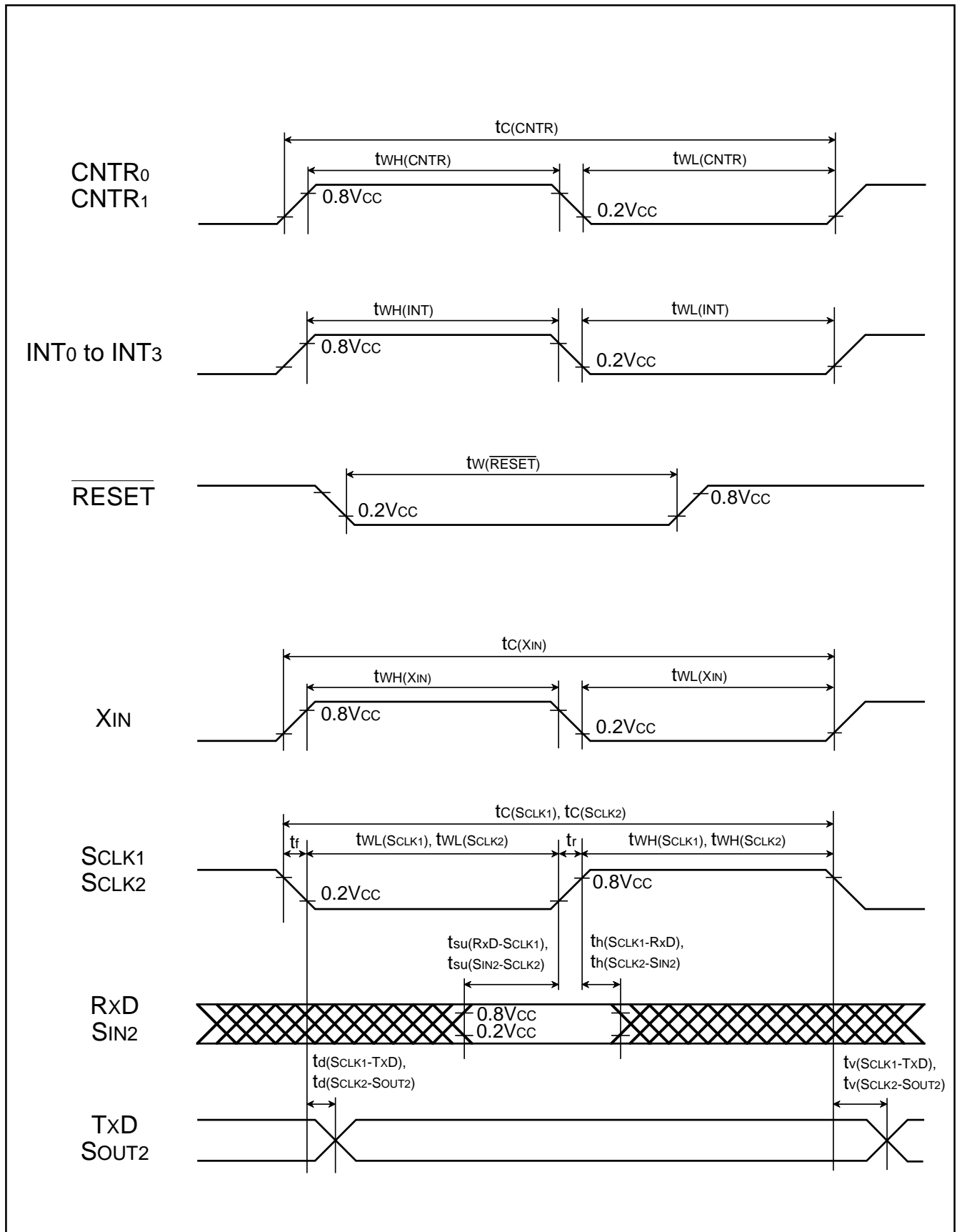
Fig. 81 Timing diagram
