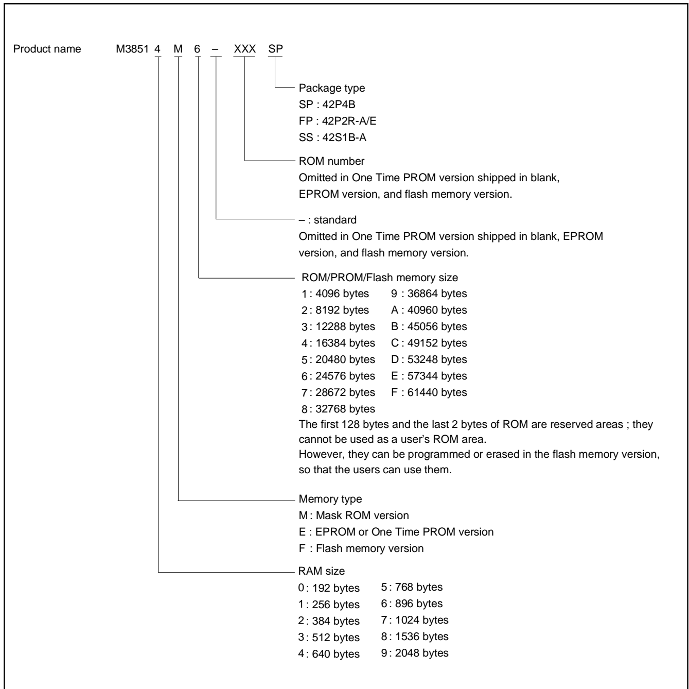
Fig. 3 Part numbering
