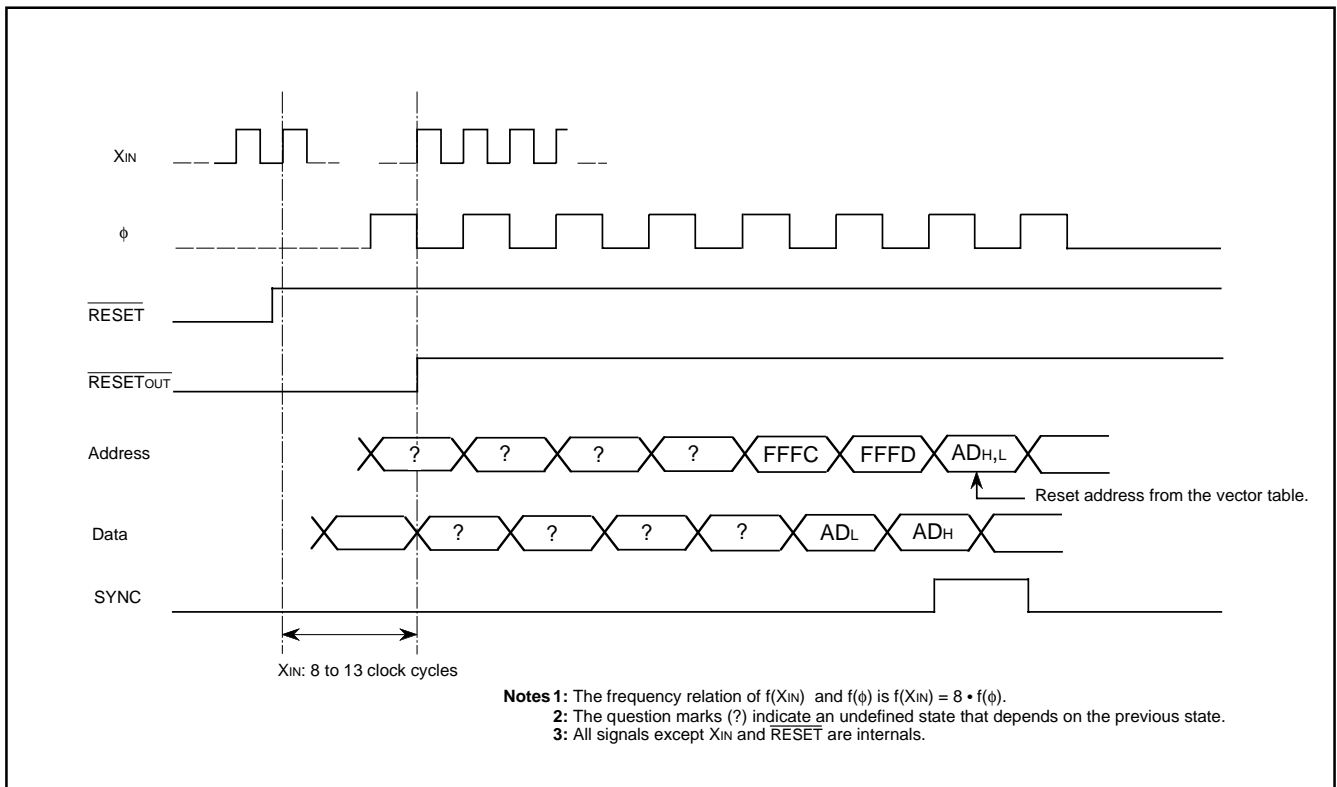
Fig. 50 Reset sequence
