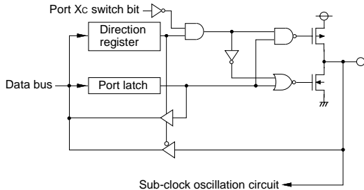
(7) Port P4 1
