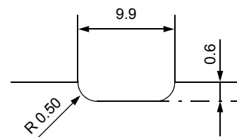
Detail C
