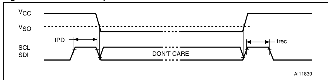
Figure 17. Power down/up mode AC waveforms
