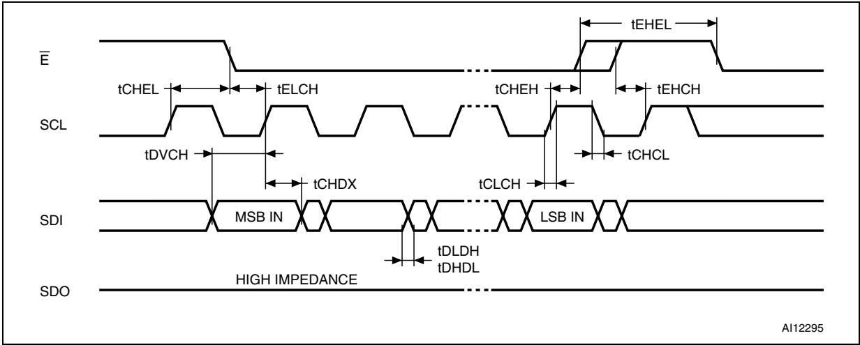
Figure 18. Input timing requirements
