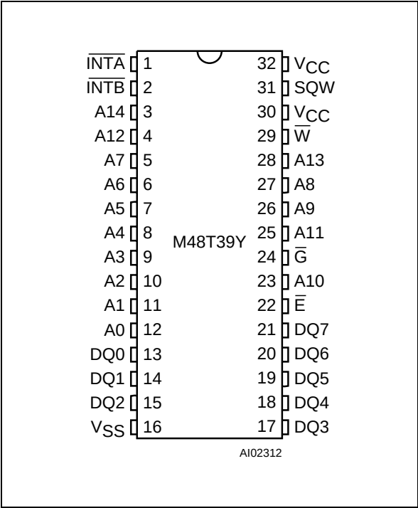
Figure 2. DIP Connections
