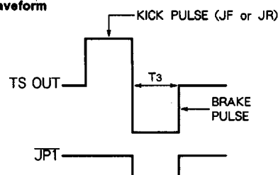
Jump T. ACT waveform
