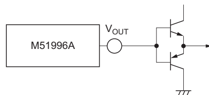
Figure 34 Output Buffer Circuit Diagram
