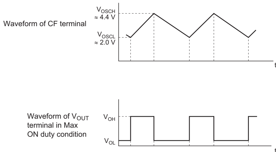
Figure 5 Oscillator Waveform When the SOFT Circuit is Operating
