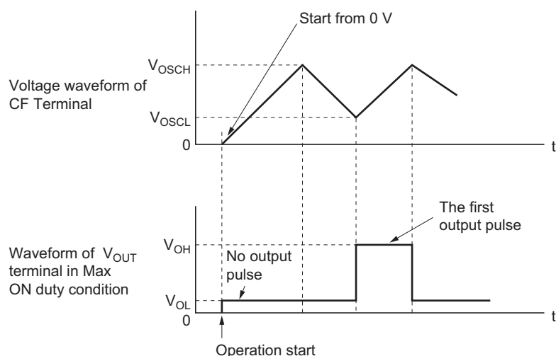
Figure 6 Relationship Between Oscillator Waveform and Output Waveform at Start-up
