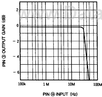
M52065P FREQUENCY CHARACTERISTICS
