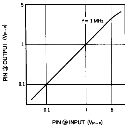
M52065P INPUT/OUTPUT CHARACTERISTICS
