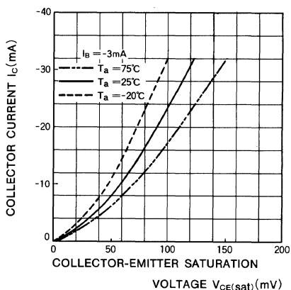
OUTPUT CHARACTERISTICS
