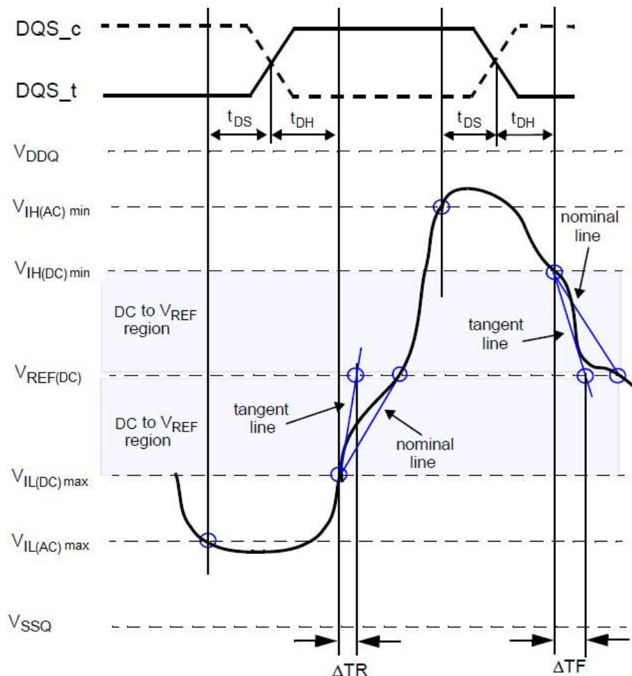
Figure 24. Illustration of tangent line for hold time t_{DH} for DQ with respect to strobe
