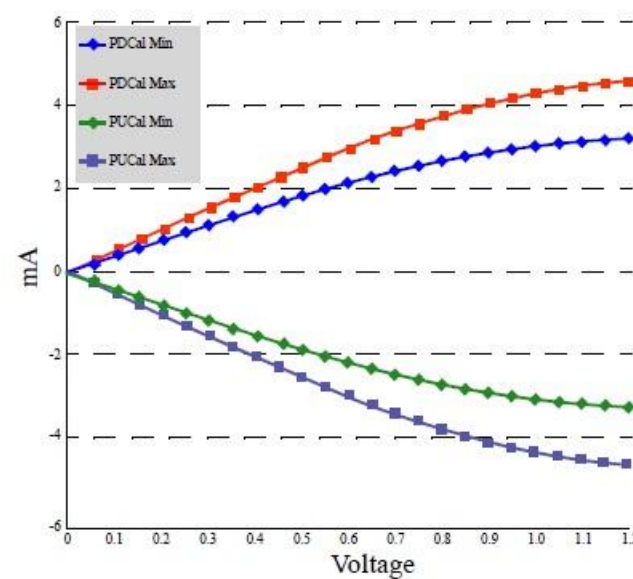
Figure 15. R_{ON} = 240\text{ Ohms} IV Curve after calibration
