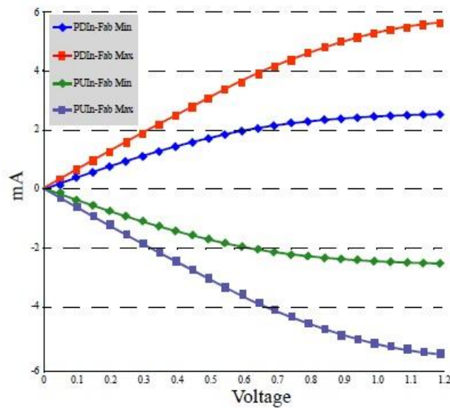
Figure 14. R_{ON} = 240\text{ Ohms} IV Curve after ZQReset
