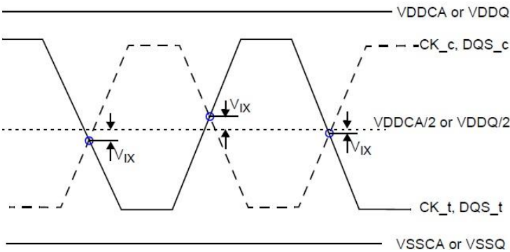
Figure 7. V_{IX} Definition
