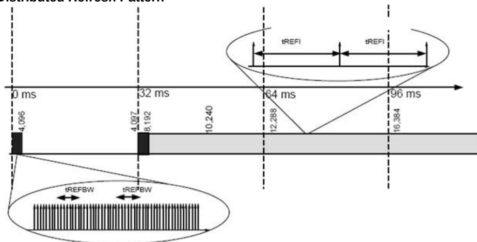
Figure 55. Allowable Transition from Repetitive Burst Refresh with Subsequent Refresh Pause to Regular, Distributed Refresh Pattern
