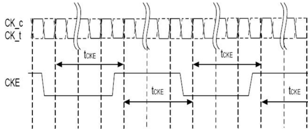
Figure 72. CKE Intensive Environment
