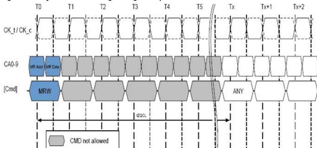
Figure 69. ZQ Calibration Long timing example
