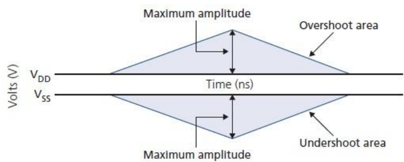
Figure 11. Overshoot/Undershoot Definition
