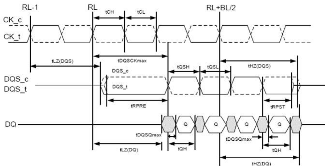
Figure 30. Data output (read) timing ( t_{DQ\text{SCK}_{\text{max}}} )
