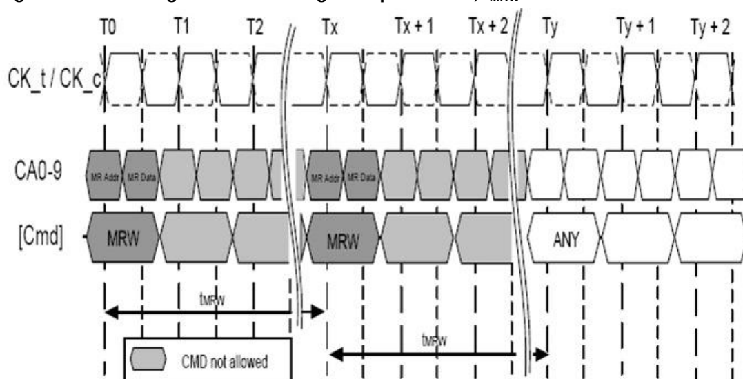
Figure 66. Mode Register Write timing example: RL = 3, t_{MRW} = 5
