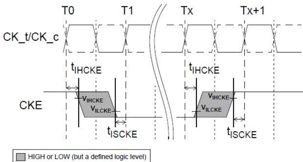
Figure 29. CKE Input Setup and Hold Timing
