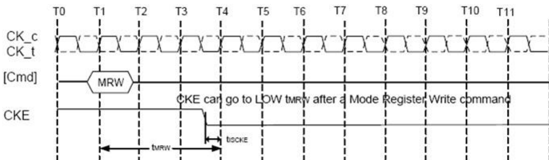
Figure 82. Mode Register Write to Power Down Entry
