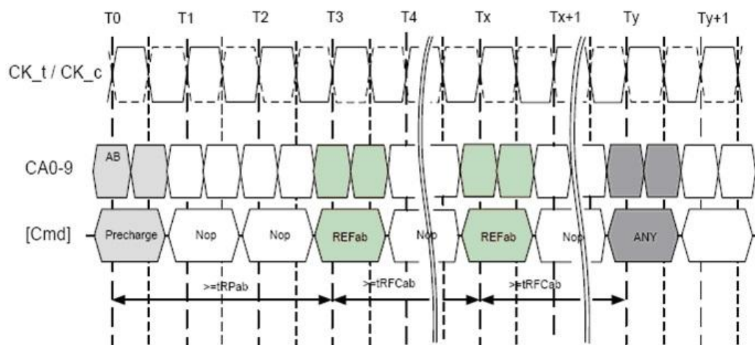
Figure 58. All Bank Refresh Operation
