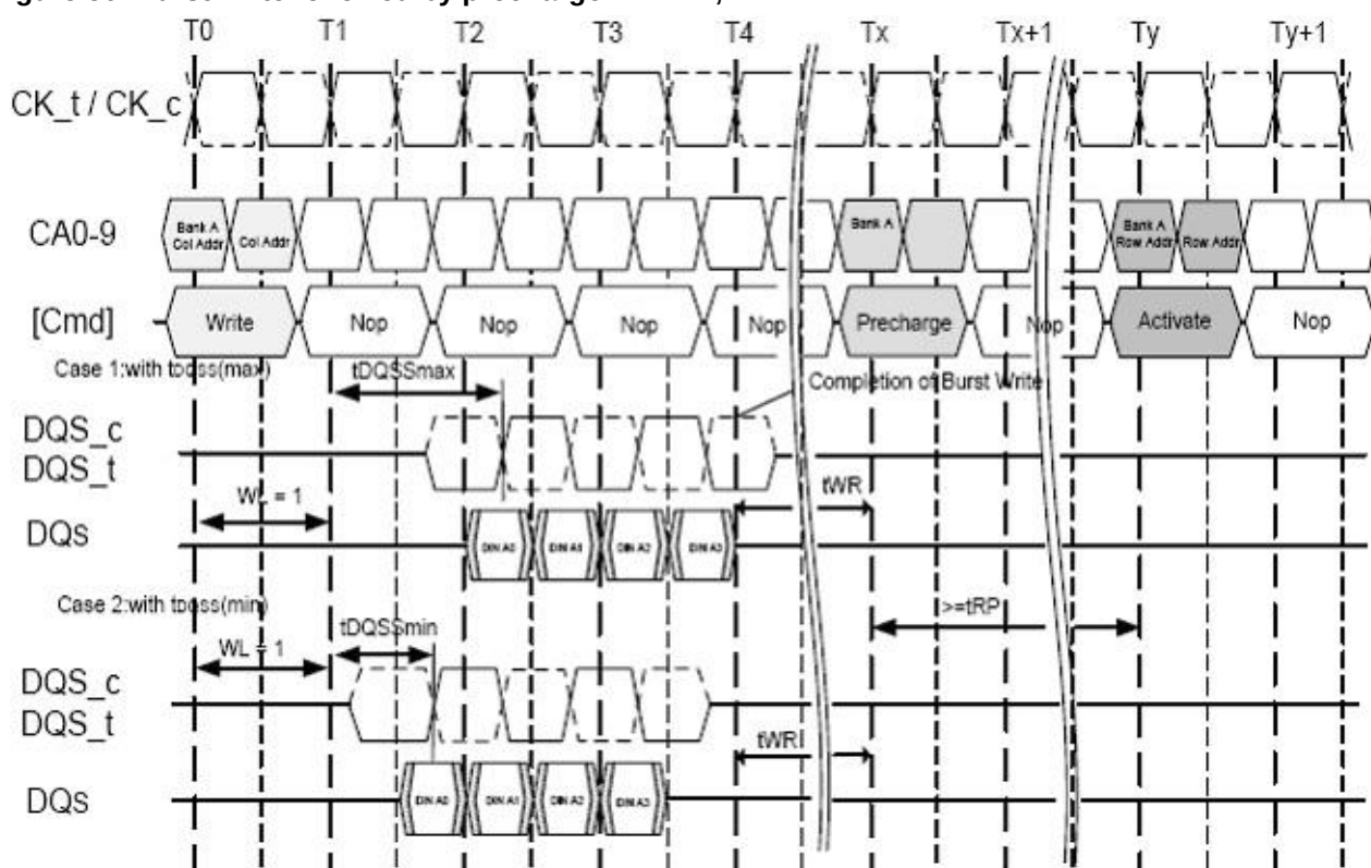
Figure 50. Burst write followed by precharge: WL = 1, BL = 4
