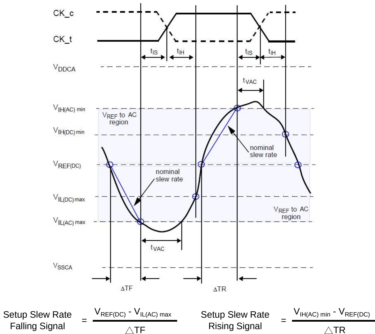
Figure 17. Illustration of nominal slew rate and t_{VAC} for setup time t_{IS} for CA and CS_n with respect to clock
