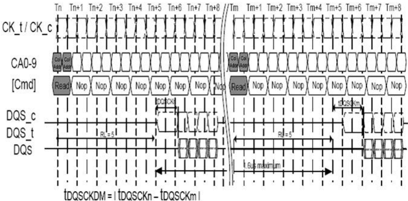
Figure 35. t_{DQSKDM} timing
