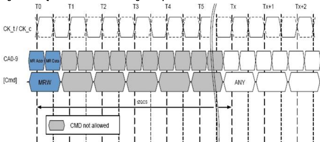
Figure 68. ZQ Calibration Short timing example
