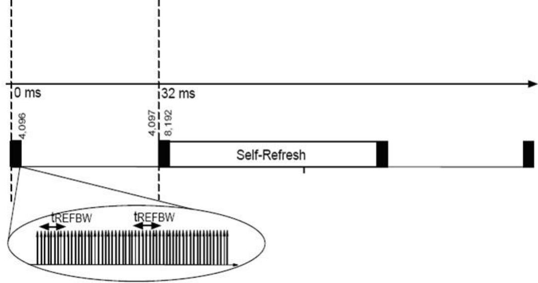
Figure 57. Recommended Self Refresh entry and exit in conjunction with a Burst/Pause Refresh patterns
