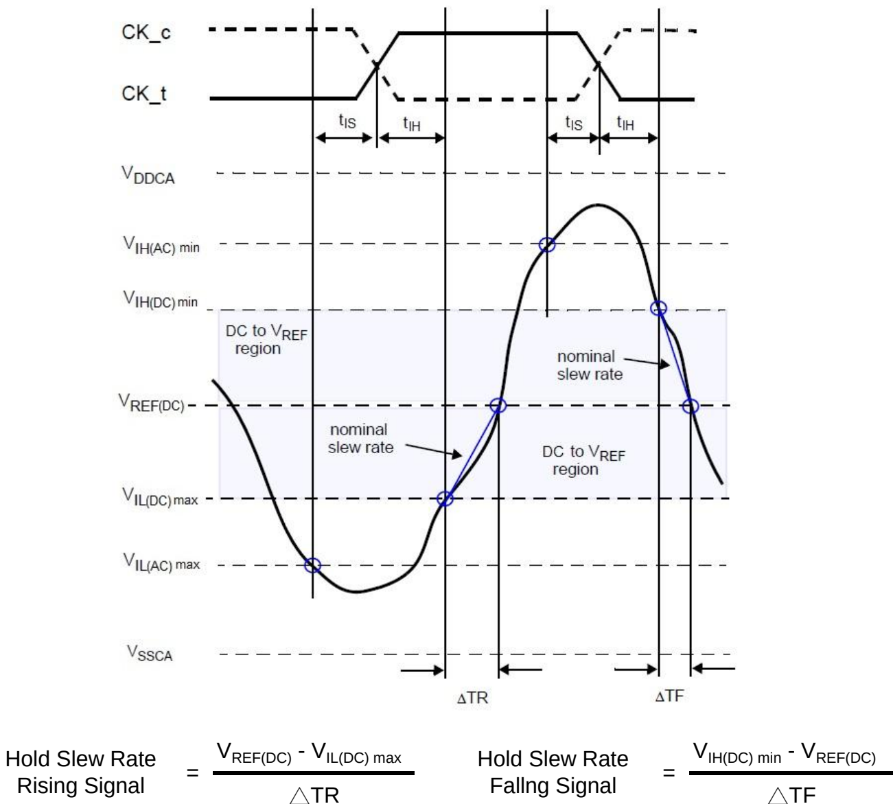
Figure 18. Illustration of nominal slew rate for hold time t_{IH} for CA and CS_n with respect to clock
