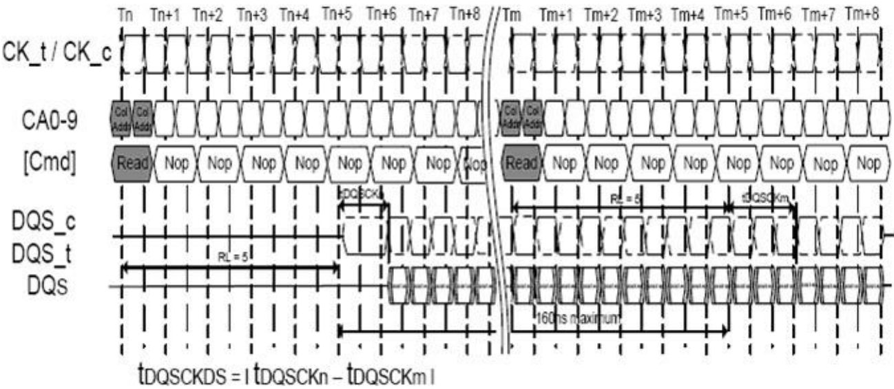
Figure 36. t_{DQSKDS} timing
