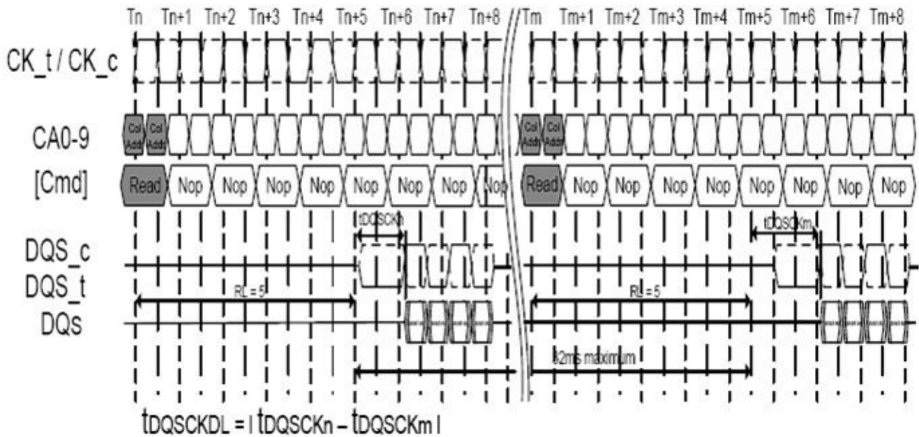
Figure 34. t_{DQSKDL} timing
