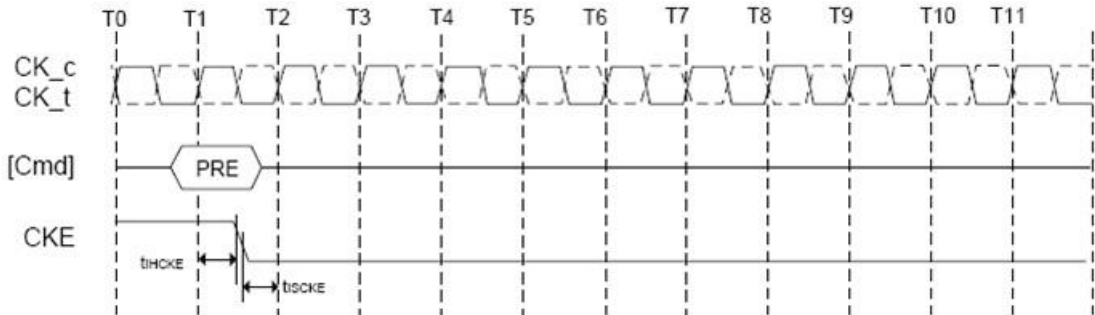
Figure 80. Precharge/Precharge All command to Power Down Entry
