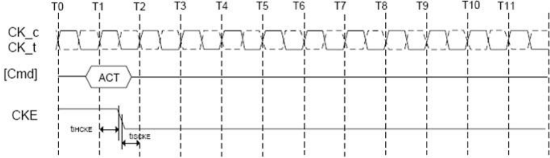
Figure 79. Activate command to Power Down Entry
