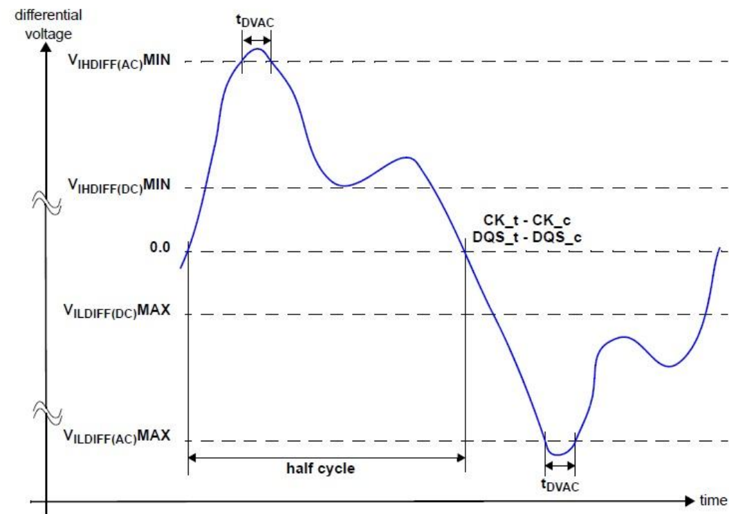
Figure 5. Differential AC swing time and t_{DVAC}
