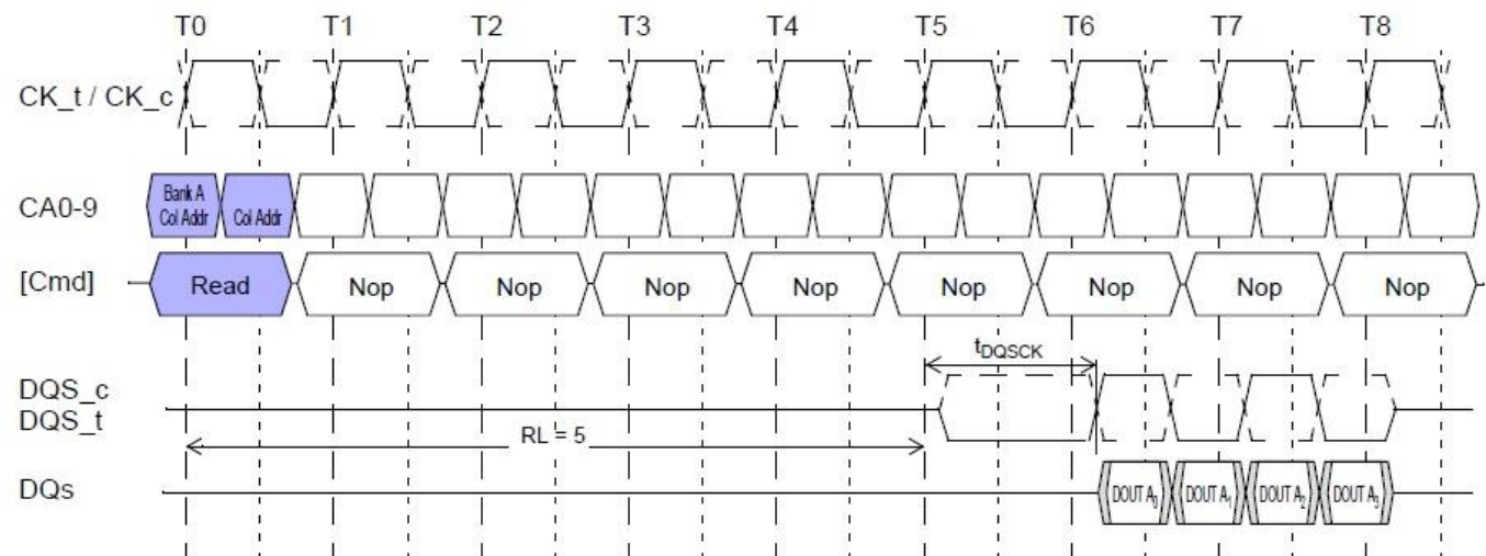
Figure of Burst read: RL = 5, BL = 4, t_{DQSK} > t_{CK}
