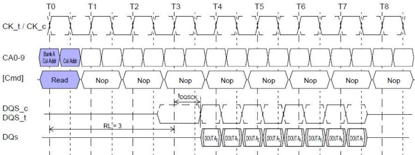
Figure of Burst read: RL = 3, BL = 8, t_{DQSK} < t_{CK}
