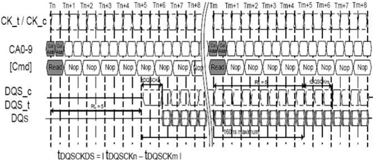
Figure of t_{DQSCKDS} timing
