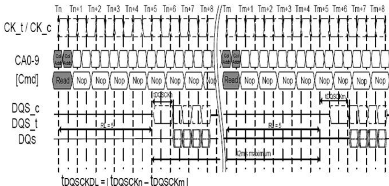
Figure of t_{DQSKDL} timing
