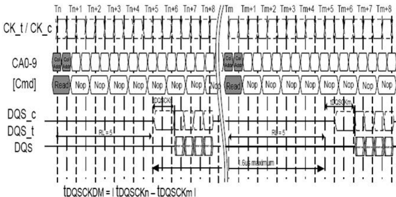
Figure of t_{DQSKDM} timing
