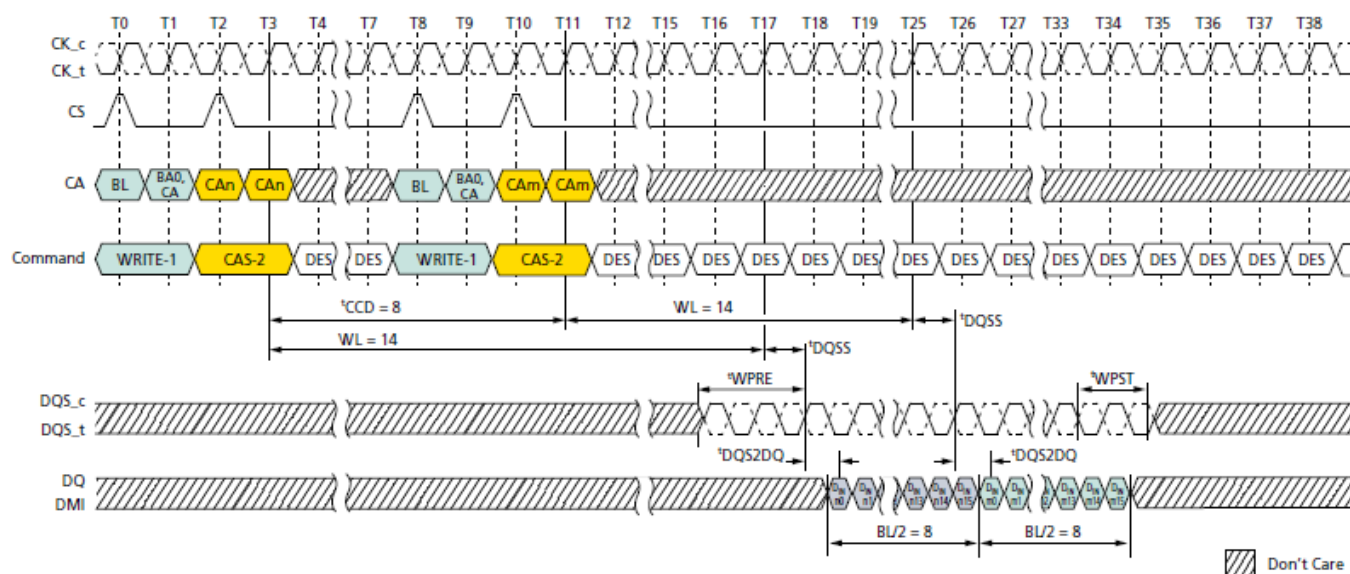
Figure 49. Seamless WRITE: t_{CCD} = \text{MIN} , 1.5nCK Postamble
