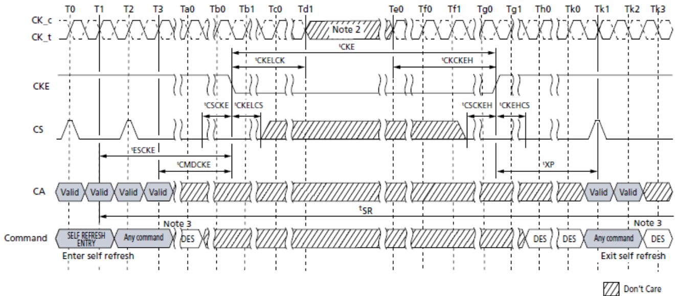
Figure 73. Command Input Timings after Power-Down Exit During Self Refresh
