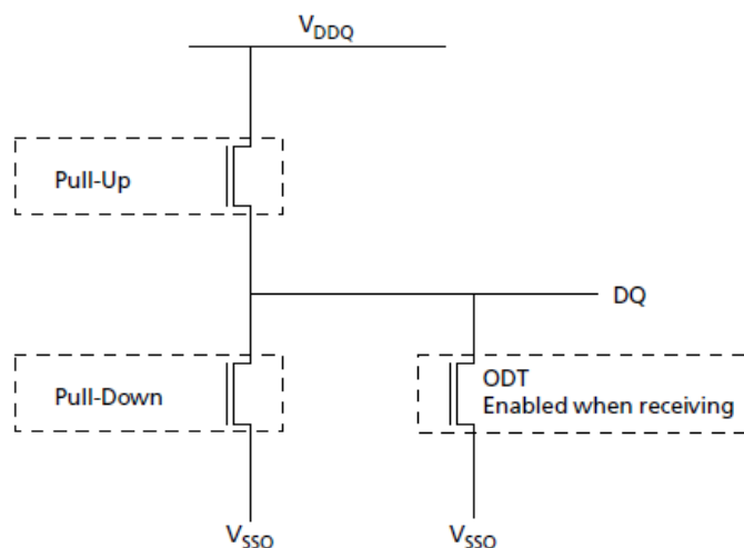
Figure 158. LVSTL I/O Cell
