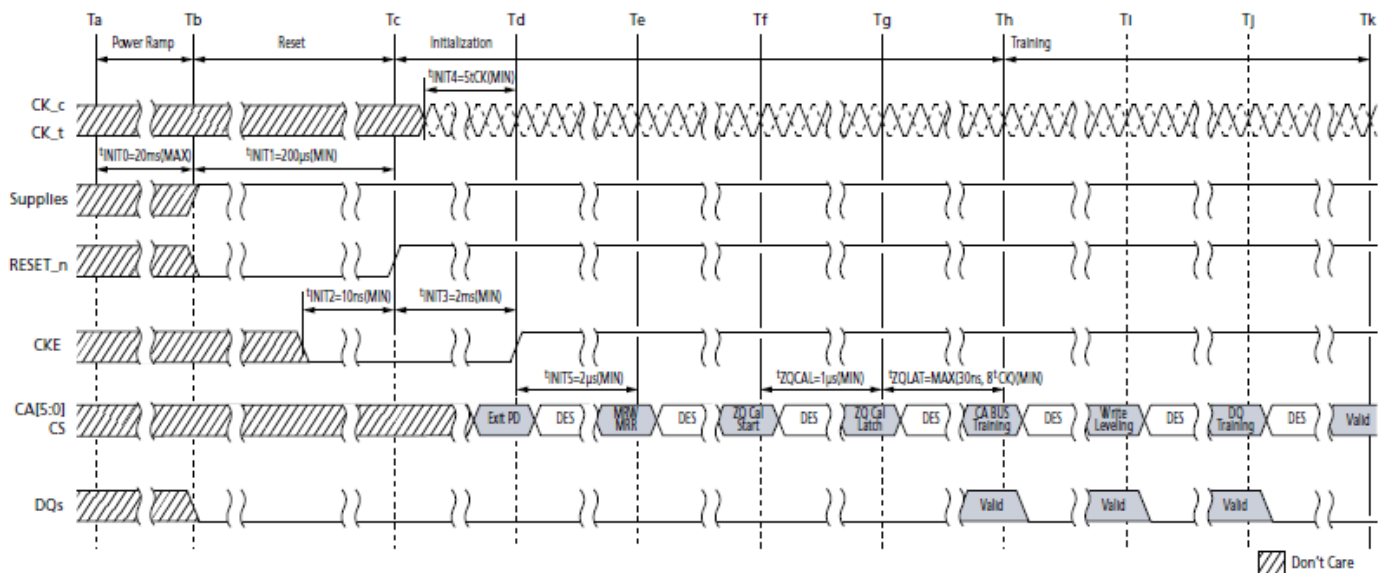
Figure 6. Voltage Ramp and Initialization Sequence
