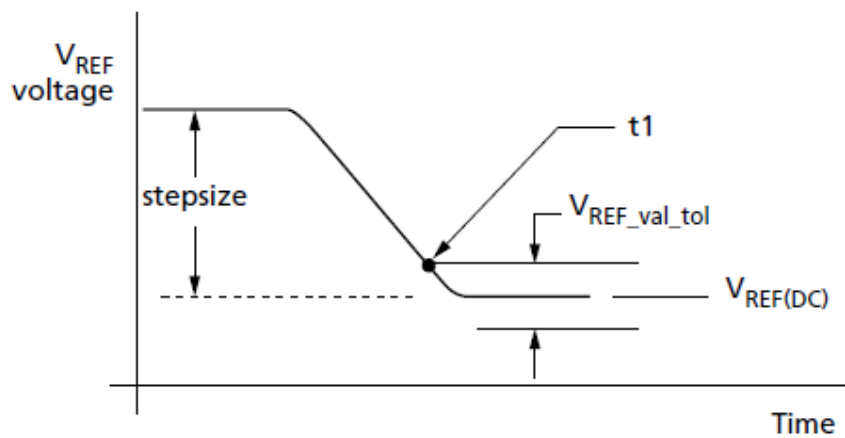
Figure 104. V_{REF(DQ)} Single-Step Size Decrement
