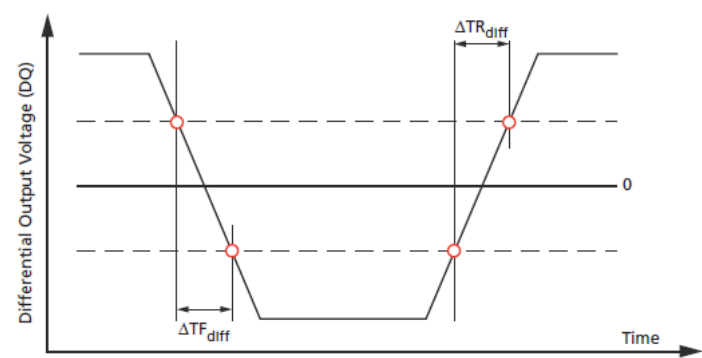
Figure 180. Differential Output Slew Rate Definition
