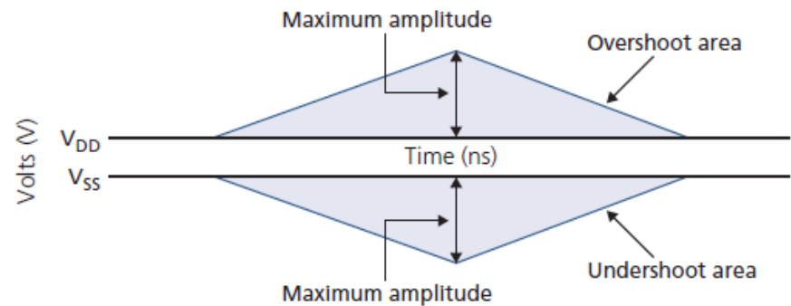
Figure 156. Overshoot and Undershoot Definition
