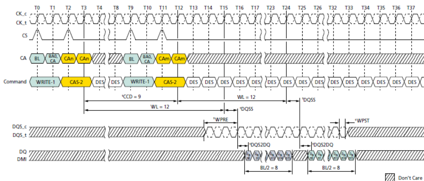
Figure 50. Consecutive WRITE: t_{CCD} = \text{MIN} + 1 , 0.5nCK Postamble
