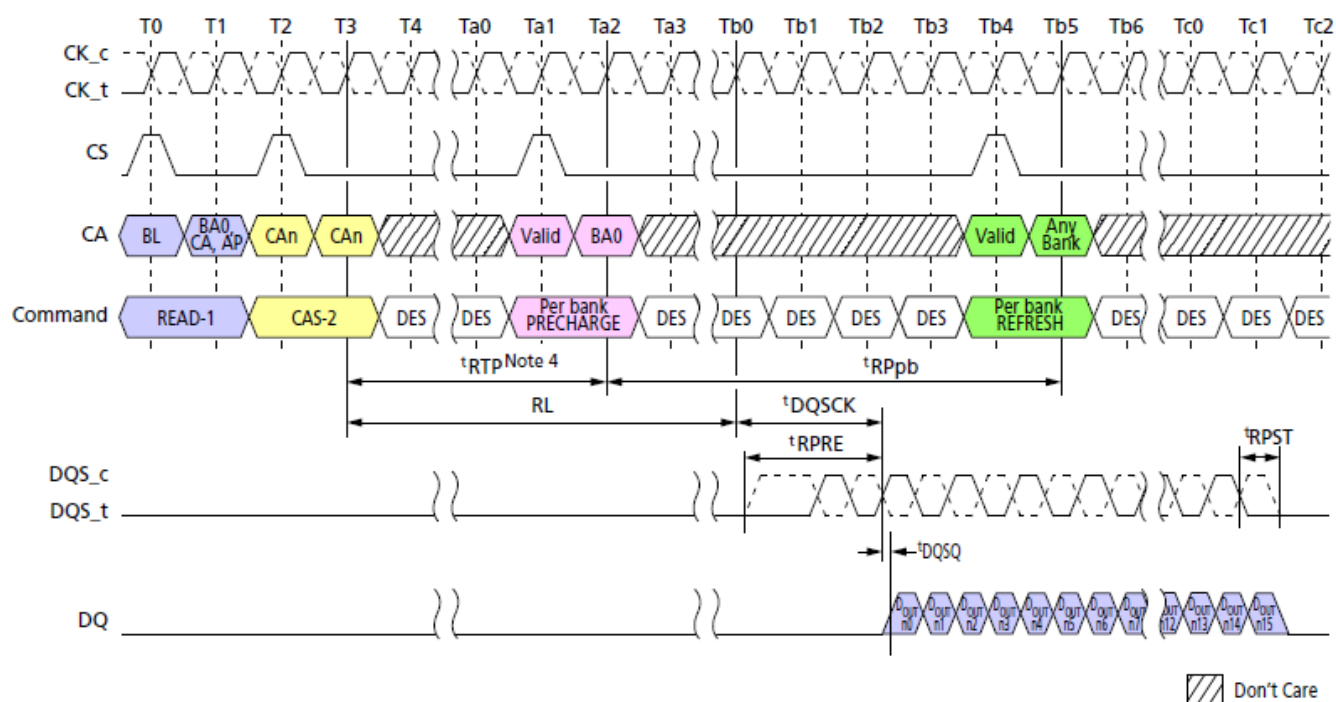
Figure 69. Burst READ Operation Followed by Per Bank Refresh
