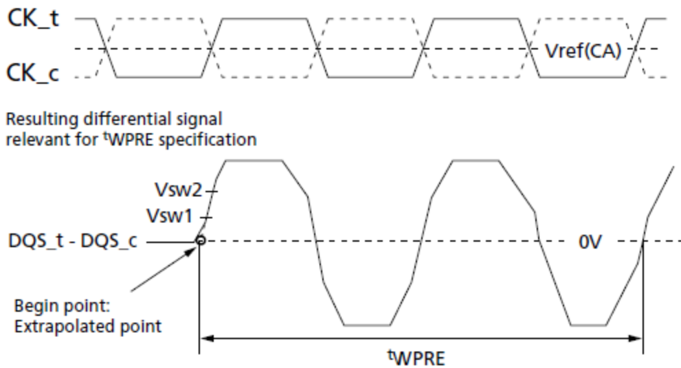
Figure 24. Method for Calculating tWPRE Transitions and Endpoints
