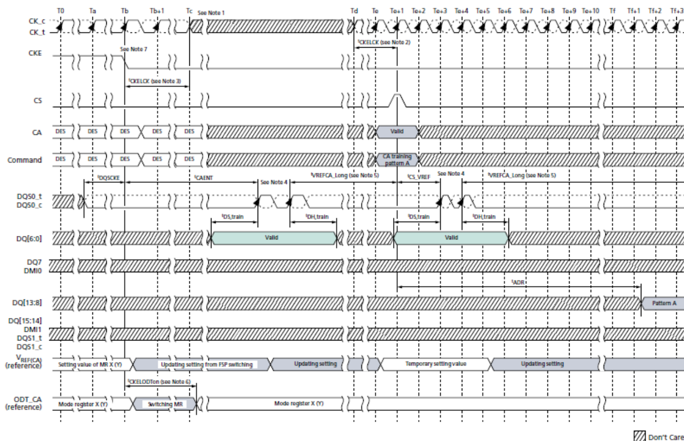
Figure 108. Consecutive V_{REF(CA)} Value Update
