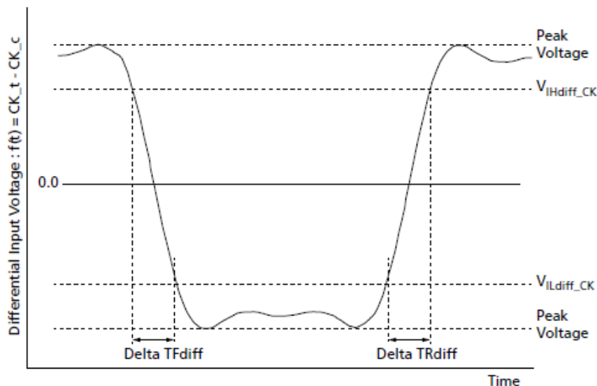
Figure 147. Differential Input Slew Rate Definition for CK_t, CK_c
