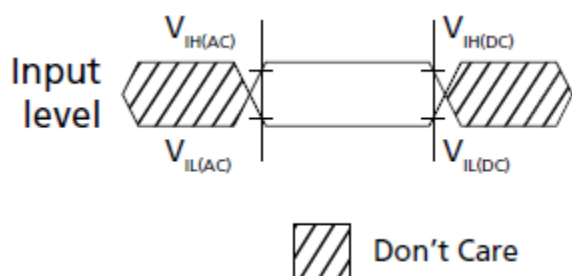
Figure 142. Input Timing Definition for CKE
