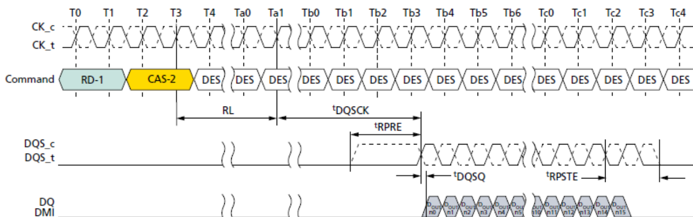
Figure 10. DQS Read Preamble and Postamble – Static Preamble and 1.5nCK Postamble
