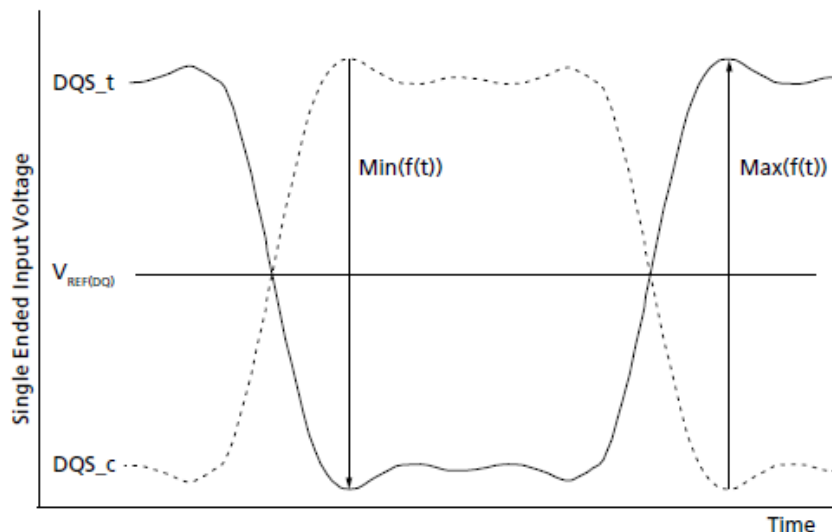
Figure 150. Definition of Differential DQS Peak Voltage
