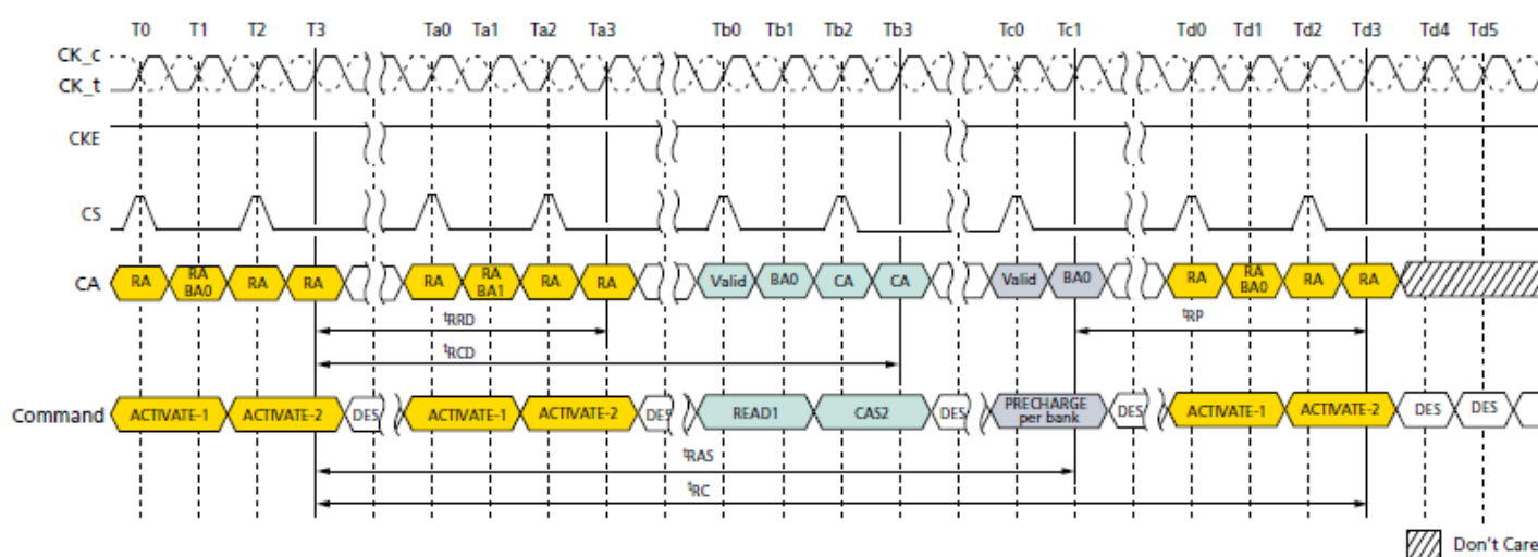
Figure 7. ACTIVATE Command
