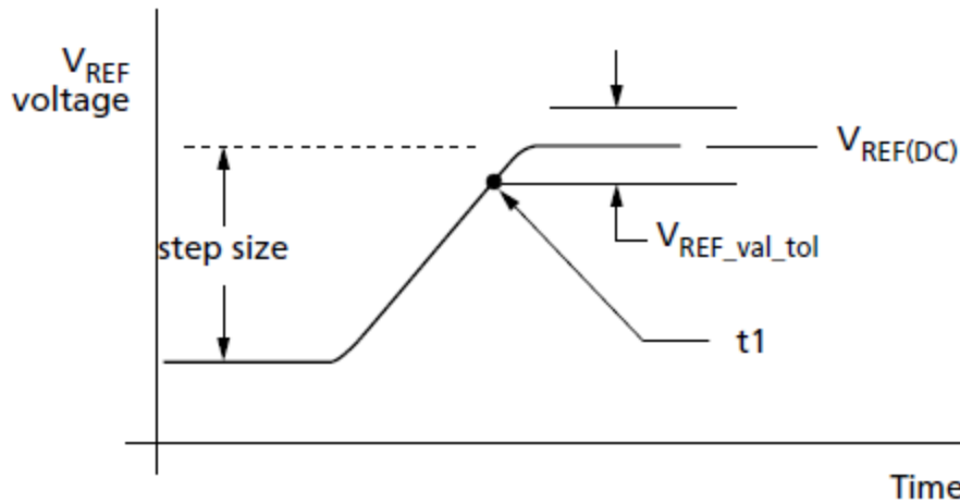
Figure 96. V_{REF(CA)} Single-Step Increment
