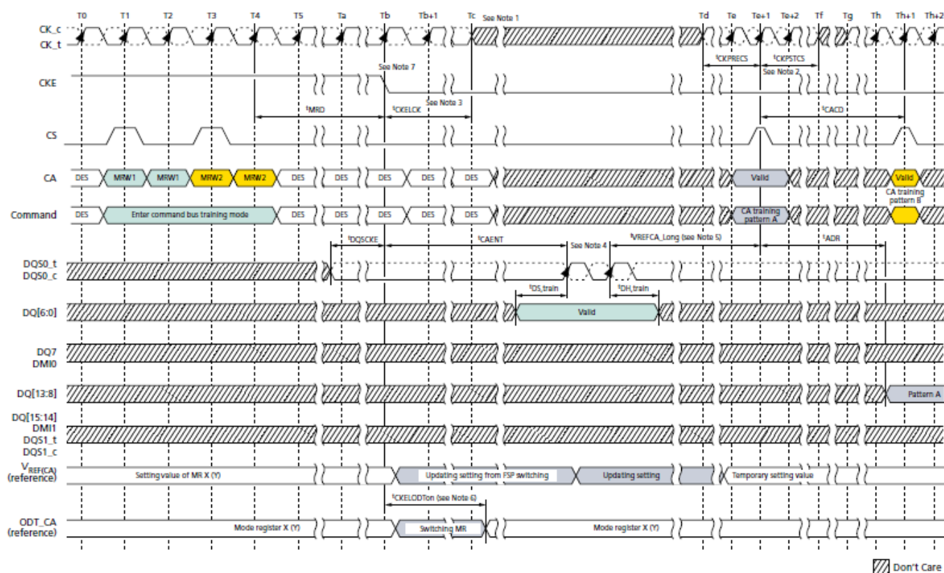
Figure 107. Command Bus Training Mode Entry – CA Training Pattern I/O with V_{REF(CA)} Value Update
