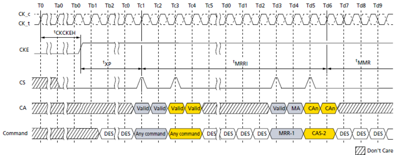
Figure 89. MRR Following Power-Down
