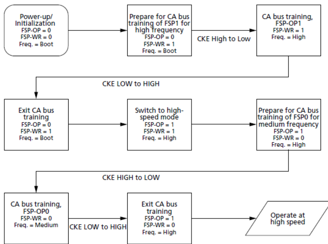
Figure 132. Training for Two Frequency Set Points
