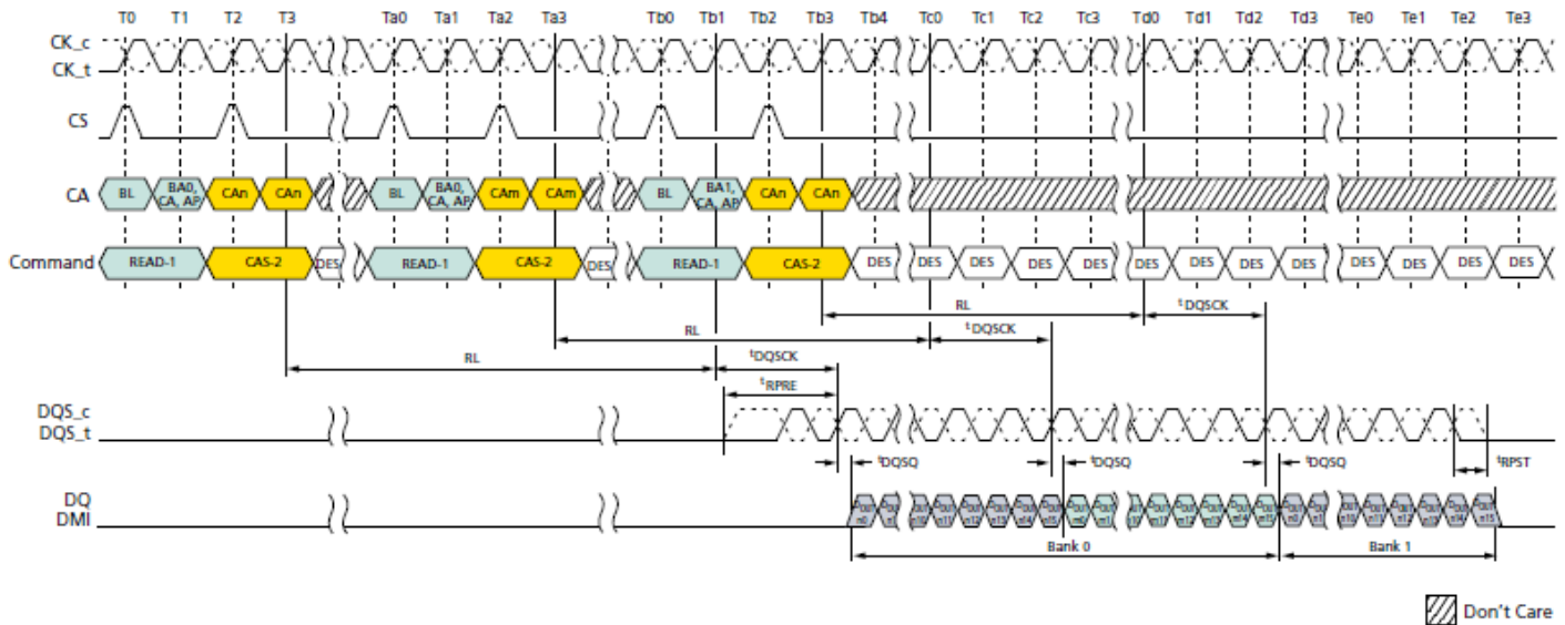
Figure 15. Seamless Burst Read
