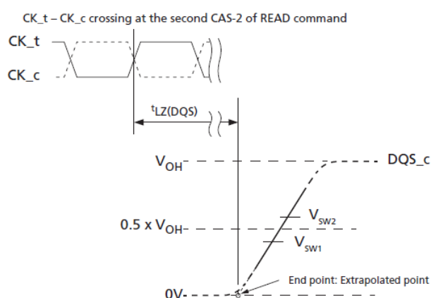
Figure 173. t_{LZ}(DQS) Method for Calculating Transitions and Endpoint
