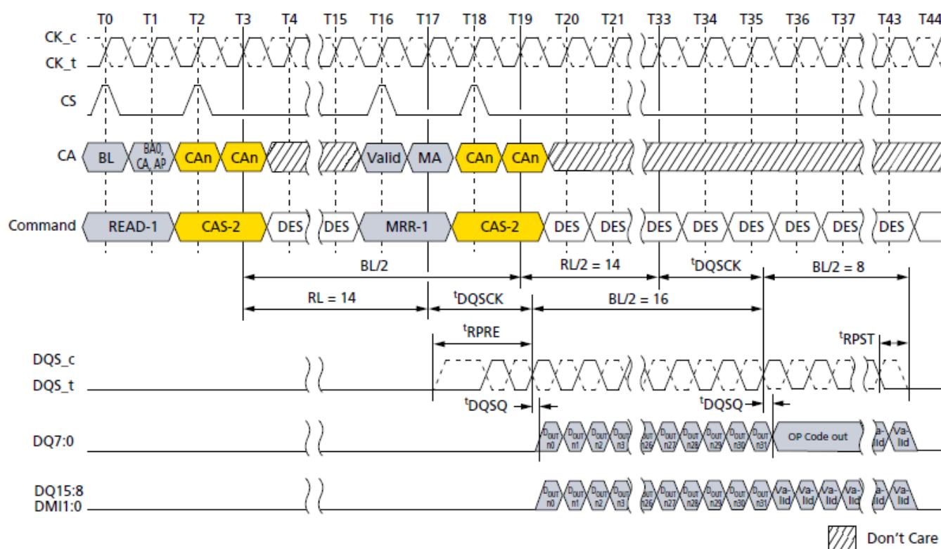
Figure 87. READ-to-MRR Timing
