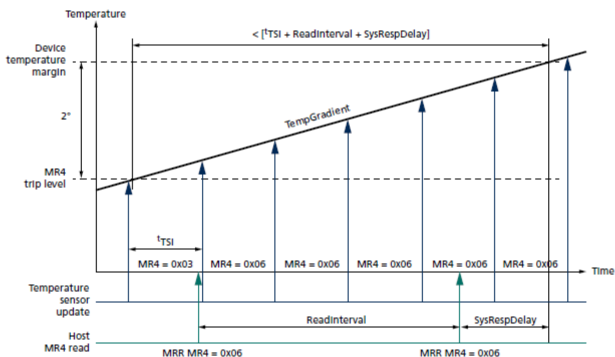
Figure 129. Temperature Sensor Timing
