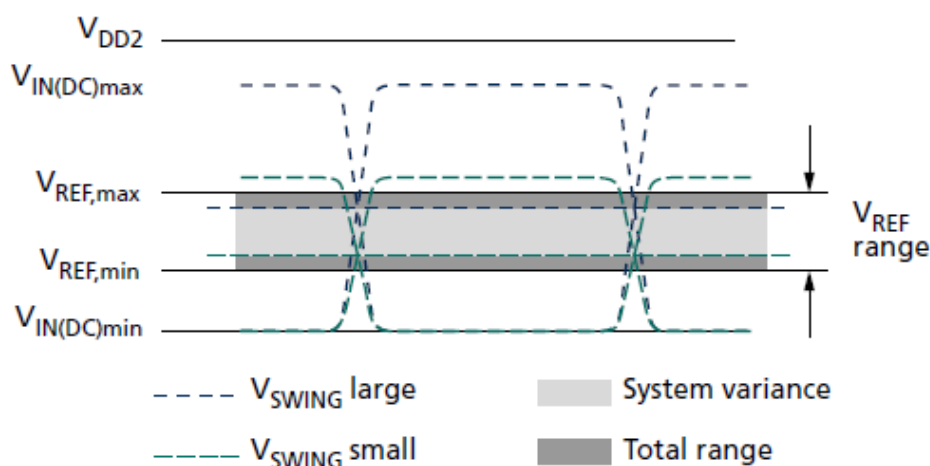
Figure 93. V REF Operating Range (V REF,max , V REF,min )
