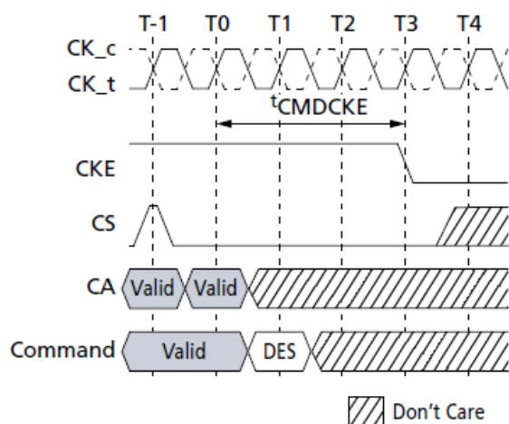
Figure 160. t_{CMDCKE} Timing
