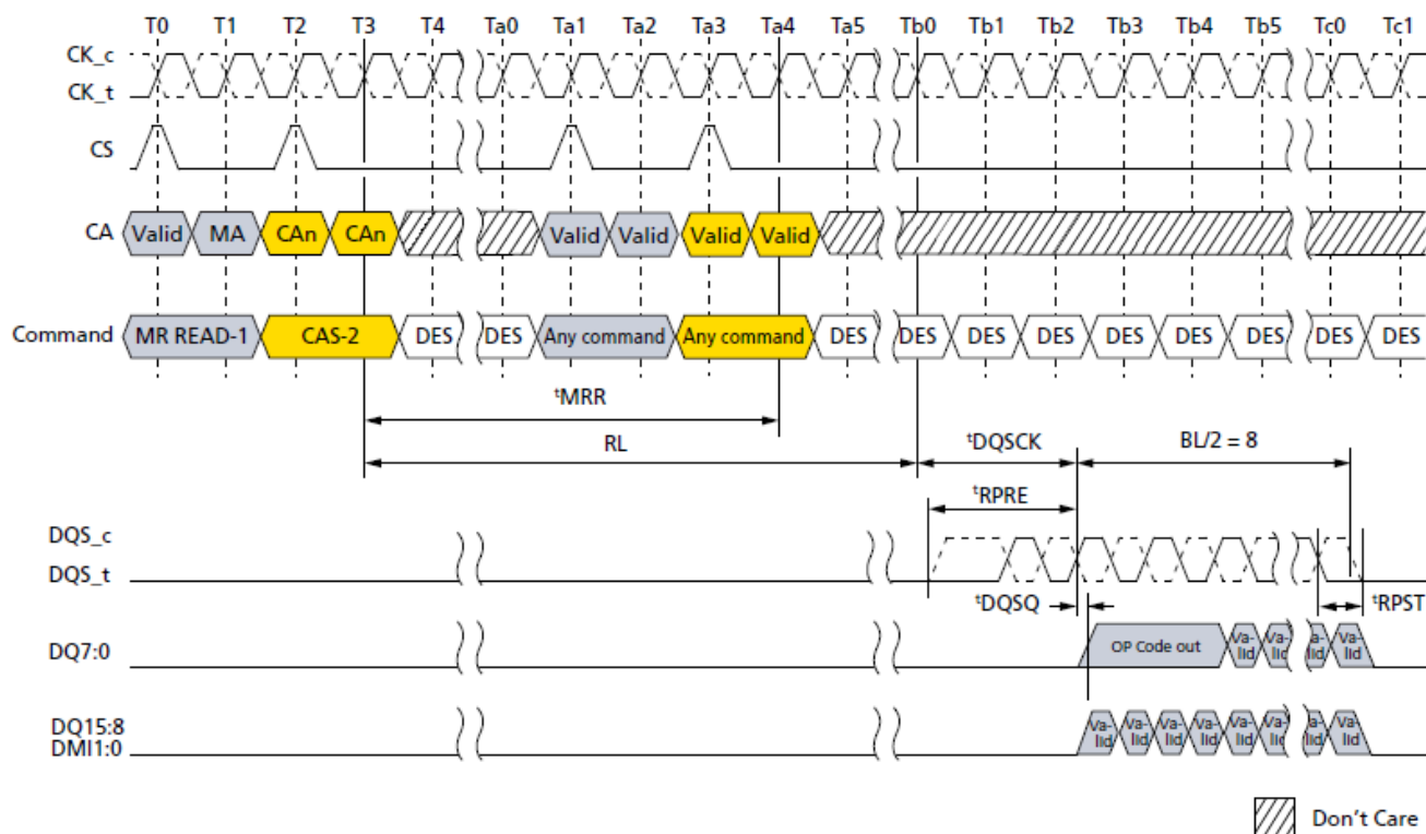
Figure 86. MODE REGISTER READ Operation
