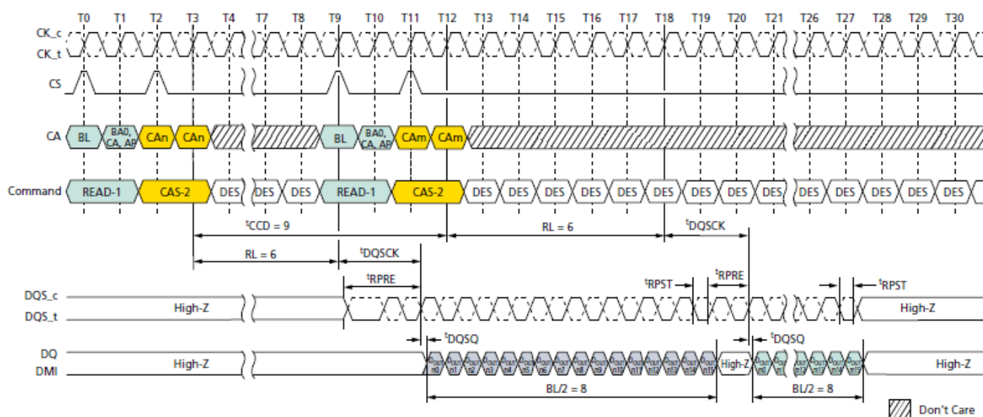
Figure 36. Consecutive READ: t_{CCD} = MIN + 1 , Preamble = Toggle, 0.5nCK Postamble
