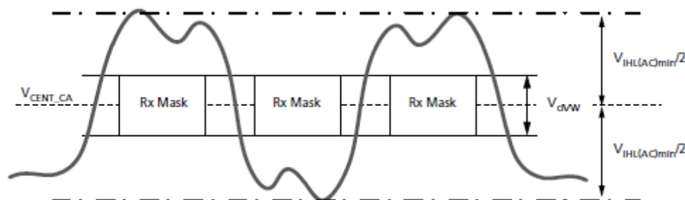
Figure 166. CA V_{IHL\_AC} Definition (for Each Input Pulse)
