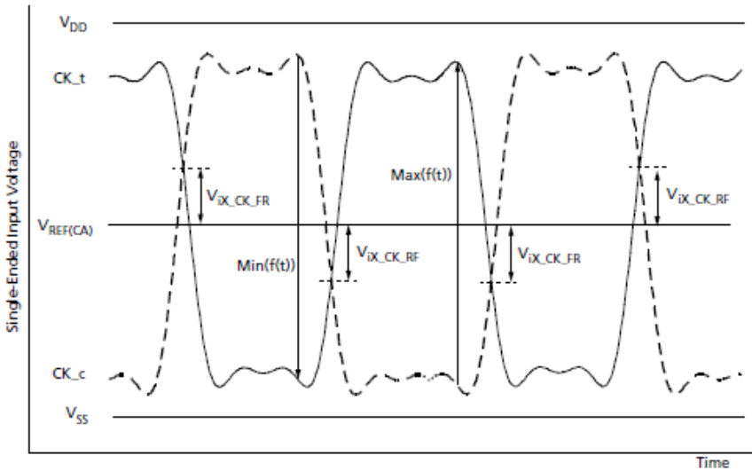
Figure 148. V_{ix} Definition (Clock)
