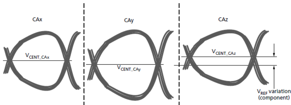
Figure 163. Across Pin V_{REF(CA)} Voltage Variation
