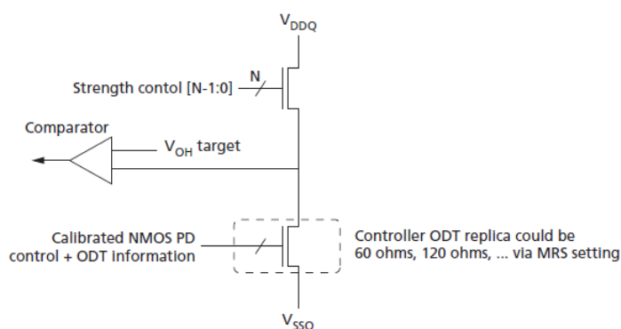
Figure 182. Pull-Up Calibration
