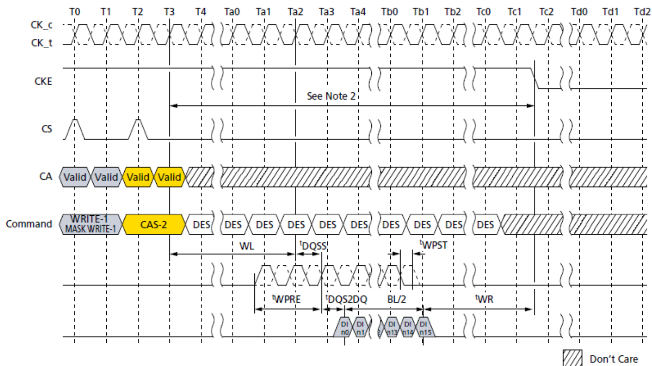
Figure 78. Write and Mask Write to Power-Down Entry
