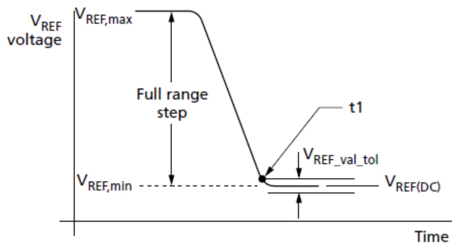
Figure 99. V_{REF(CA)} Full Step from V_{REF,max} to V_{REF,min}
