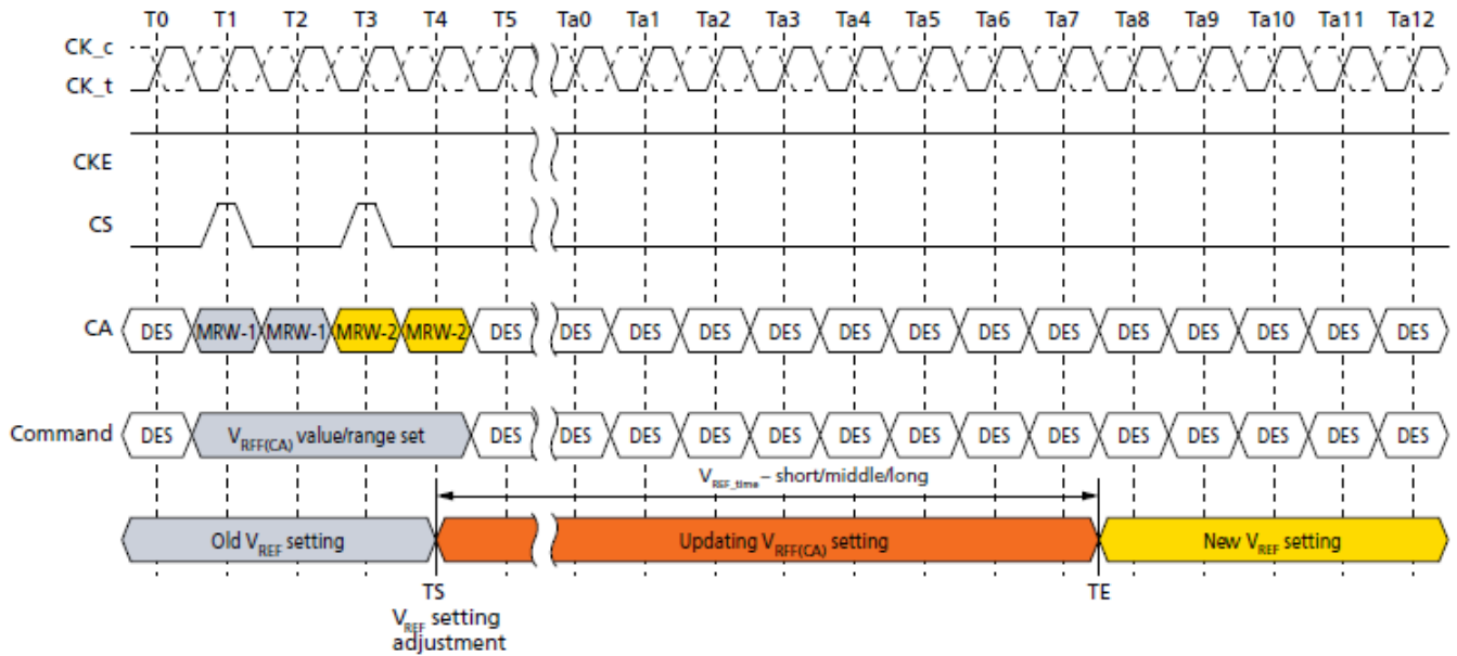
Figure 95. t_{V_{ref}} for Short, Middle, and Long Timing Diagram
