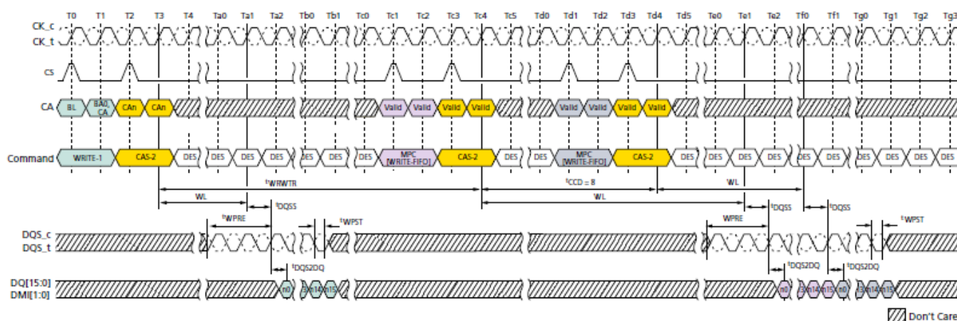
Figure 115. WRITE-FIFO – t_{WPRE} = 2nCK , t_{WPST} = 0.5nCK
