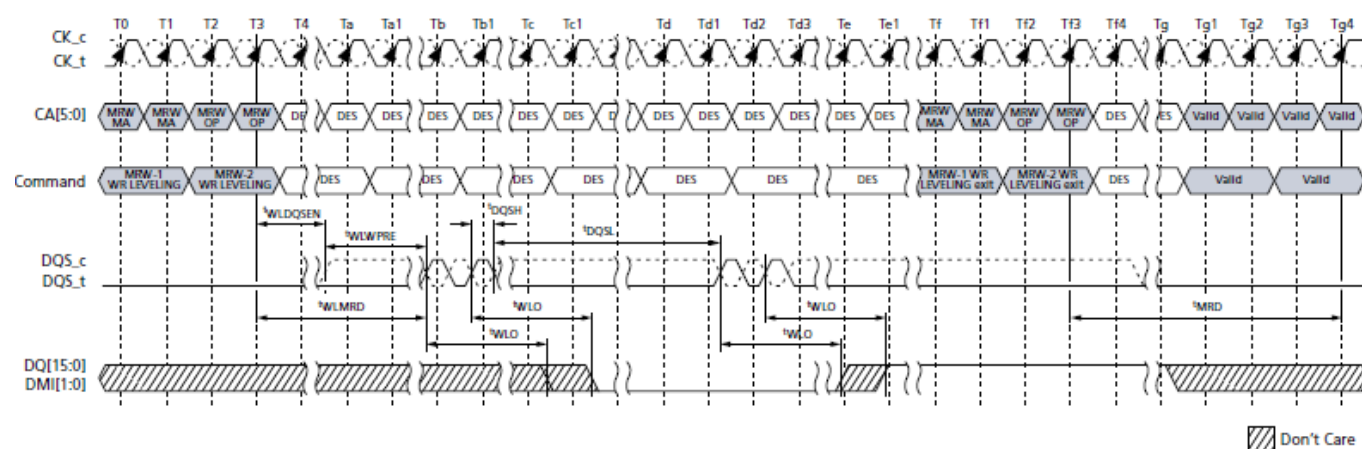
Figure 111. Write Leveling Timing – t_{DQSL}(\text{MAX})
