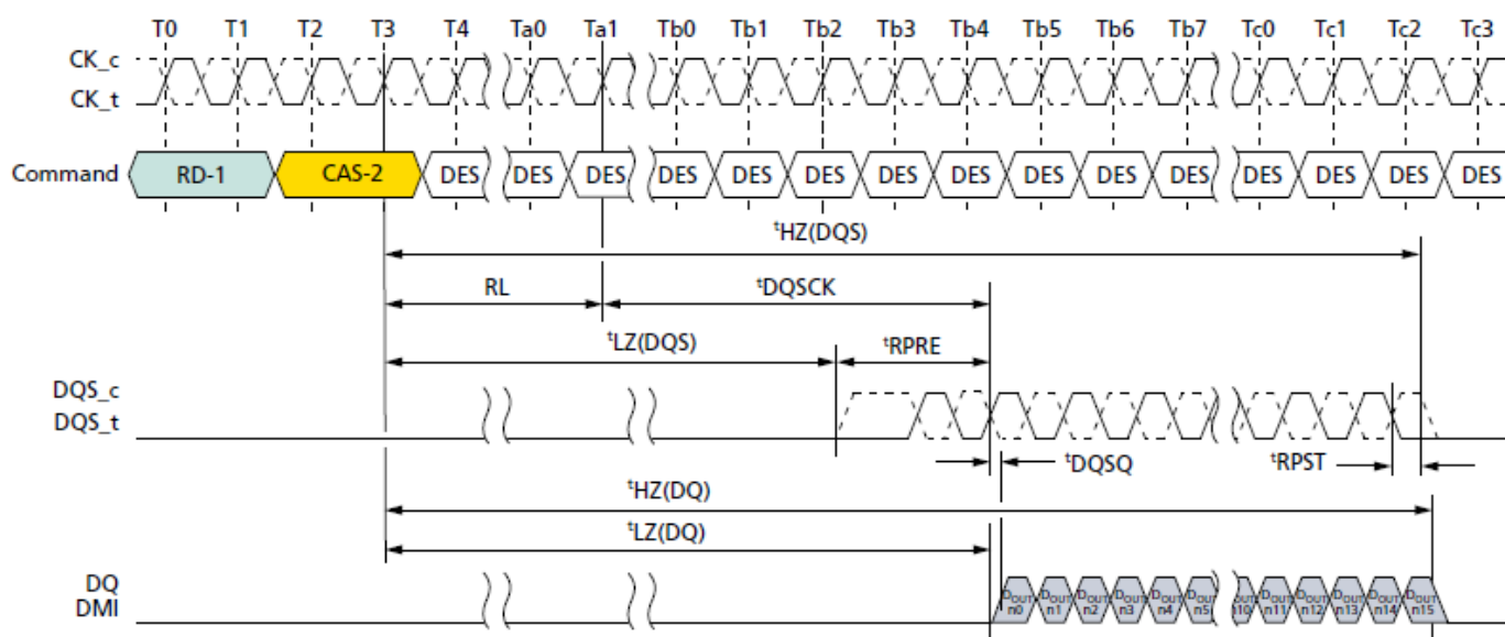
Figure 16. Read Timing
