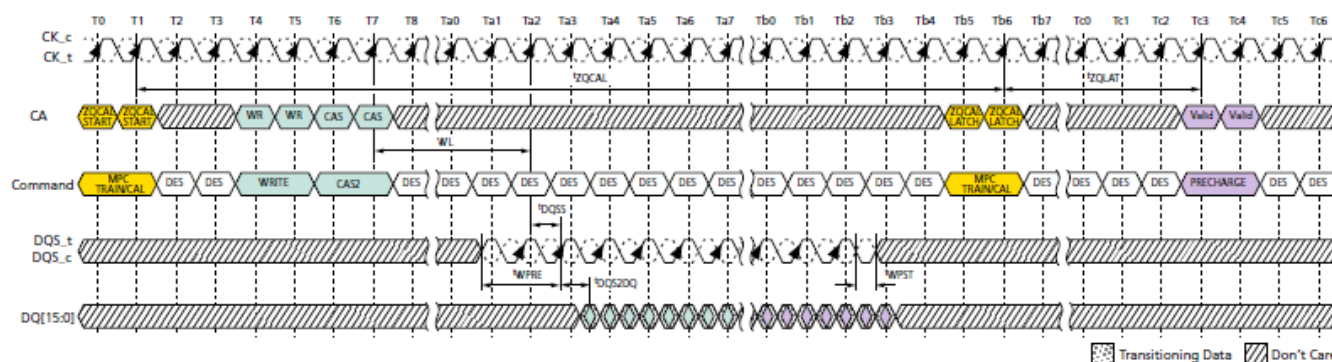
Figure 130. ZQCAL Timing
