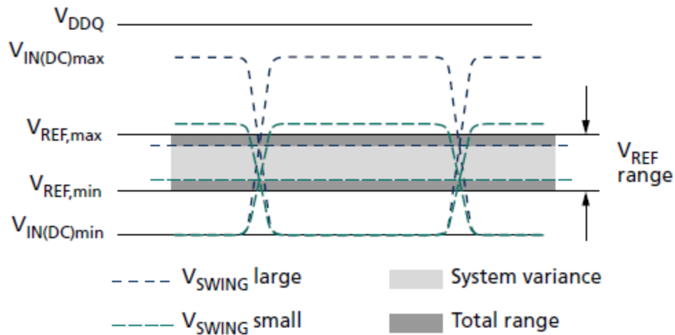
Figure 100. V_{REF} Operating Range ( V_{REF,max} , V_{REF,min} )
