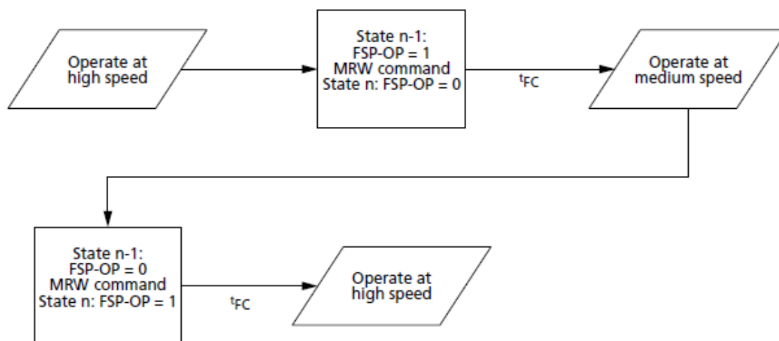
Figure 133. Example of Switching Between Two Trained Frequency Set Points
