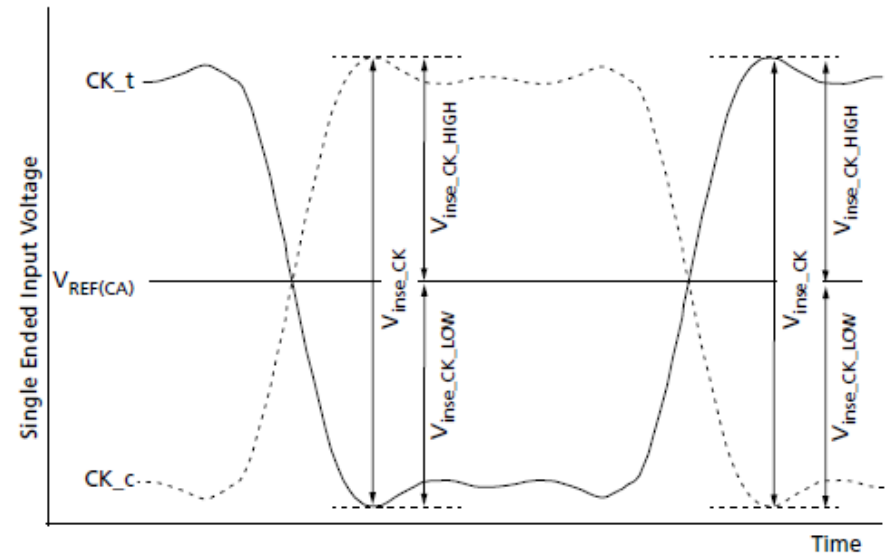
Figure 146. Clock Single-Ended Input Voltage
