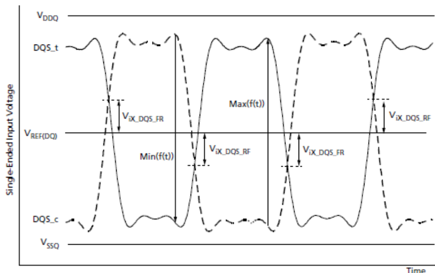
Figure 153. V_{ix} Definition (DQS)
