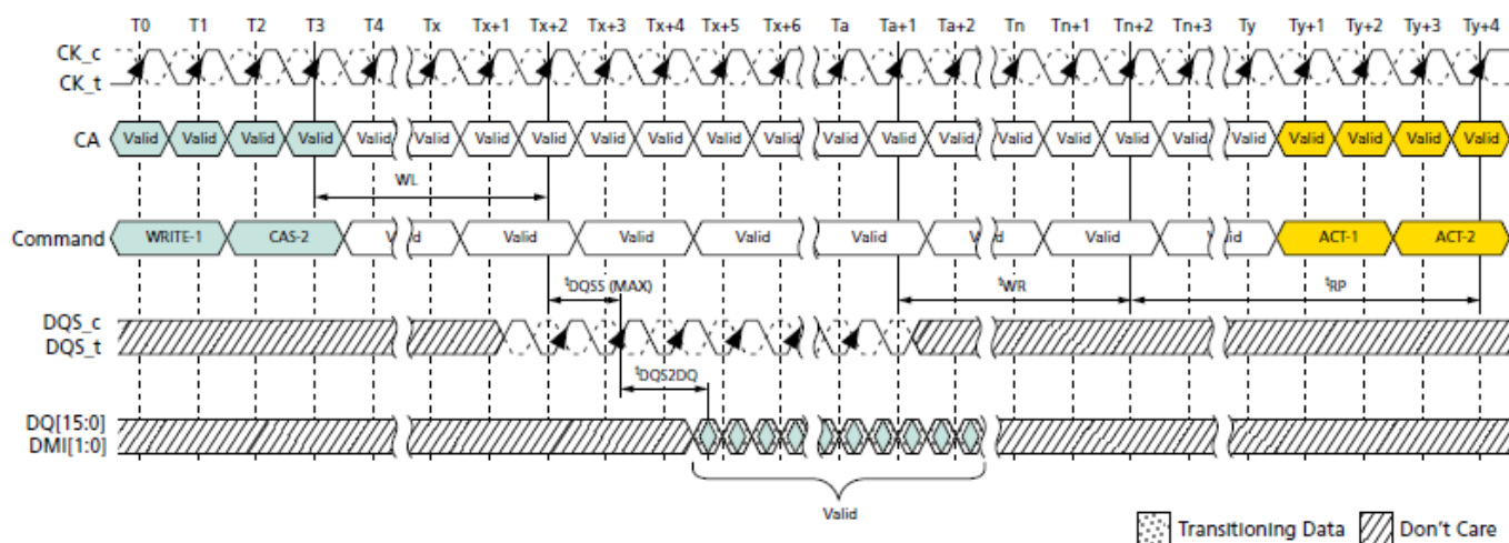
Figure 62. Burst WRITE With Auto Precharge – BL16, 2nCK Preamble, 0.5nCK Postamble
