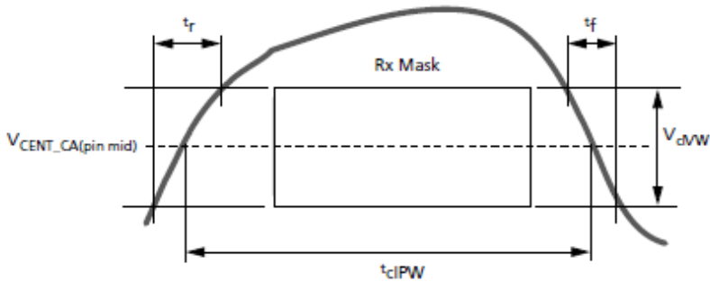
Figure 165. t_{cIPW} and SRIN_cIVW Definition (for Each Input Pulse)
