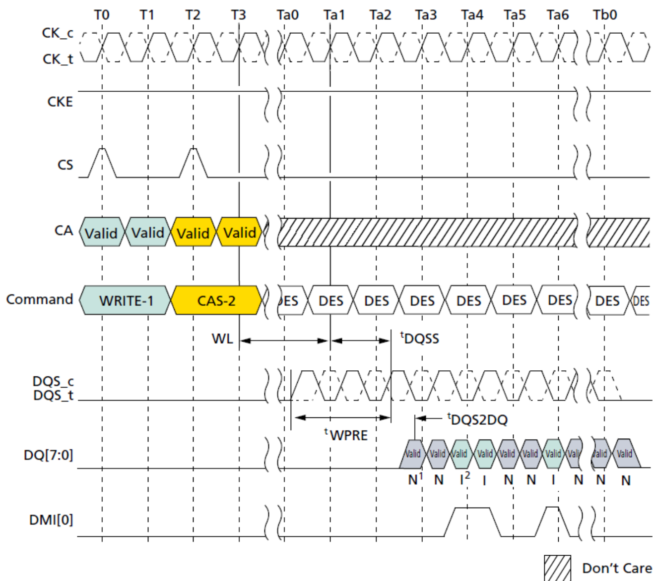
Figure 29. WRITE Command with Write DBI Enabled; DM Disabled
