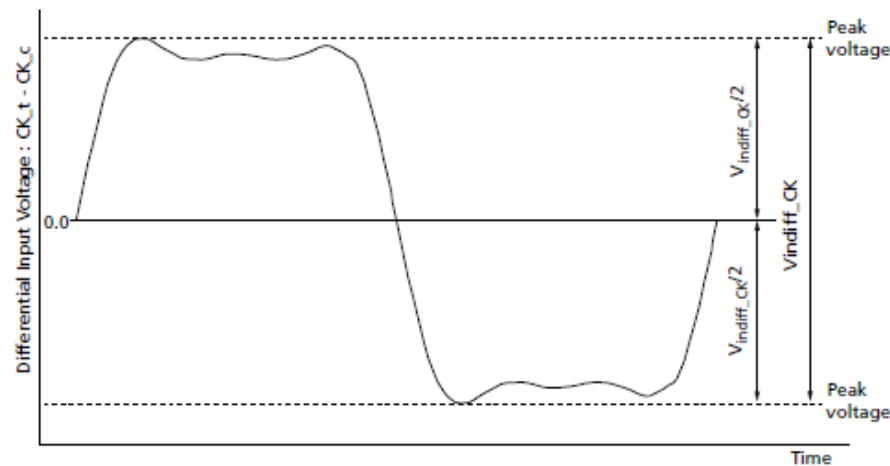
Figure 144. CK Differential Input Voltage
