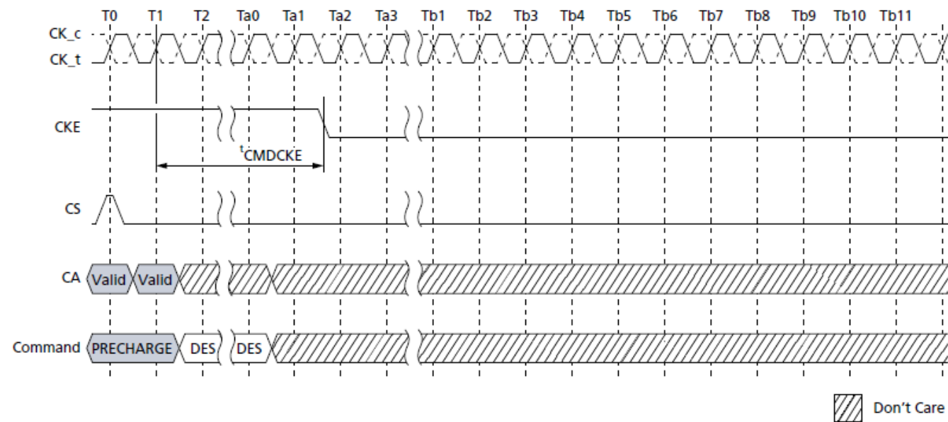
Figure 82. PRECHARGE Command to Power-Down Entry
