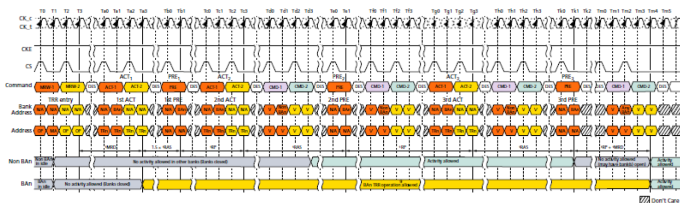
Figure 139. Target Row Refresh Mode
