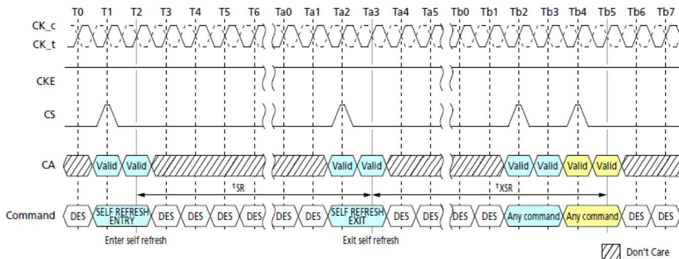
Figure 71. Self Refresh Entry/Exit Timing
