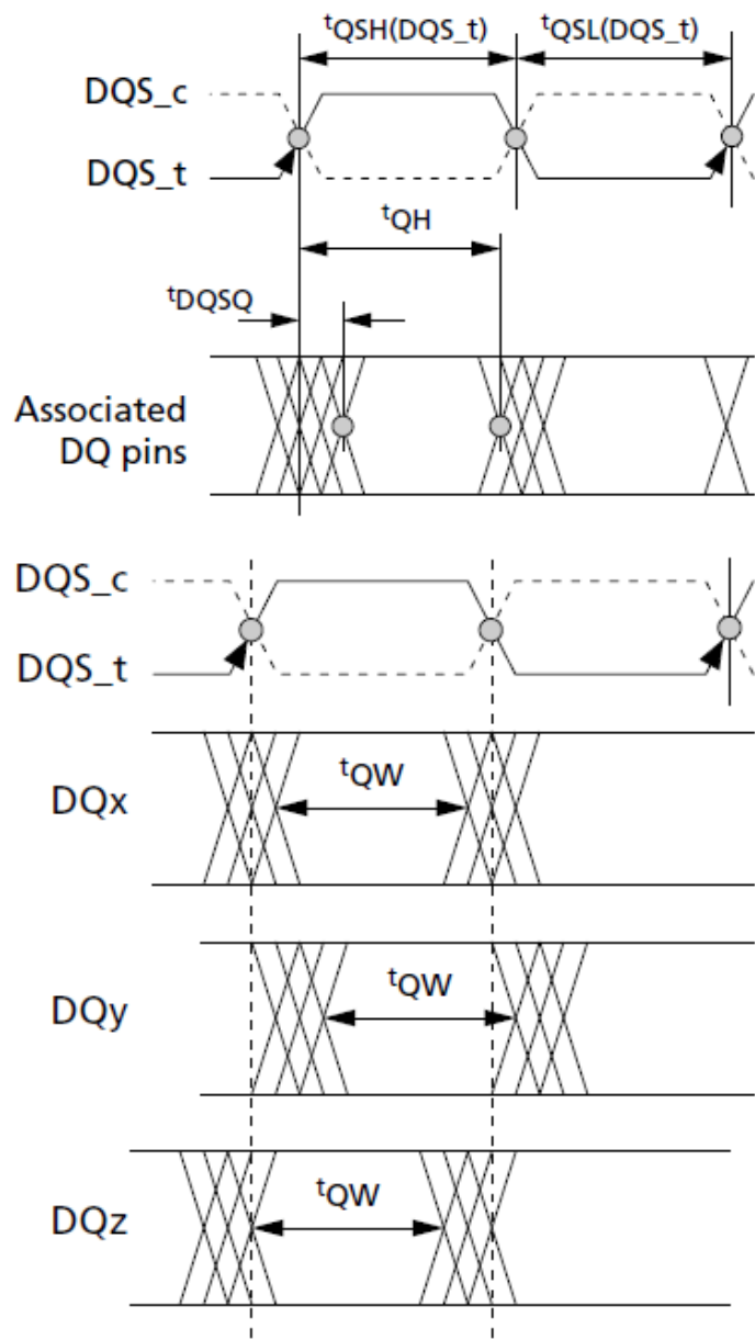
Figure 167. Read Data Timing Definitions – t_{QH} and t_{DQSQ} Across DQ Signals per DQS Group
