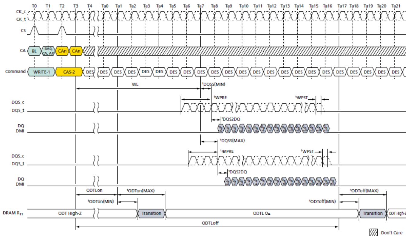
Figure 138. Asynchronous ODTon/ODToff Timing
