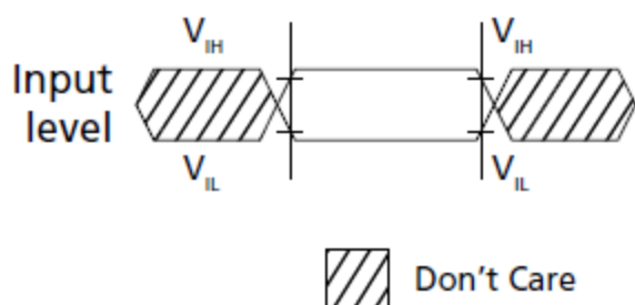
Figure 143. Input Timing Definition for RESET_n
