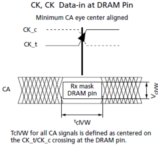
Figure 164. CA Timings at the DRAM Pins
