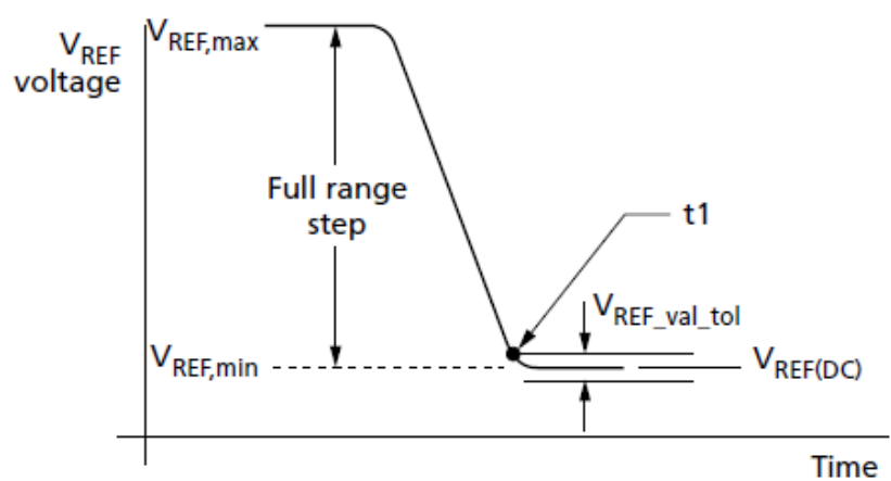
Figure 106. V_{REF(DQ)} Full Step from V_{REF,max} to V_{REF,min}
