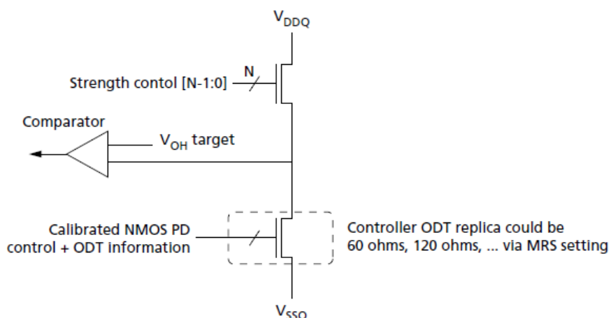
Figure 159. Pull-Up Calibration
