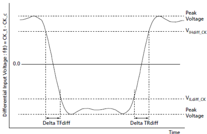
Figure 152. Differential Input Slew Rate Definition for DQS t , DQS c
