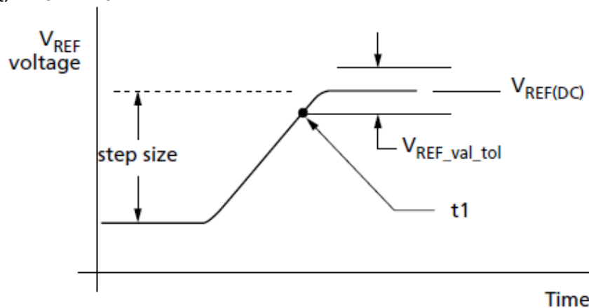
Figure 103. V_{REF(DQ)} Single-Step Size Increment
