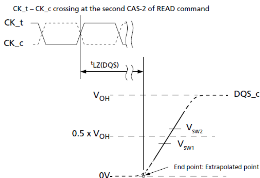
Figure 17. t_{LZ}(DQS) Method for Calculating Transitions and Endpoint
