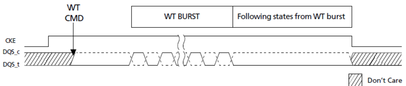
Figure 30. WDQS Control Mode 1
