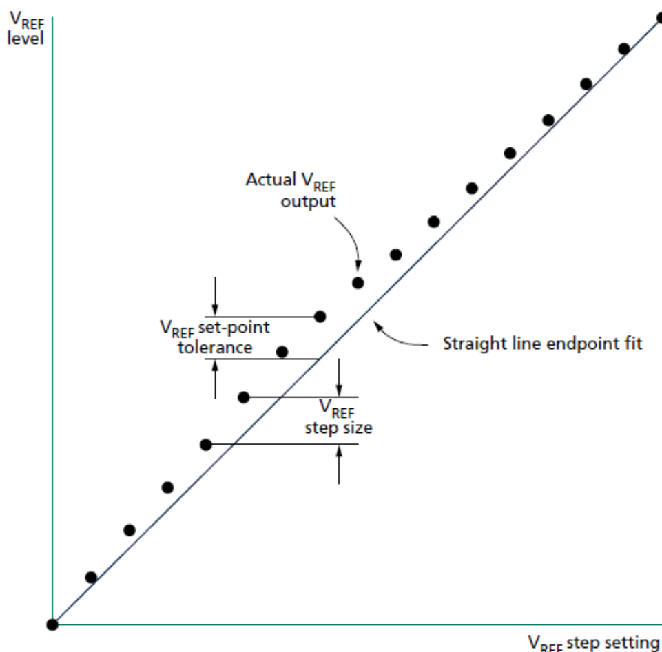
Figure 101. V_{REF} Set Tolerance and Step Size
