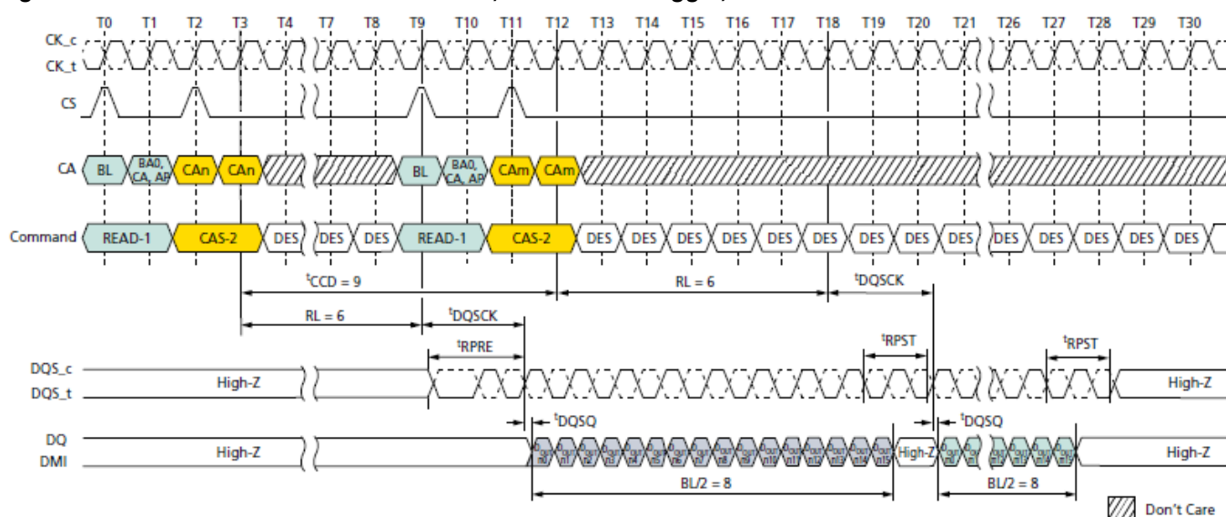
Figure 35. Seamless READ: t_{CCD} = MIN + 1 , Preamble = Toggle, 1.5nCK Postamble
