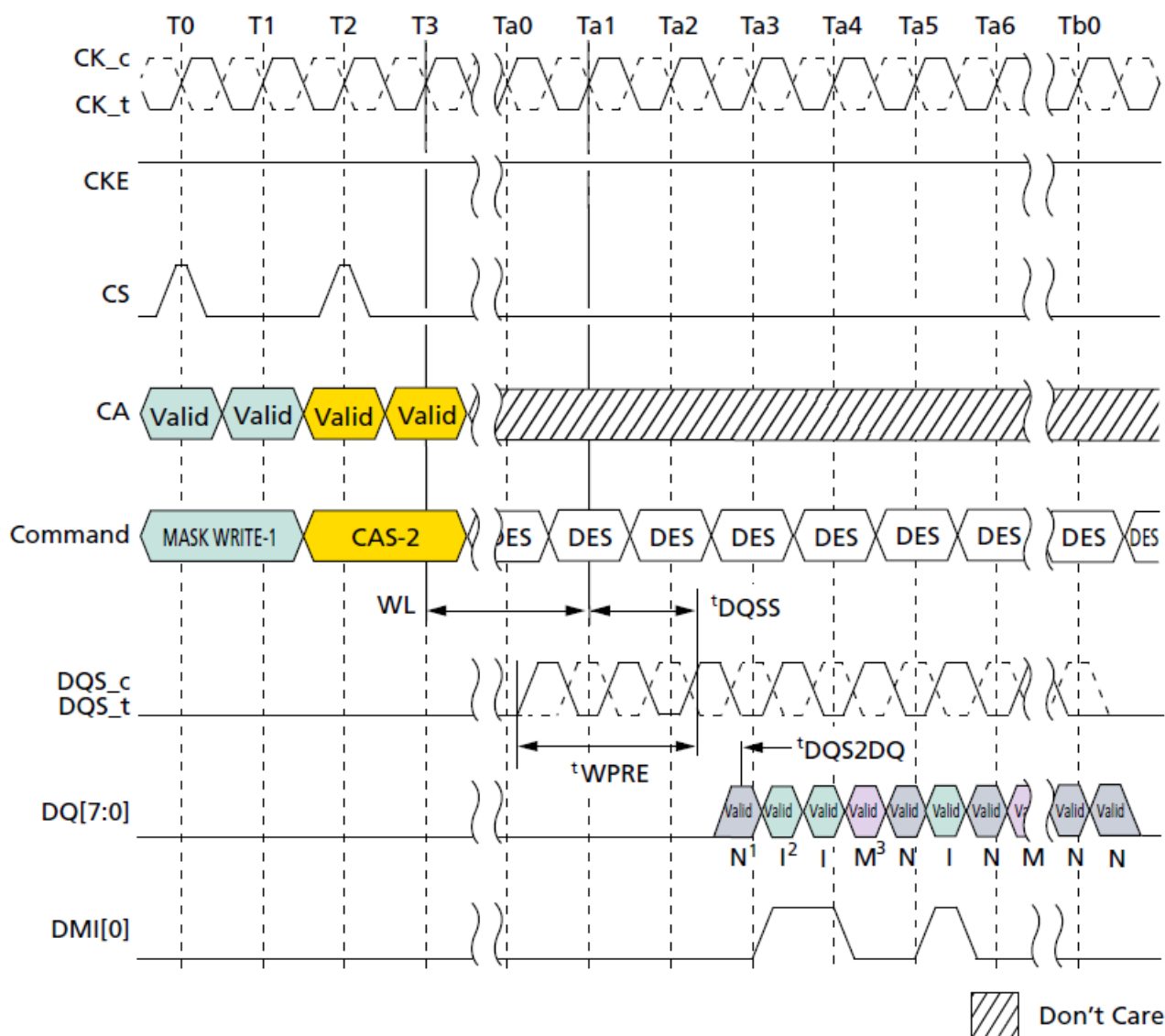
Figure 28. MASKED WRITE Command with Write DBI Enabled; DM Enabled
