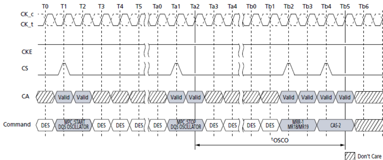
Figure 127. In Case of DQS Interval Oscillator is Stopped by MPC Command
