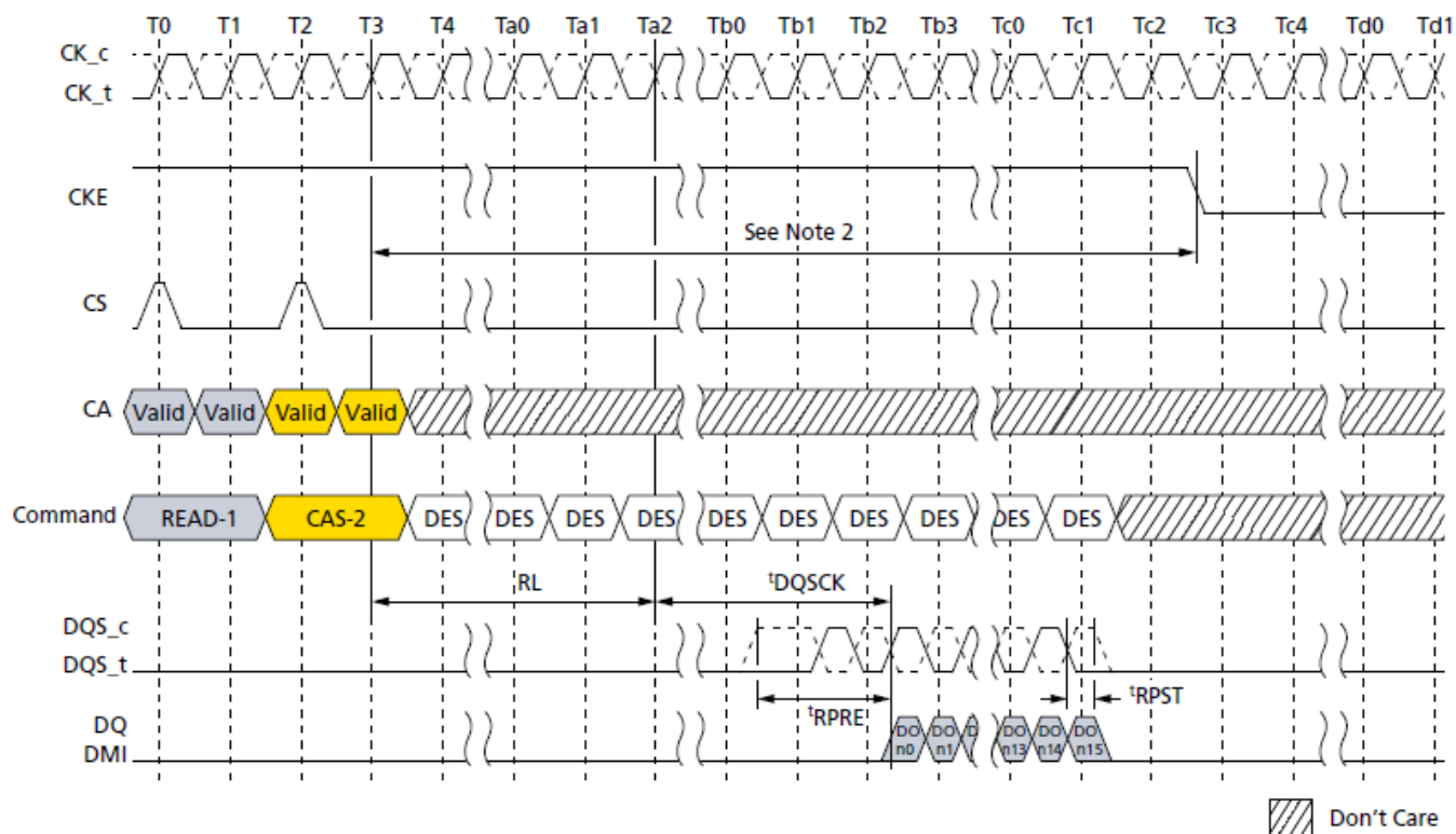
Figure 77. Read and Read with Auto Precharge to Power-Down Entry
