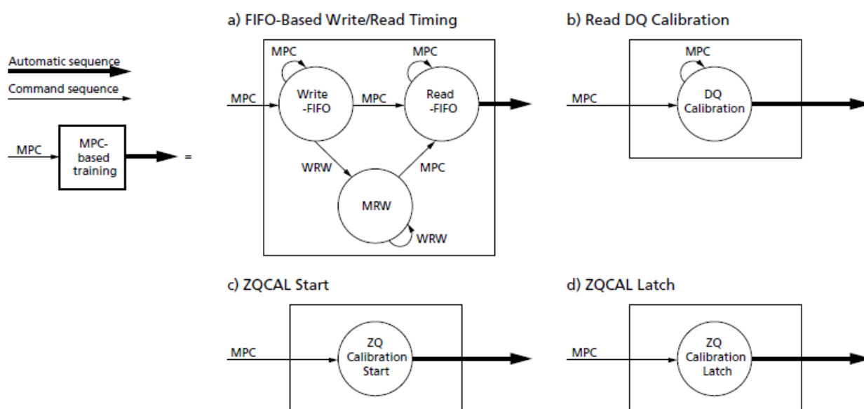
Figure 5. Simplified State Diagram
