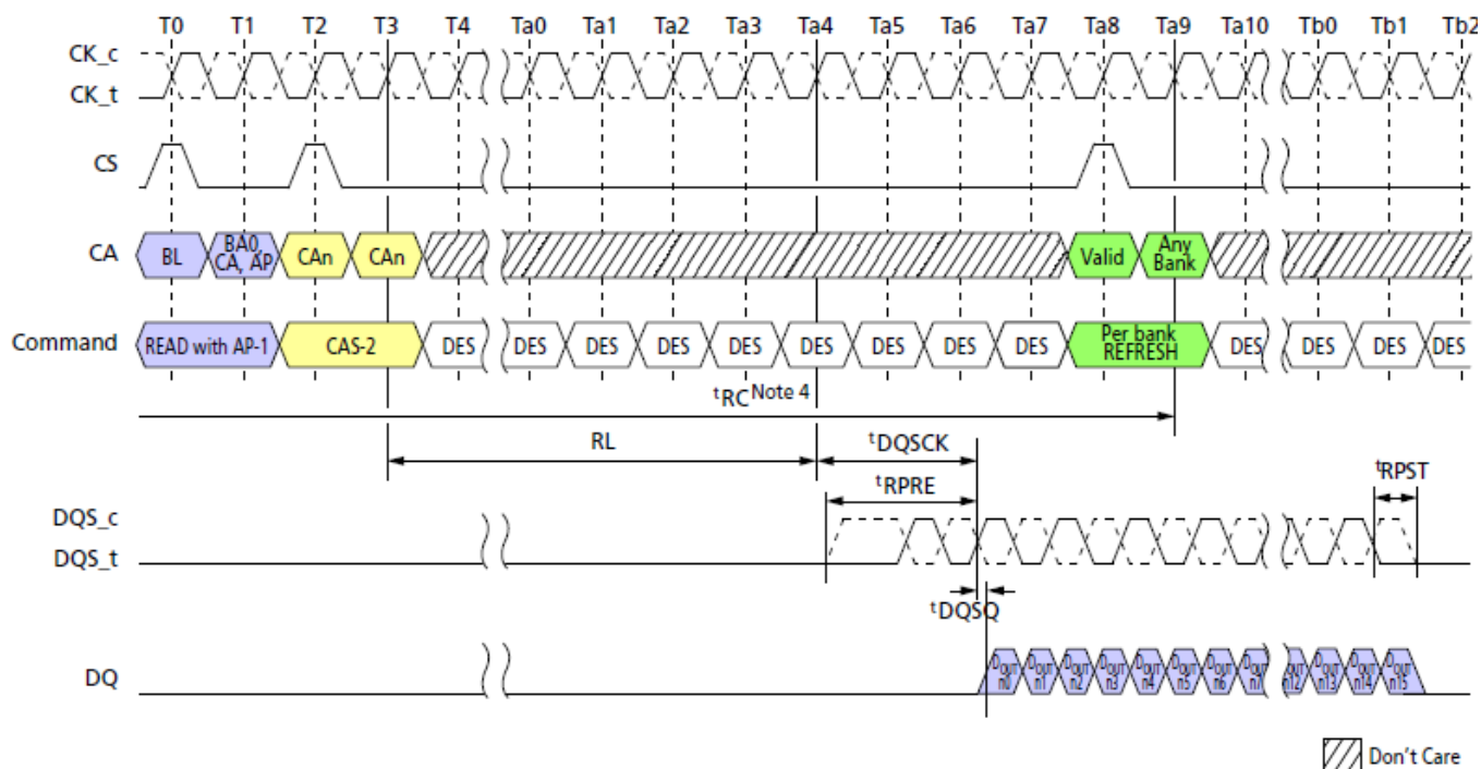
Figure 70. Burst READ With AUTO PRECHARGE Operation Followed by Per Bank Refresh
