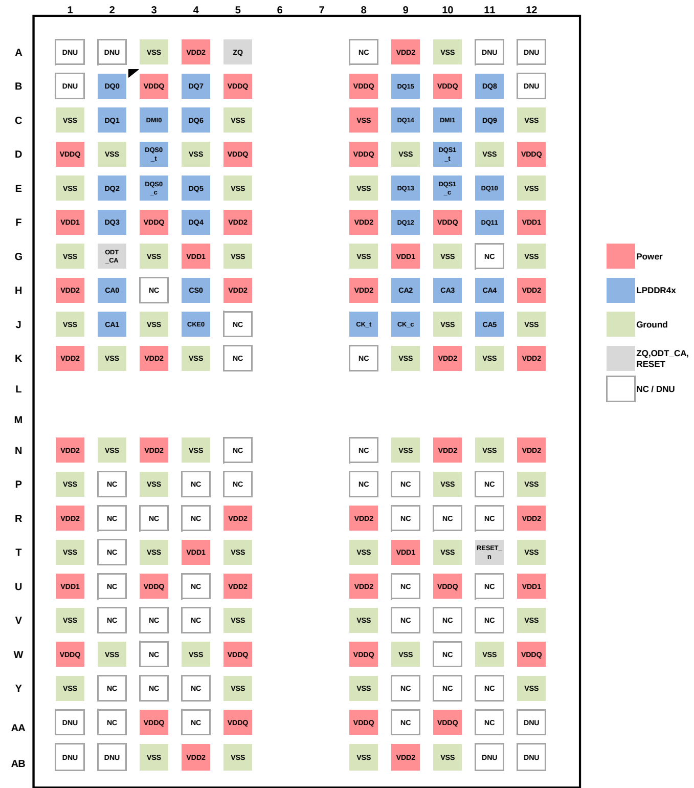
Figure 2. Ball Configuration (Top View)
