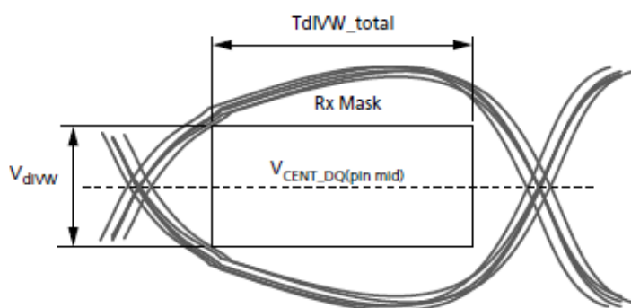
Figure 168. DQ Receiver (Rx) Mask
