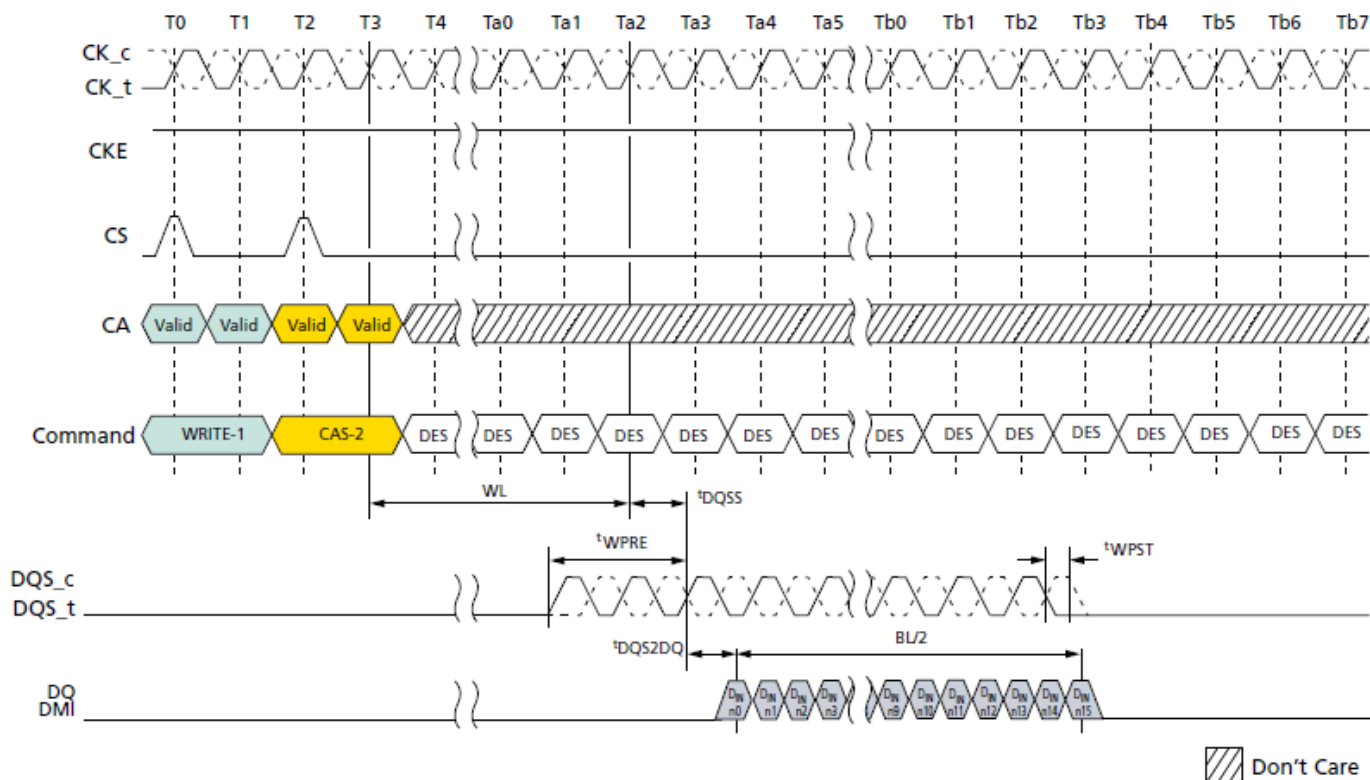
Figure 11. DQS Write Preamble and Postamble – 0.5nCK Postamble
