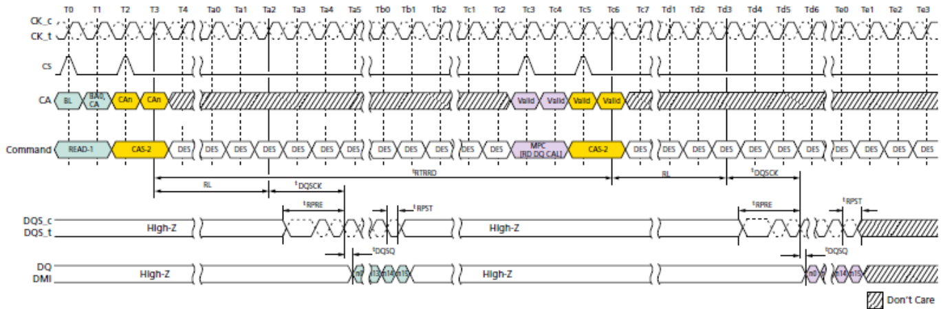
Figure 118. Read DQ Calibration Training Timing: Read-to-Read DQ Calibration
