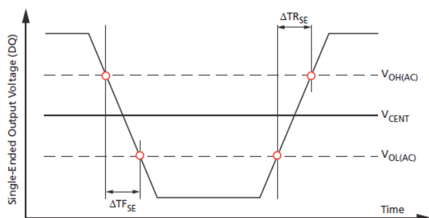
Figure 179. Single-Ended Output Slew Rate Definition
