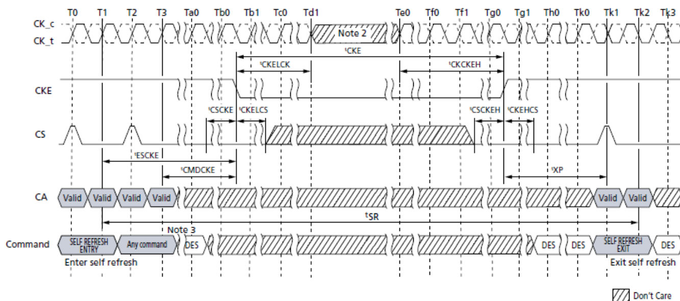
Figure 72. Self Refresh Entry/Exit Timing with Power-Down Entry/Exit
