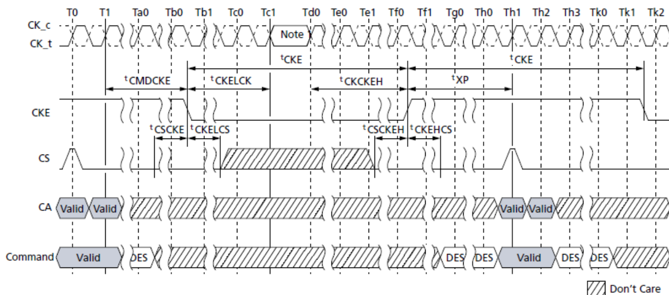
Figure 76. Basic Power-Down Entry and Exit Timing
