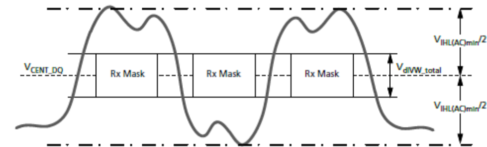
Figure 172. DQ V_{IHL(AC)} Definition (for Each Input Pulse)
