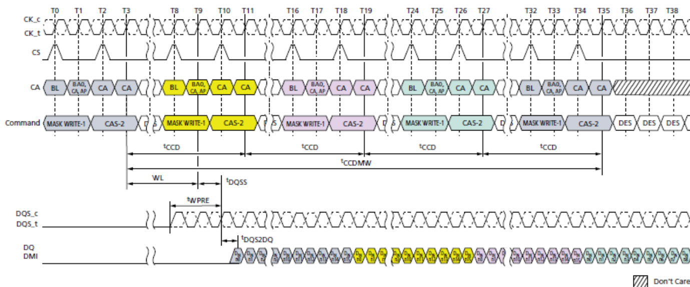
Figure 27. MASK WRITE Command – Different Bank
