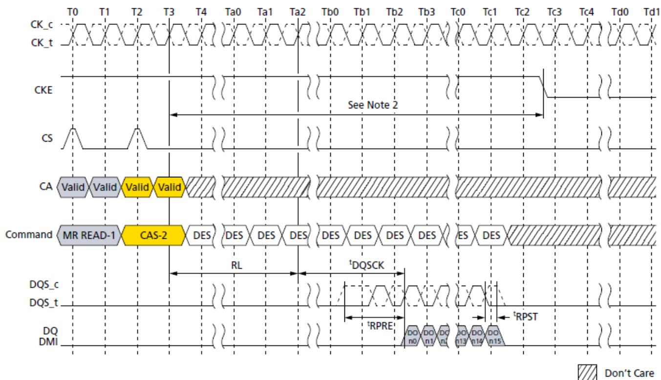
Figure 83. Mode Register Read to Power-Down Entry
