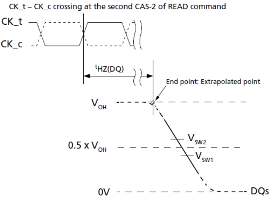
Figure 20. t HZ(DQ) Method for Calculating Transitions and Endpoint
