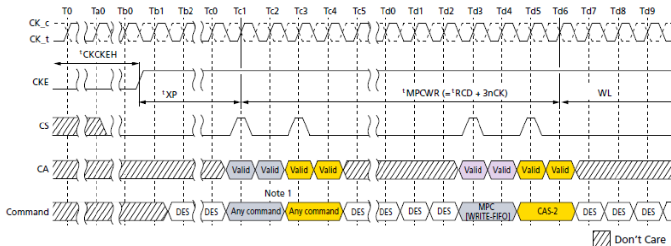
Figure 125. Power-Down Exit to MPC[WRITE-FIFO] Timing
