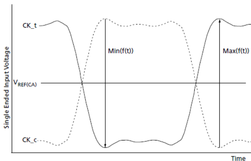
Figure 145. Definition of Differential Clock Peak Voltage
