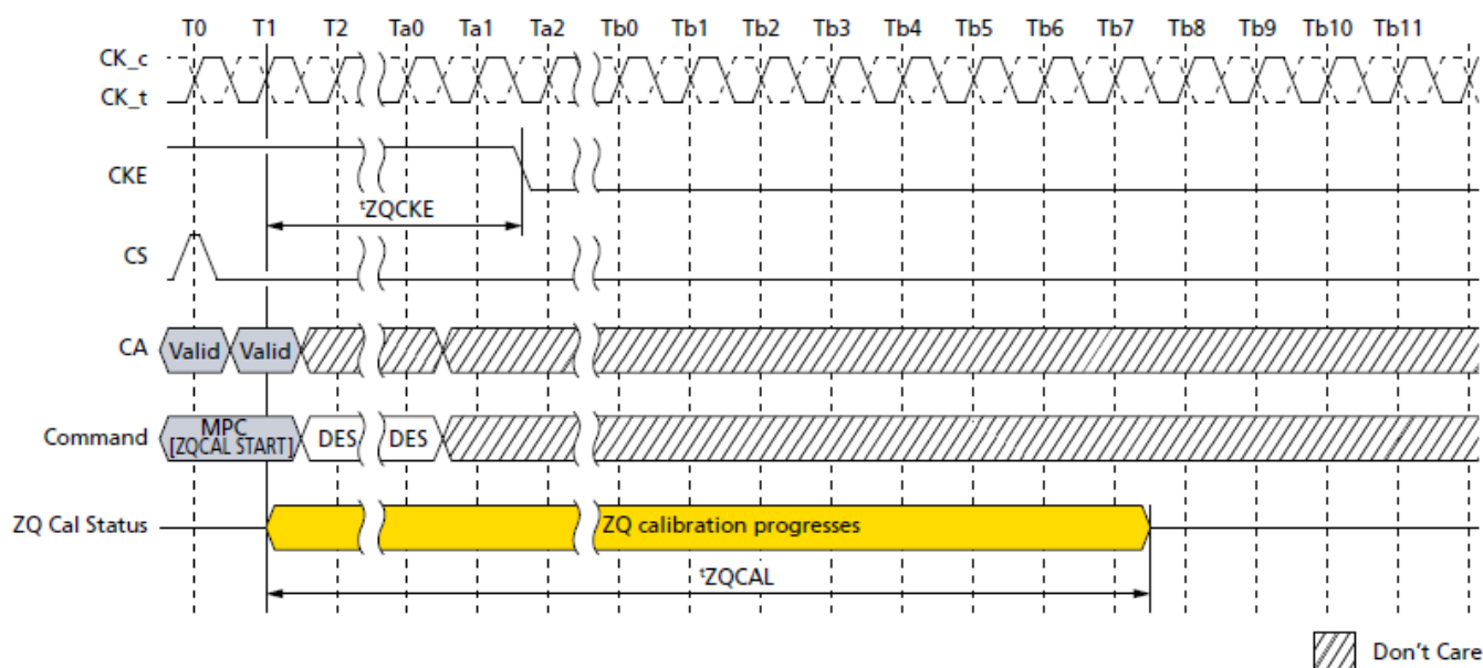
Figure 85. MULTI PURPOSE Command for ZQCAL Start to Power-Down Entry
