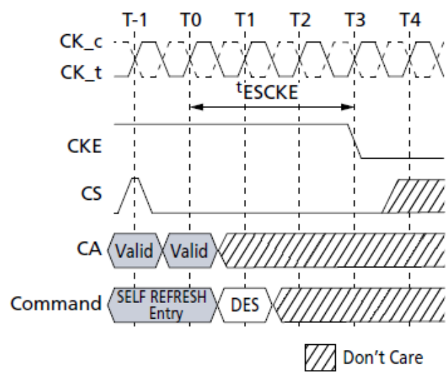
Figure 161. t ESCKE Timing
