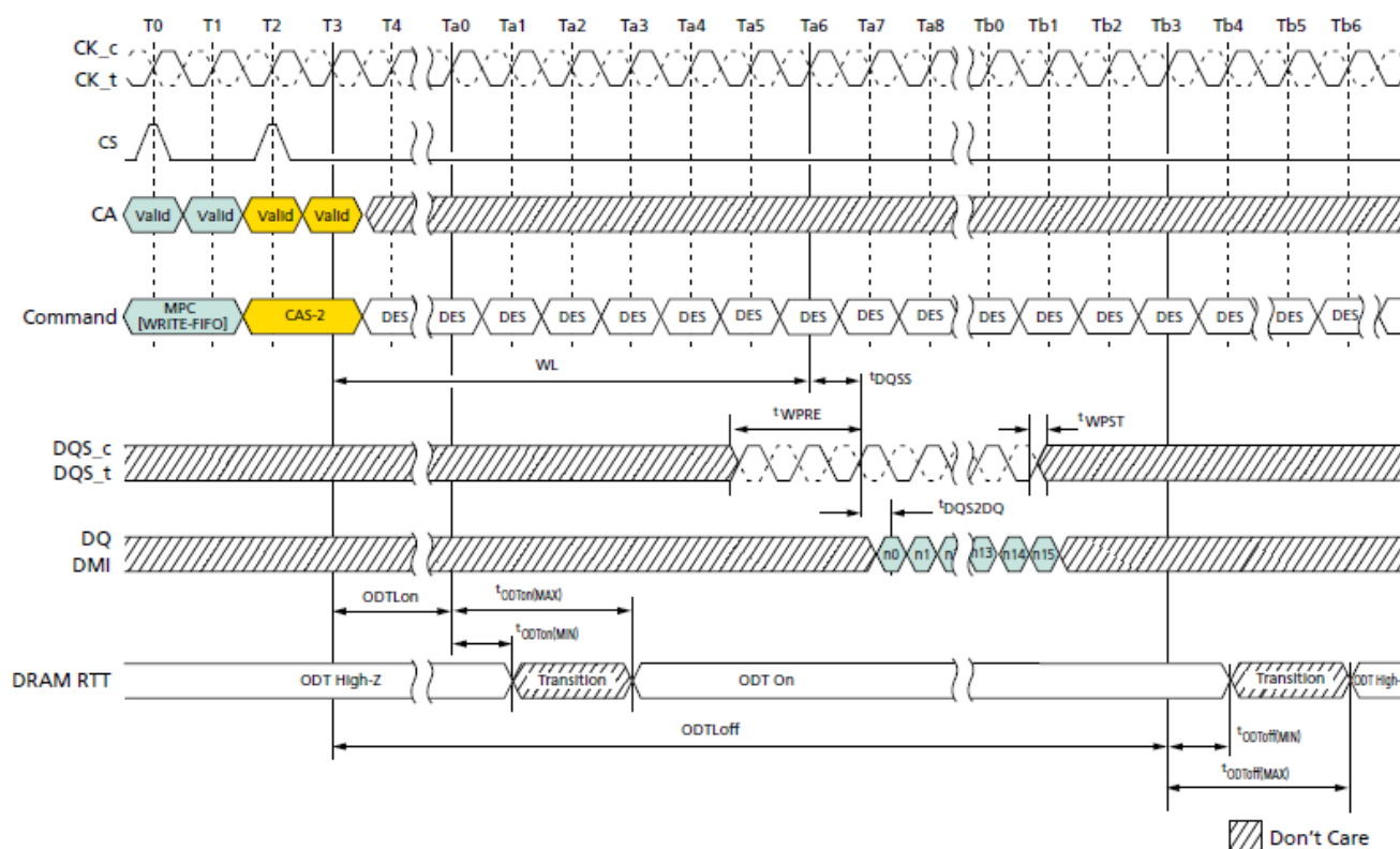
Figure 124. MPC[WRITE-FIFO] with DQ ODT Timing
