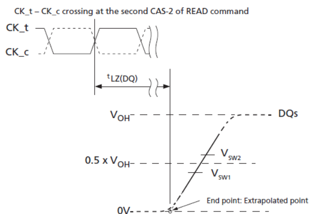
Figure 175. t LZ(DQ) Method for Calculating Transitions and Endpoint
