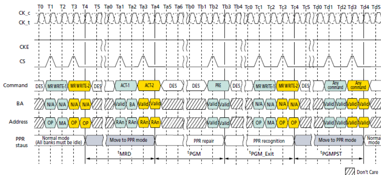
Figure 140. Post-Package Repair Timing
