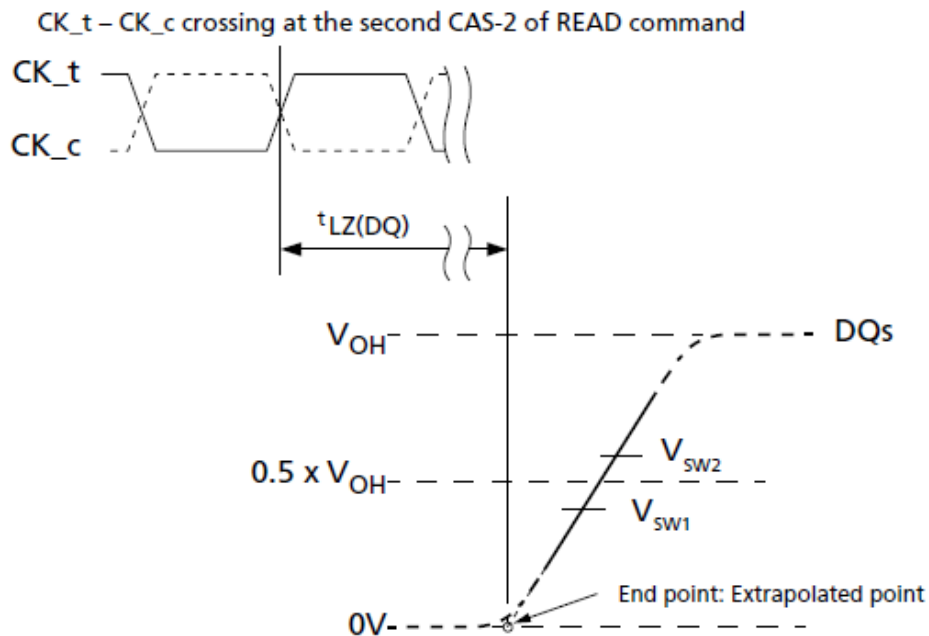
Figure 19. t_{LZ(DQ)} Method for Calculating Transitions and Endpoint
