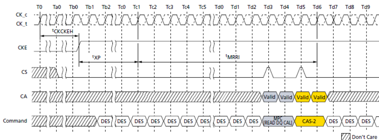
Figure 120. MPC[READ DQ CALIBRATION] Following Power-Down State
