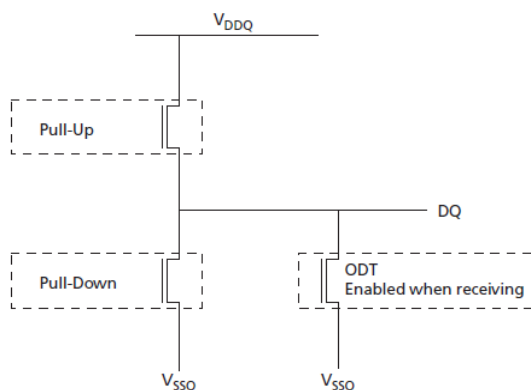
Figure 181. LVSTL I/O Cell
