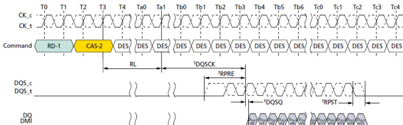
Figure 9. DQS Read Preamble and Postamble – Toggling Preamble and 0.5nCK Postamble
