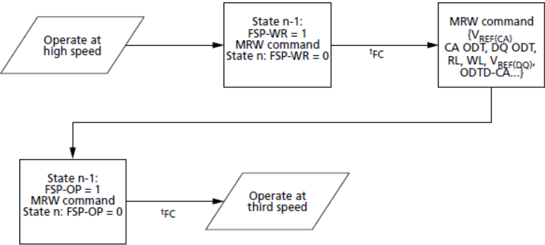
Figure 134. Example of Switching to a Third Trained Frequency Set Point
