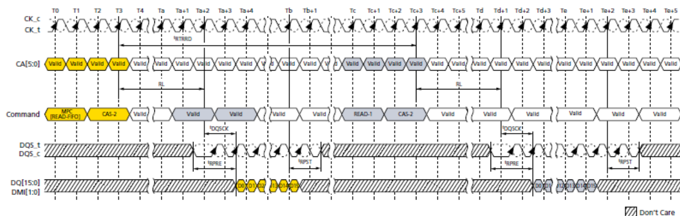
Figure 117. READ-FIFO – t_{RPRE} = \text{Toggleing} , t_{RPST} = 1.5nCK
