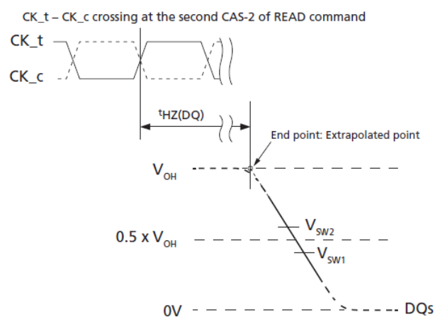
Figure 176. t HZ(DQ) Method for Calculating Transitions and Endpoint
