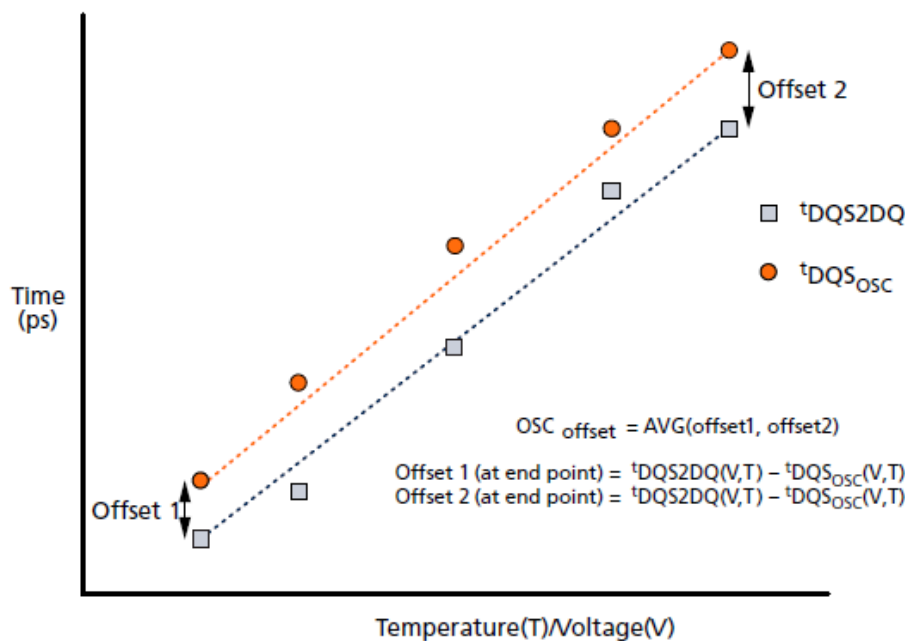
Figure 126. Interval Oscillator Offset – OSC_{Offset}
