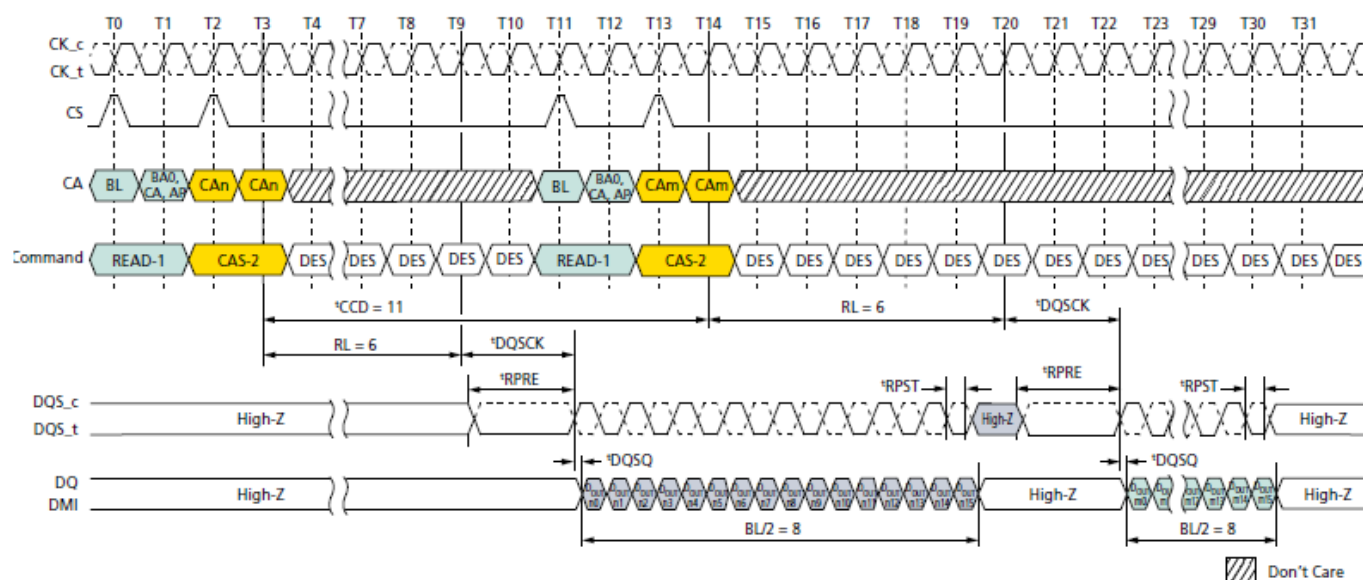
Figure 46. Consecutive READ: t_{CCD} = MIN + 3 , Preamble = Static, 0.5nCK Postamble
