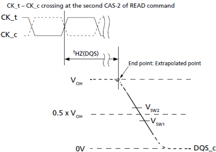
Figure 18. t HZ(DQS) Method for Calculating Transitions and Endpoint
