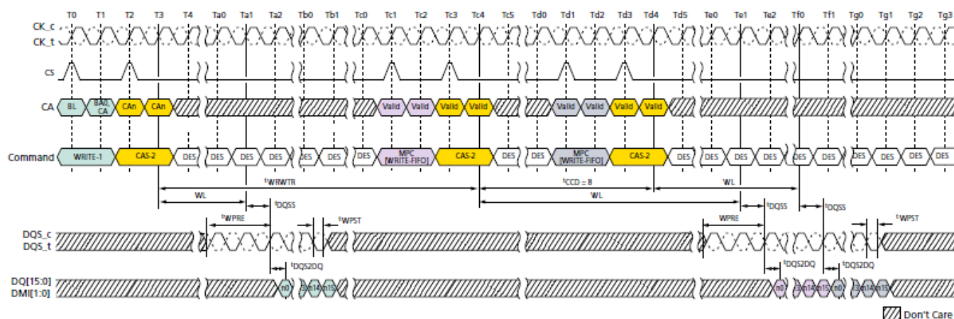
Figure 121. WRITE-to-MPC[WRITE-FIFO] Operation Timing
