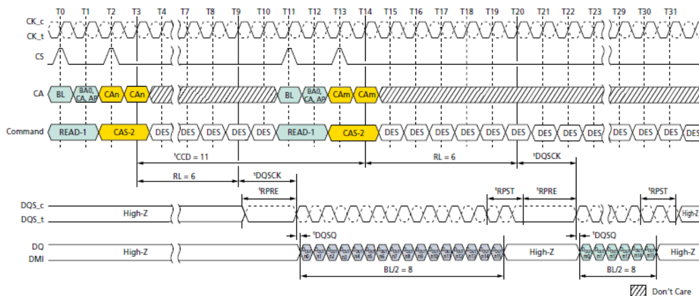
Figure 45. Consecutive READ: t_{CCD} = MIN + 3 , Preamble = Static, 1.5nCK Postamble
