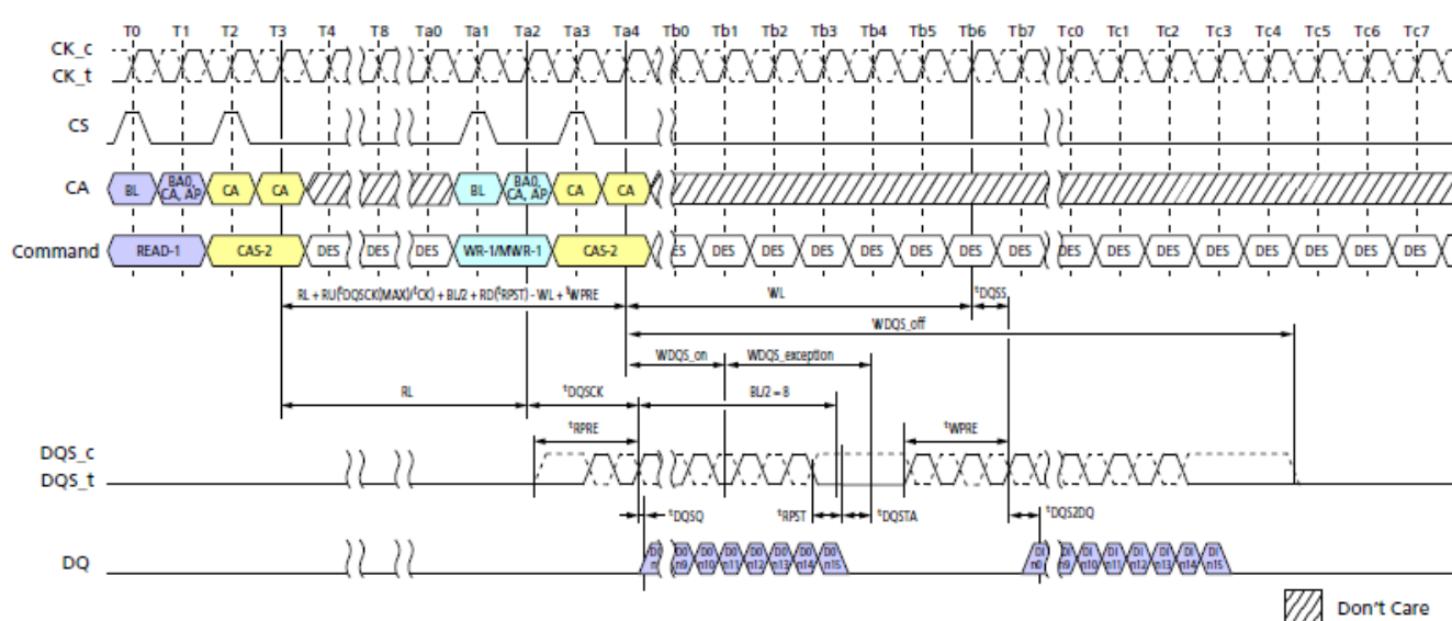
Figure 32. Burst READ Followed by Burst WRITE or Burst MASKED WRITE (ODT Disable)
