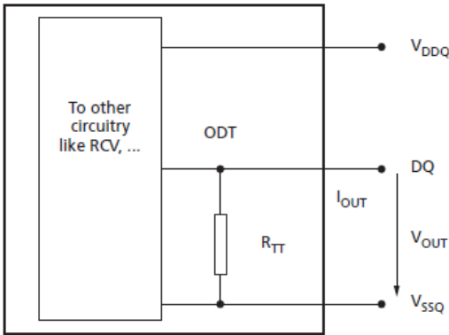
Figure 178. Functional Representation of DQ ODT
