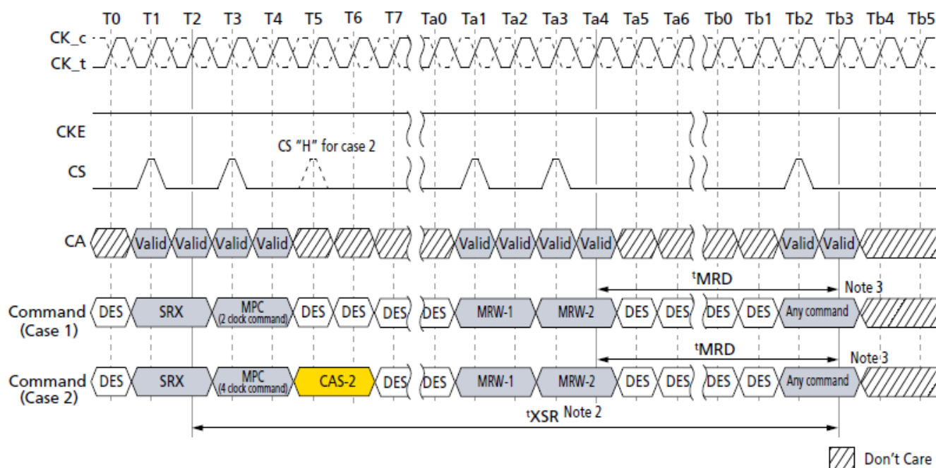
Figure 74. MRR, MRW, and MPC Commands Issuing Timing During t XSR
