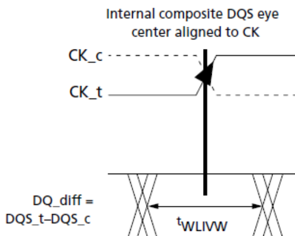
Figure 114. DQS_t/DQS_c to CK_t/CK_c Timings at the Pins Referenced from the Internal Latch
