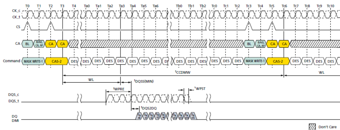
Figure 26. MASK WRITE Command – Same Bank
