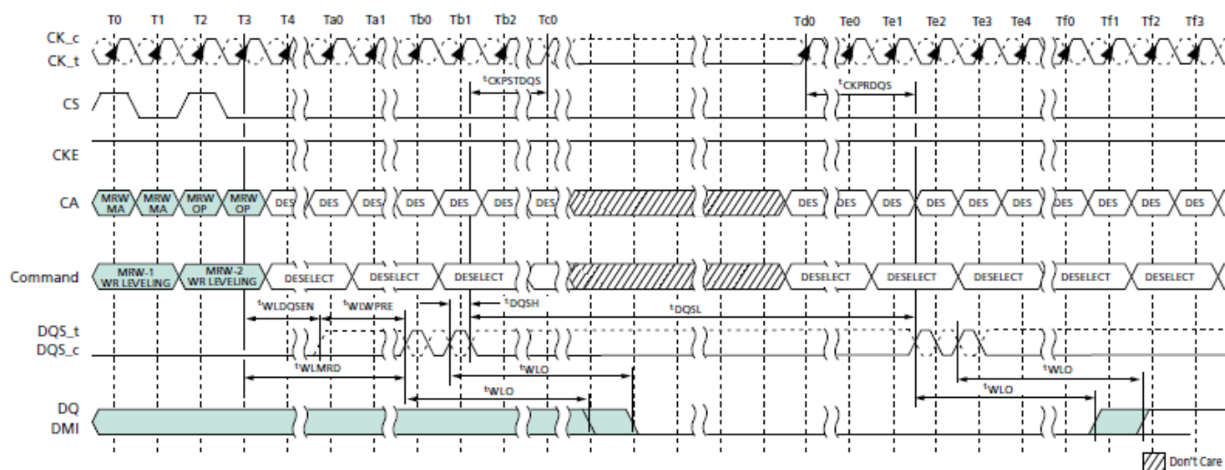
Figure 113. Clock Stop and Timing During Write Leveling
