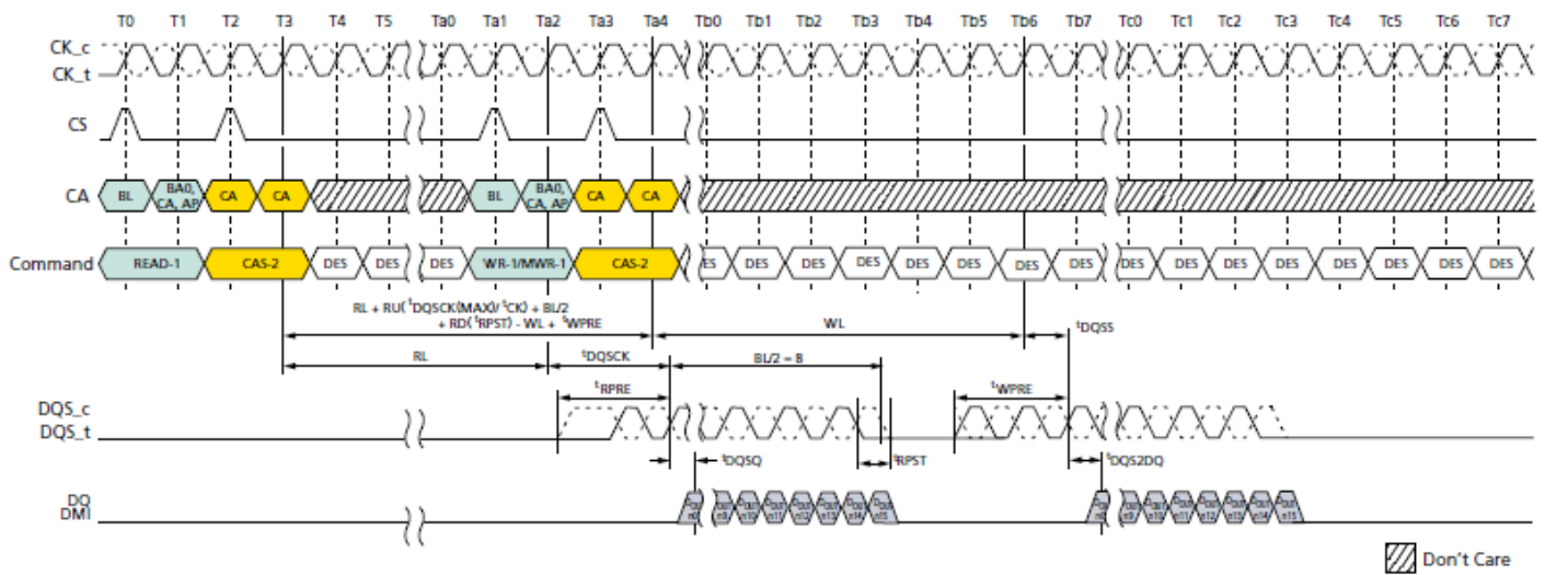
Figure 14. Burst Read Followed by Burst Write or Burst Mask Write
