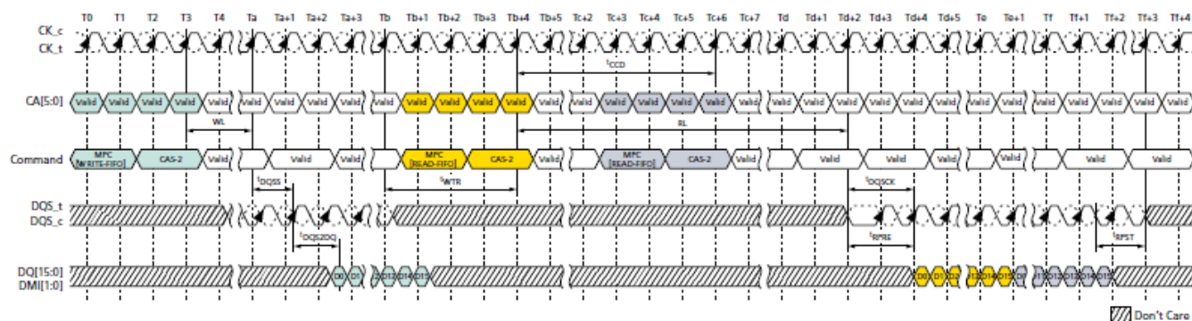
Figure 116. READ-FIFO – t_{WPRE} = 2nCK , t_{WPST} = 0.5nCK , t_{RPRE} = \text{Toggle} , t_{RPST} = 1.5nCK
