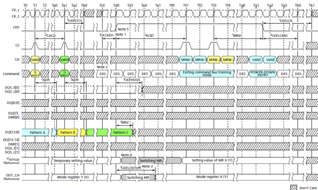
Figure 110. Command Bus Training Mode Exit with Power-Down Entry
