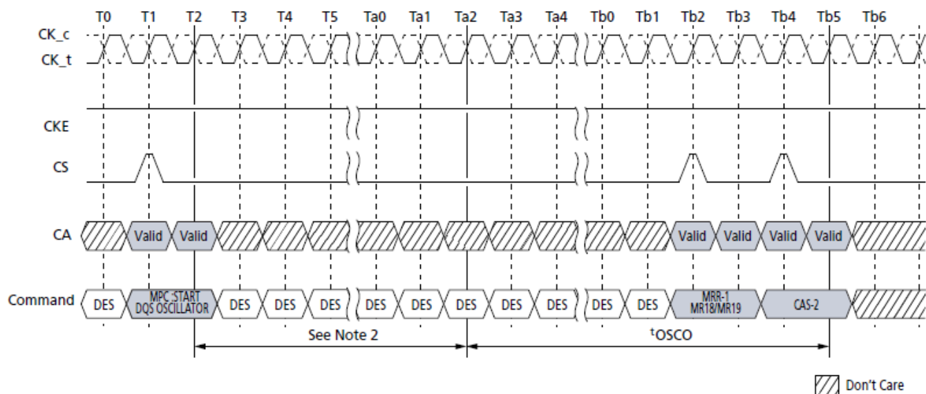
Figure 128. In Case of DQS Interval Oscillator is Stopped by DQS Interval Timer
