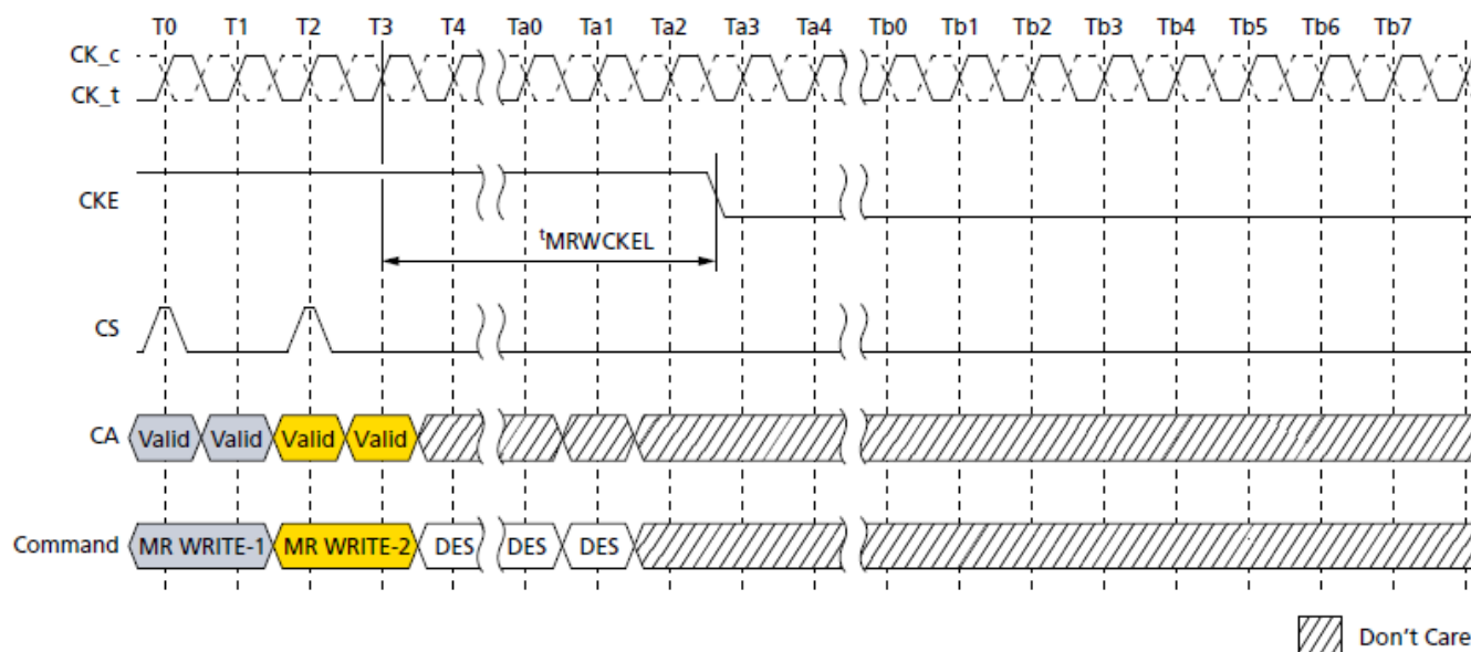
Figure 84. Mode Register Write to Power-Down Entry
