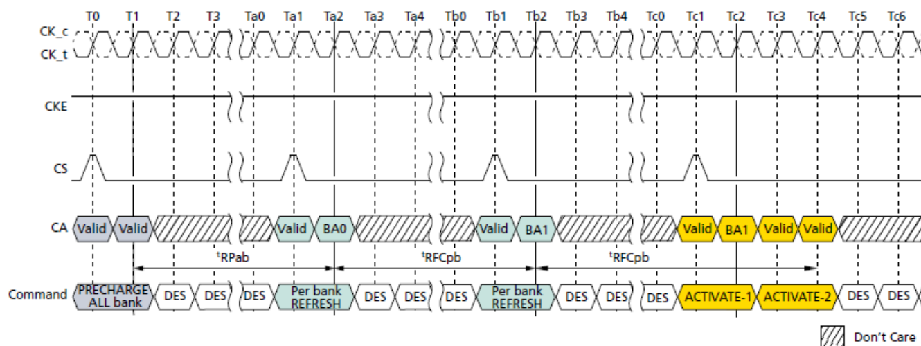
Figure 66. Per Bank REFRESH Operation
