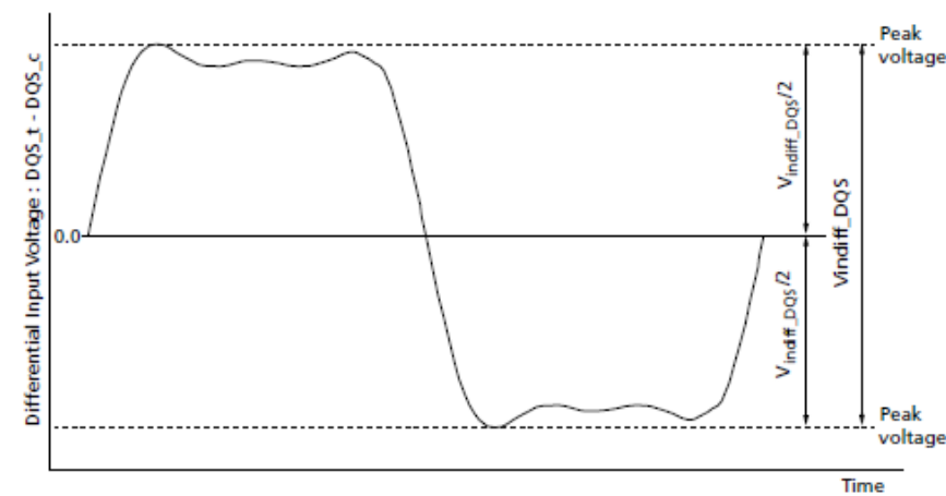
Figure 149. DQS Differential Input Voltage
