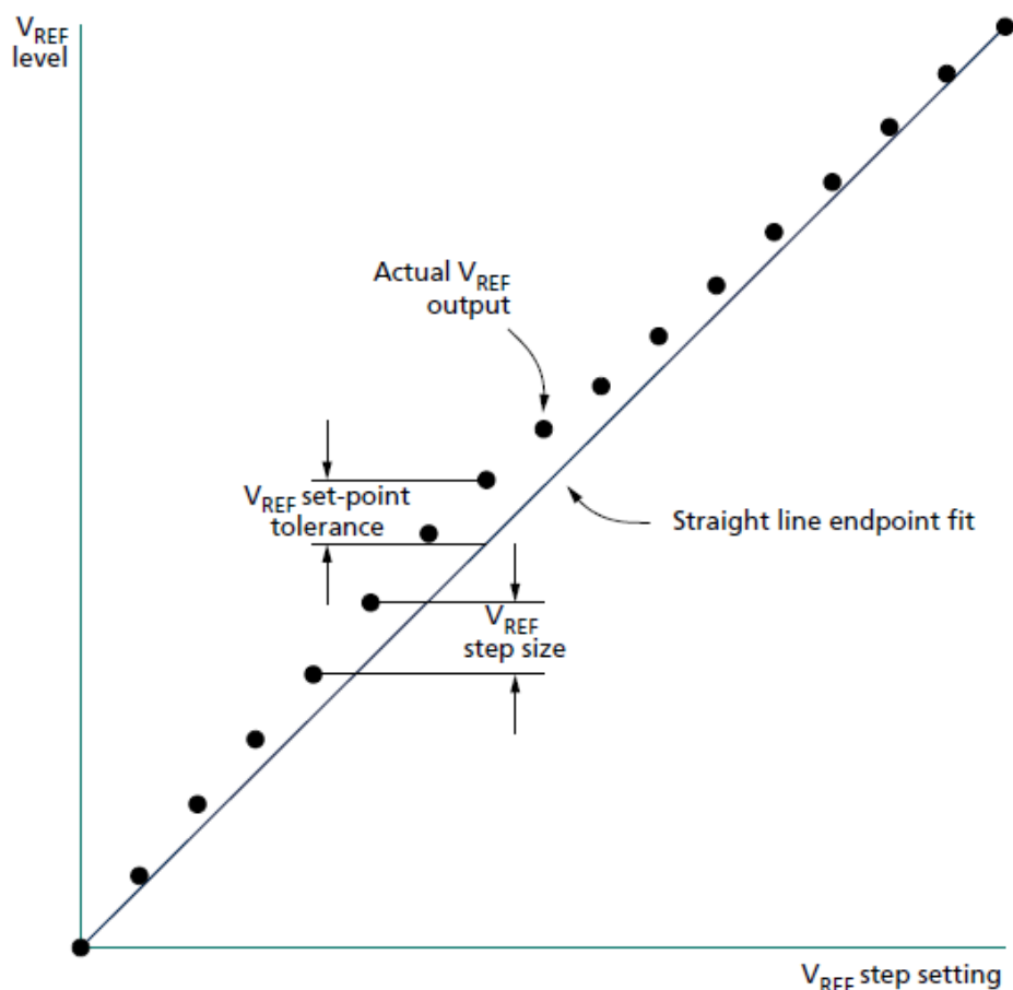
Figure 94. V_{REF} Set-Point Tolerance and Step Size
