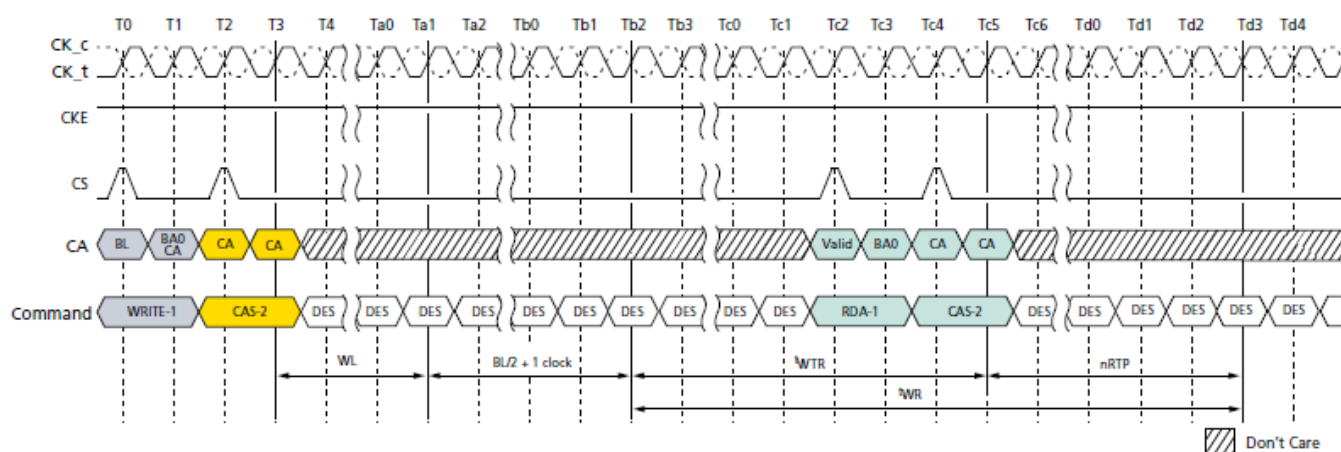
Figure 64. Delay Time From WRITE-to-READ with Auto Precharge
