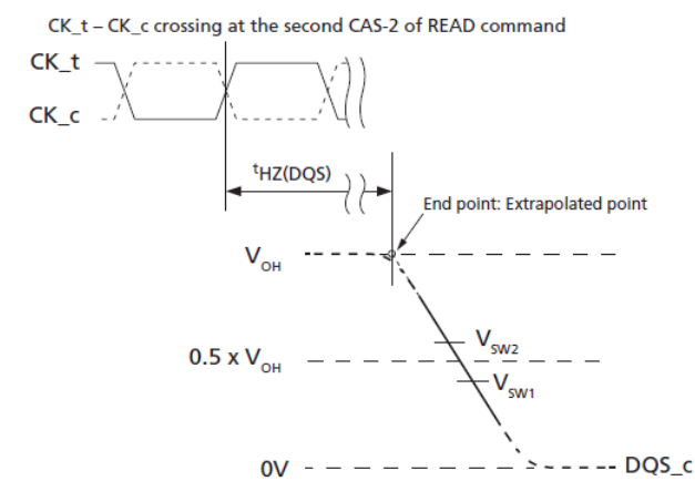
Figure 174. t HZ(DQS) Method for Calculating Transitions and Endpoint
