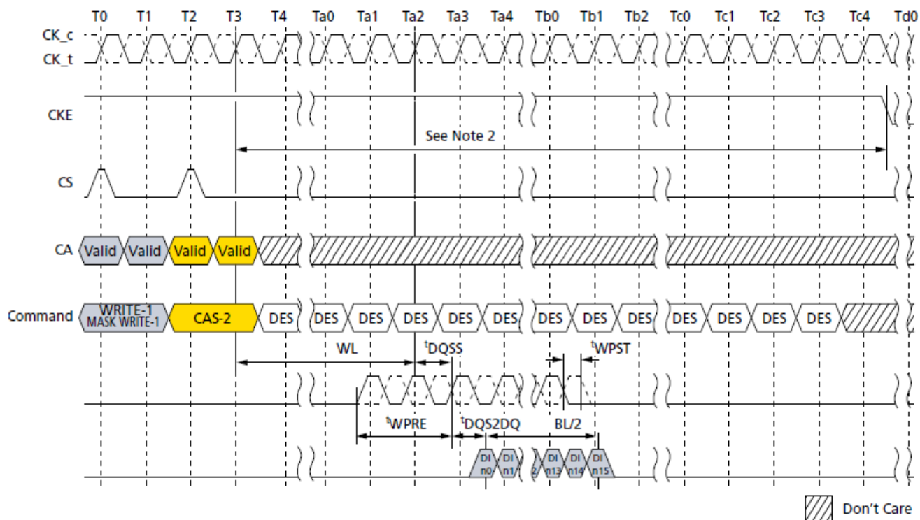
Figure 79. Write With Auto Precharge and Mask Write With Auto Precharge to Power-Down Entry
