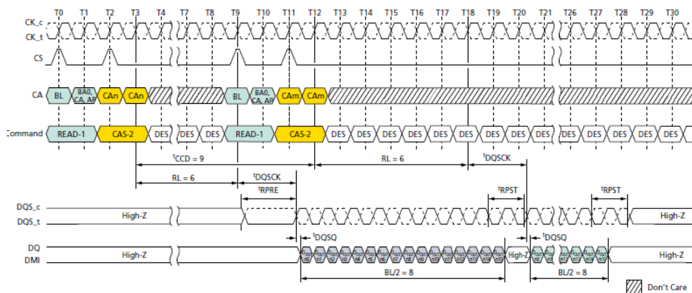
Figure 37. Consecutive READ: t_{CCD} = MIN + 1 , Preamble = Static, 1.5nCK Postamble
