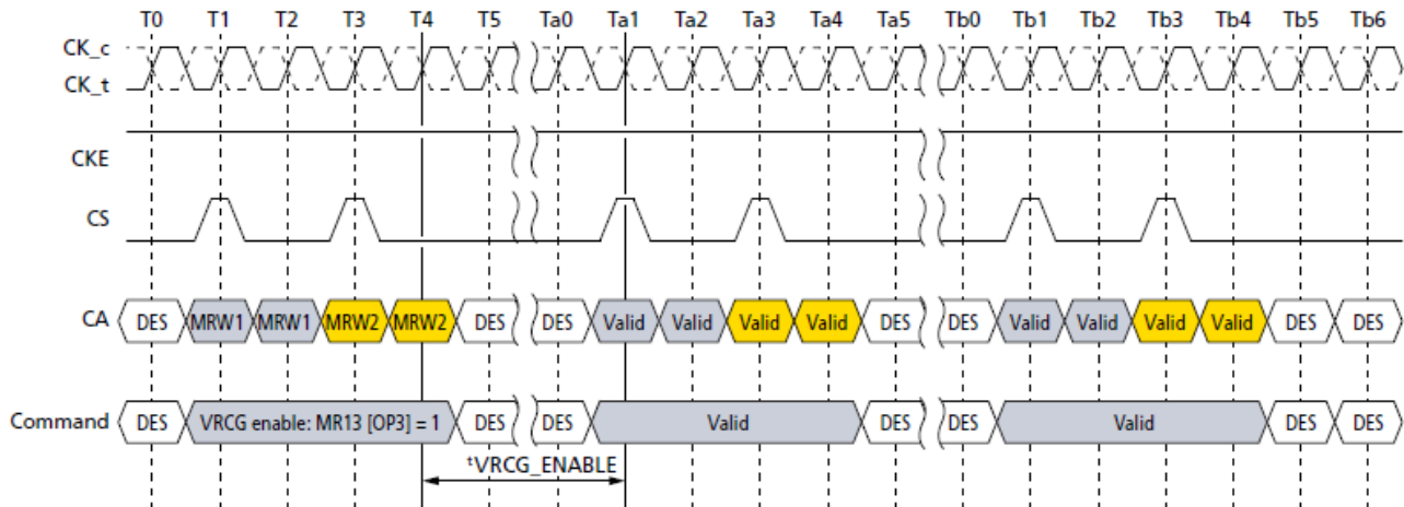
Figure 91. VRCG Enable Timing
