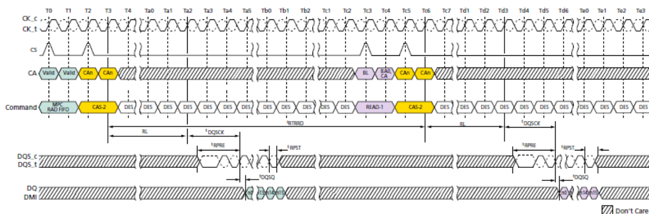
Figure 123. MPC[READ-FIFO] to Read Timing
