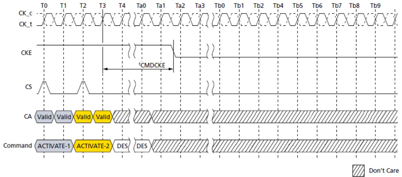
Figure 81. ACTIVATE Command to Power-Down Entry
