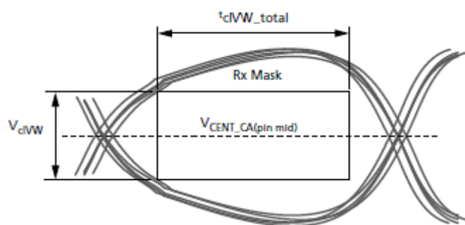
Figure 162. CA Receiver (Rx) Mask
