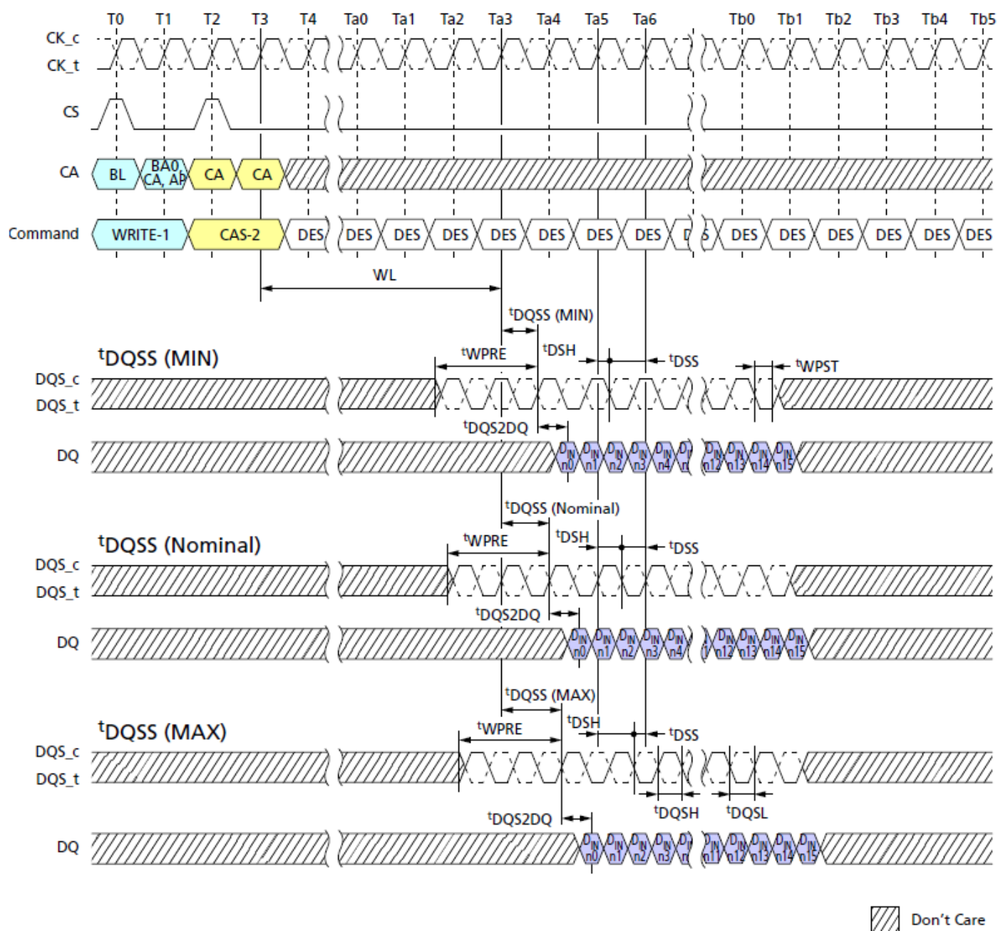
Figure 23. Write Timing
