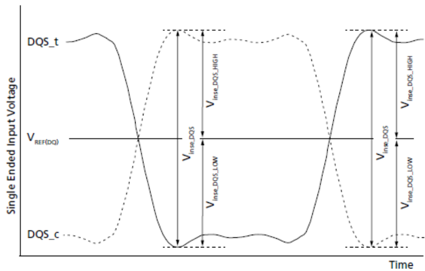
Figure 151. DQS Single-Ended Input Voltage
