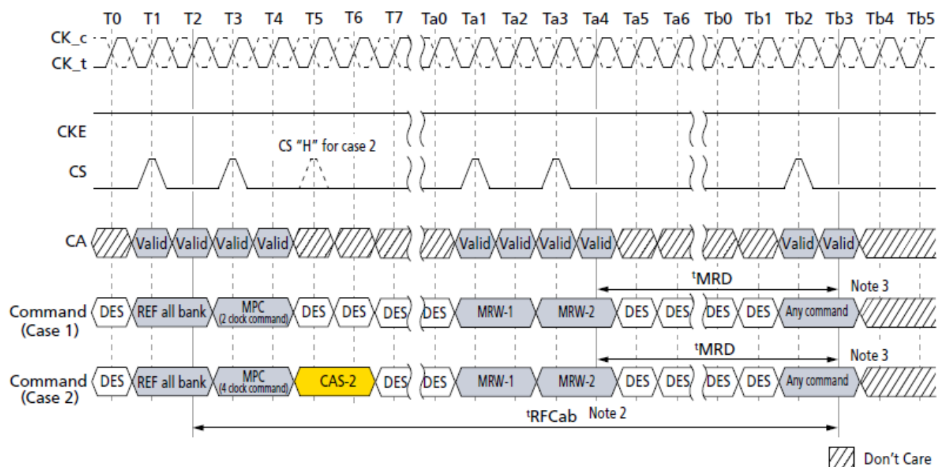
Figure 75. MRR, MRW, and MPC Commands Issuing Timing During t_{RFC}
