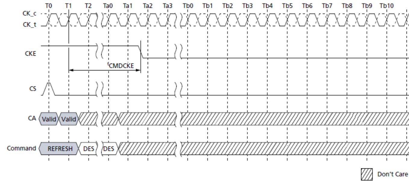
Figure 80. Refresh Entry to Power-Down Entry
