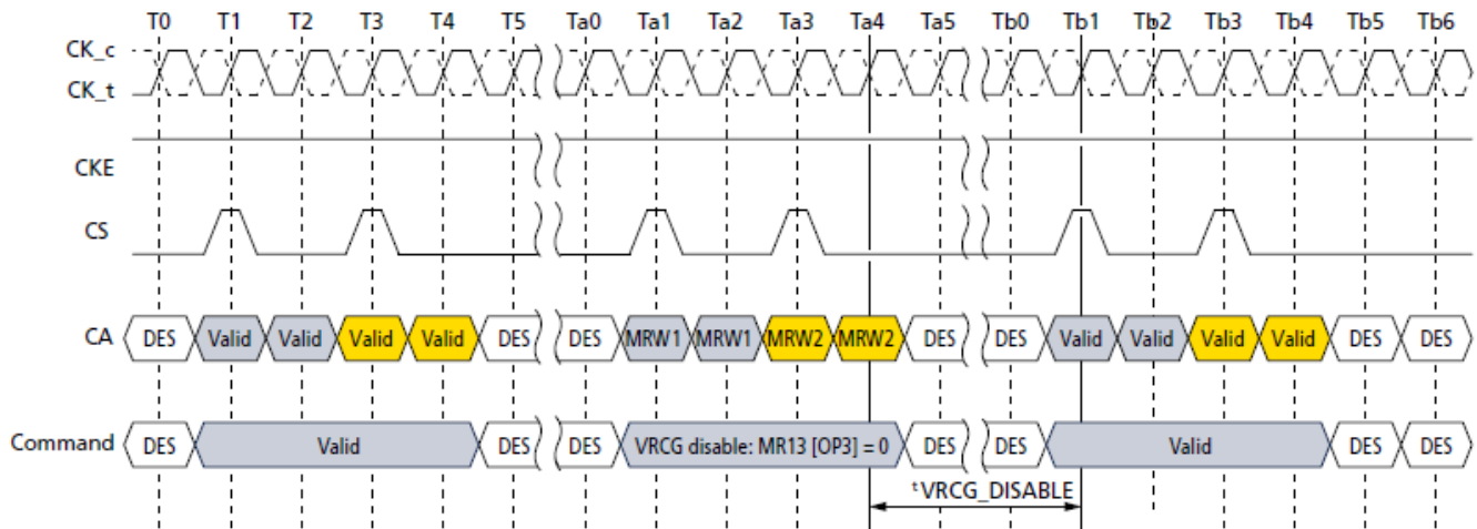
Figure 92. VRCG Disable Timing
