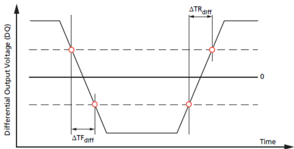
Figure 155. Differential Output Slew Rate Definition
