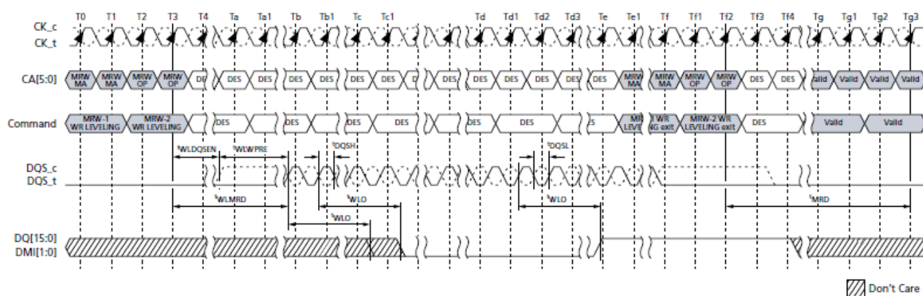
Figure 112. Write Leveling Timing – t_{DQSL}(\text{MIN})
