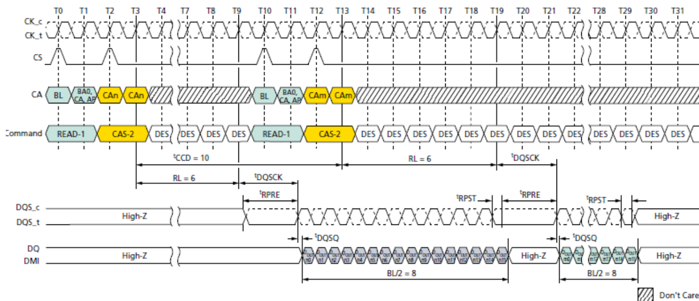
Figure 42. Consecutive READ: t_{CCD} = MIN + 2 , Preamble = Static, 0.5nCK Postamble
