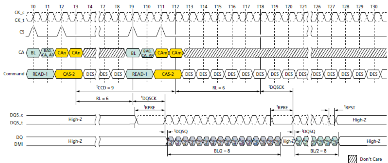
Figure 38. Consecutive READ: t_{CCD} = MIN + 1 , Preamble = Static, 0.5nCK Postamble
