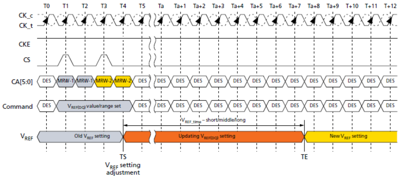
Figure 102. V_{REF(DQ)} Transition Time for Short, Middle, or Long Changes
