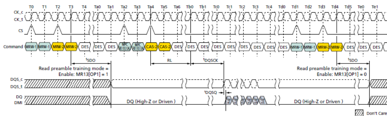
Figure 141. Read Preamble Training
