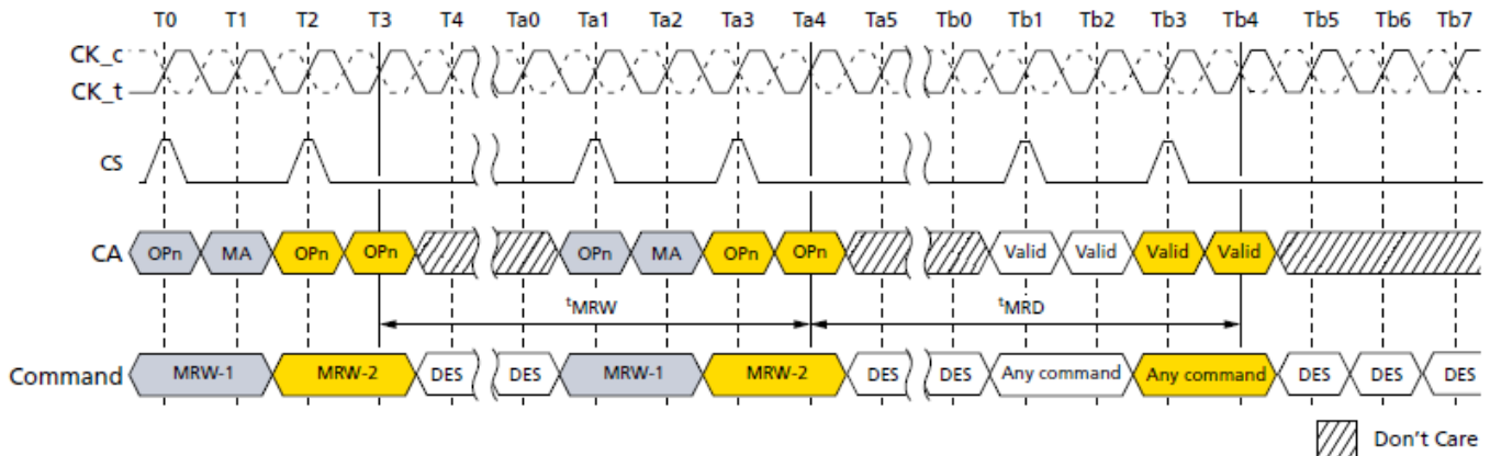
Figure 90. MODE REGISTER WRITE Timing
