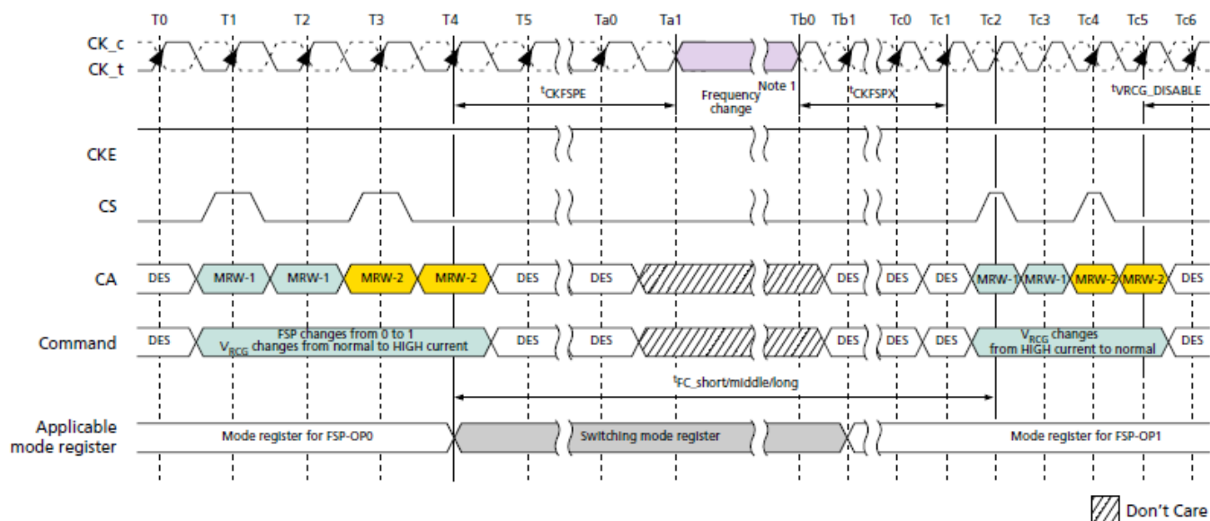
Figure 131. Frequency Set Point Switching Timing
