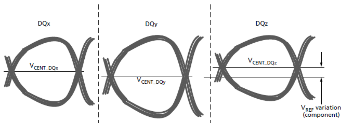
Figure 169. Across Pin V_{REF} DQ Voltage Variation
