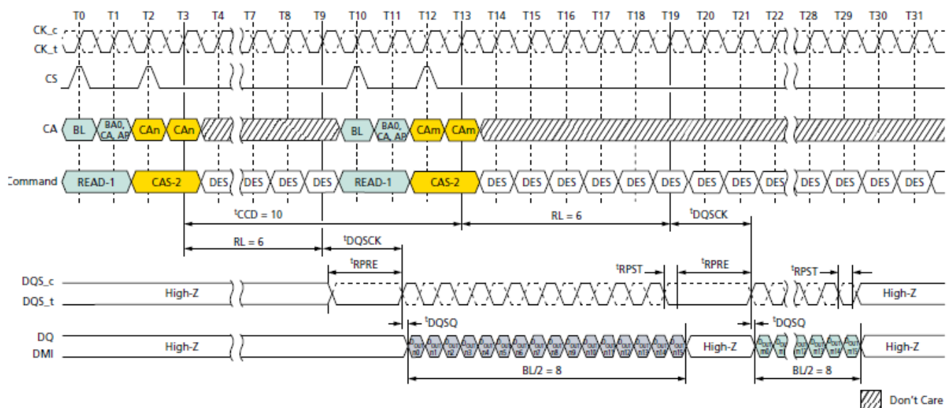
Consecutive READ: t'_{CCD} = \text{MIN} + 2 , Preamble = Static, 0.5n\text{CK} Postamble
