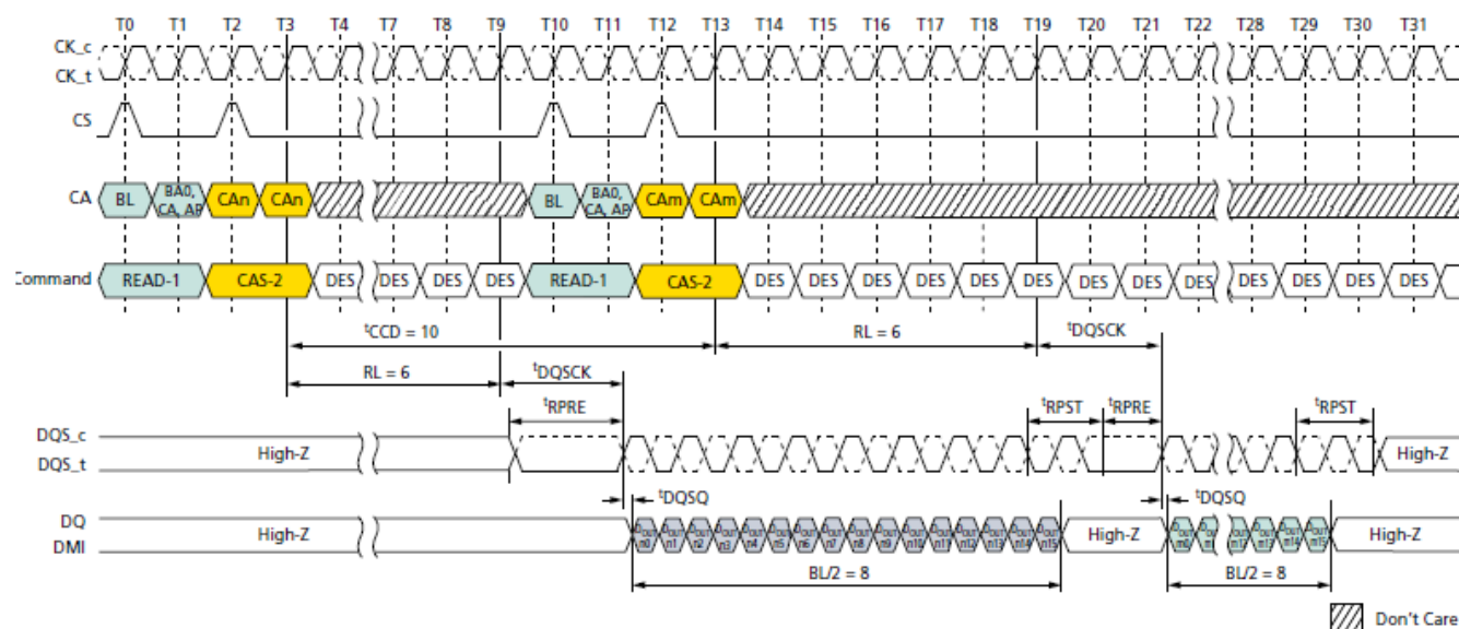
Consecutive READ: t'_{CCD} = \text{MIN} + 2 , Preamble = Static, 1.5n\text{CK} Postamble
