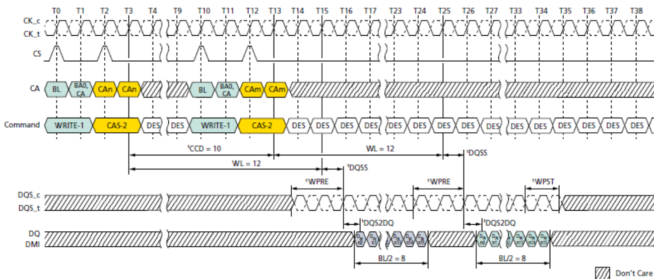
Consecutive WRITE: t_{CCD} = \text{MIN} + 2 , 1.5nCK Postamble
