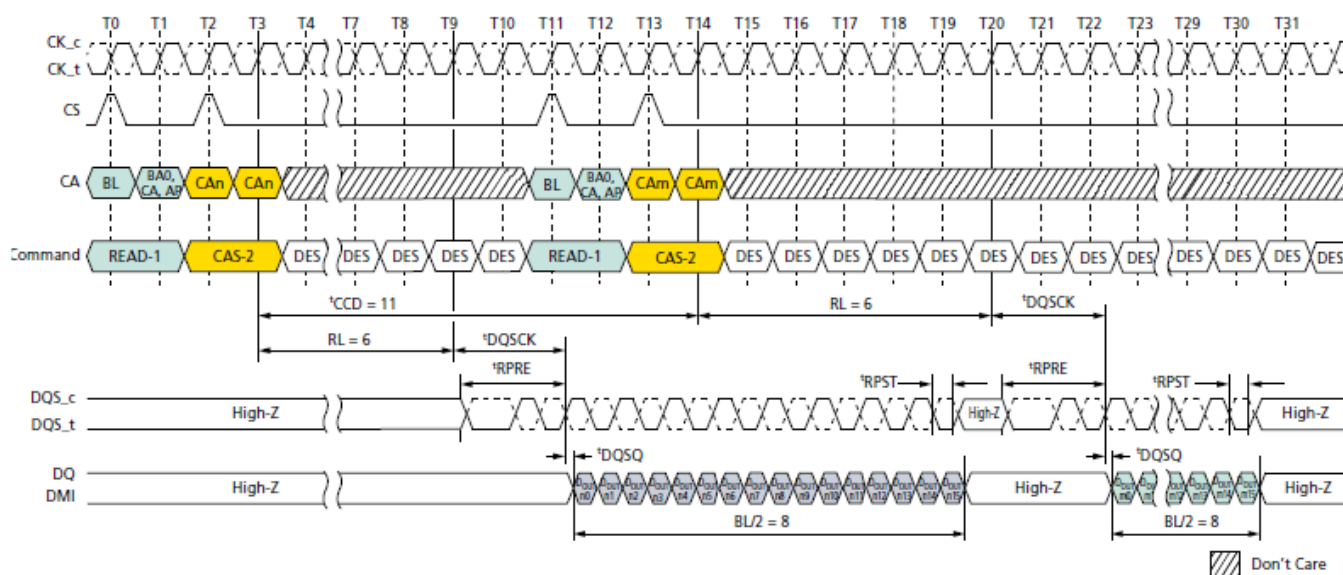
Consecutive READ: t'_{\text{CCD}} = \text{MIN} + 3 , Preamble = Toggle, 0.5nCK Postamble
