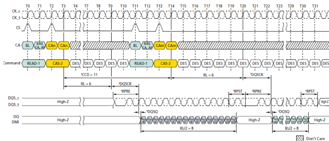
Consecutive READ: t'_{\text{CCD}} = \text{MIN} + 3 , Preamble = Toggle, 1.5nCK Postamble
