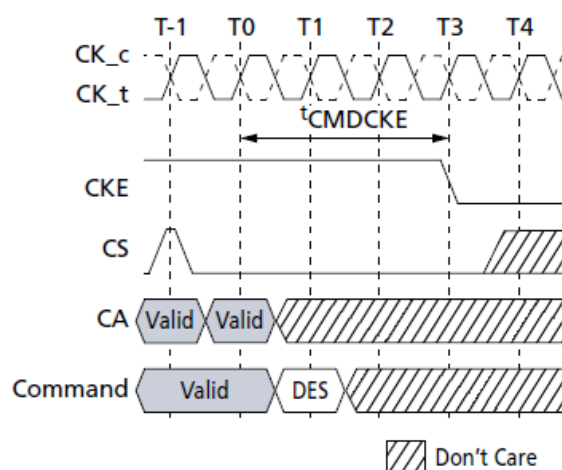
t_{\text{CMDCKE}} Timing
