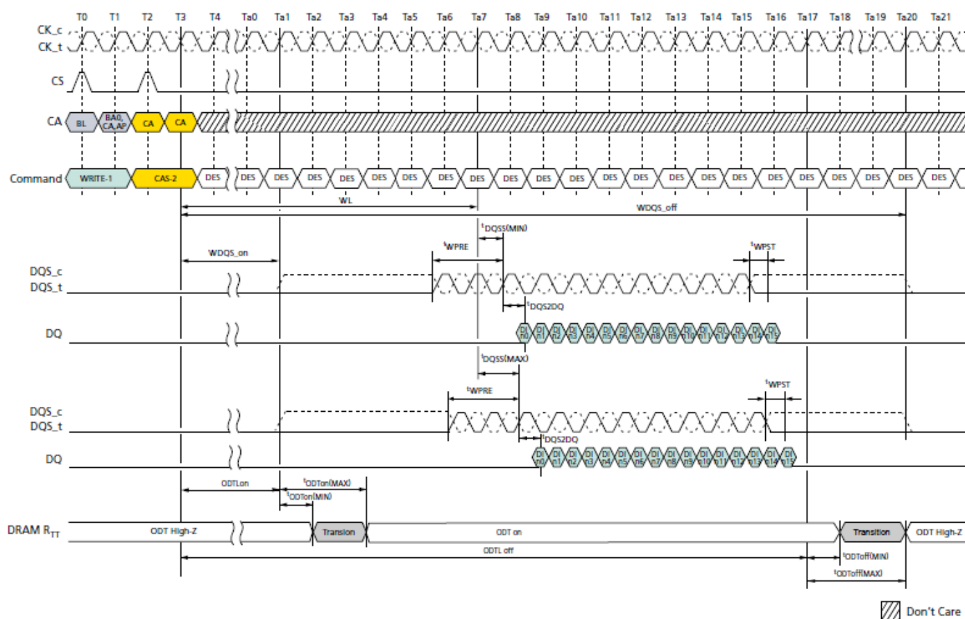
Figure 30. Burst WRITE Operation
