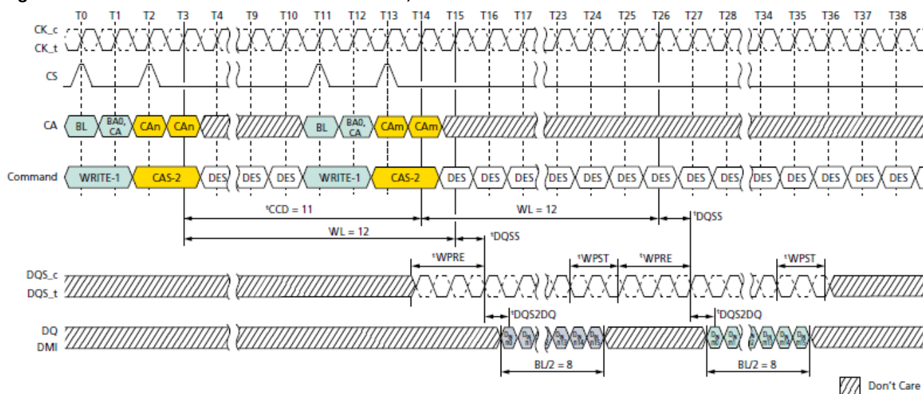
Figure 54. Consecutive WRITE: t_{CCD} = MIN + 3, 1.5nCK Postamble
