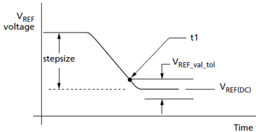
Figure 103. V_{REF(DQ)} Single-Step Size Decrement
