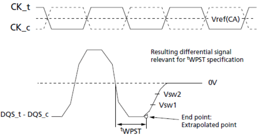
Figure 24. Method for Calculating tWPST Transitions and Endpoints
