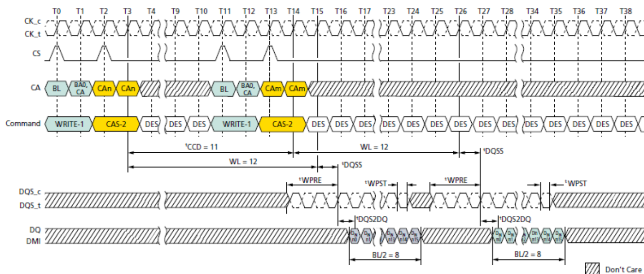
Figure 53. Consecutive WRITE: t_{CCD} = MIN + 3, 0.5nCK Postamble
