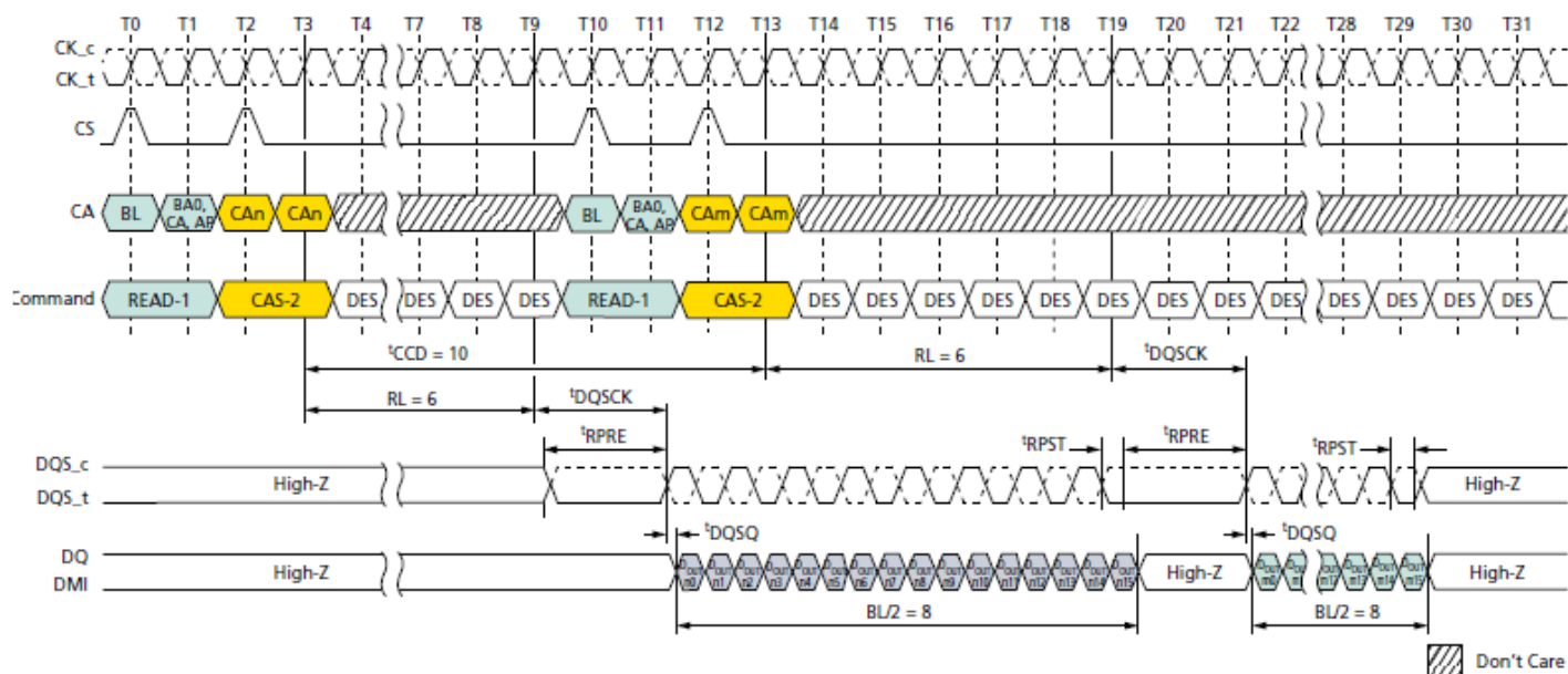
Figure 41. Consecutive READ: t_{CCD} = MIN + 2 , Preamble = Static, 0.5nCK Postamble
