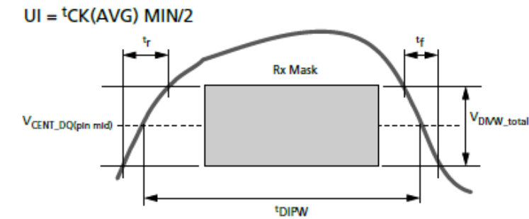
Figure 170. DQ t_{DIPW} and SRIN_dIVW Definition for Each Input Pulse
