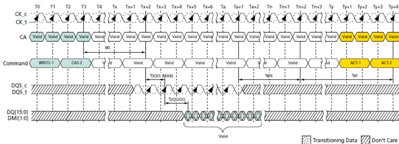
Figure 61. Burst WRITE With Auto Precharge – BL16, 2nCK Preamble, 0.5nCK Postamble
