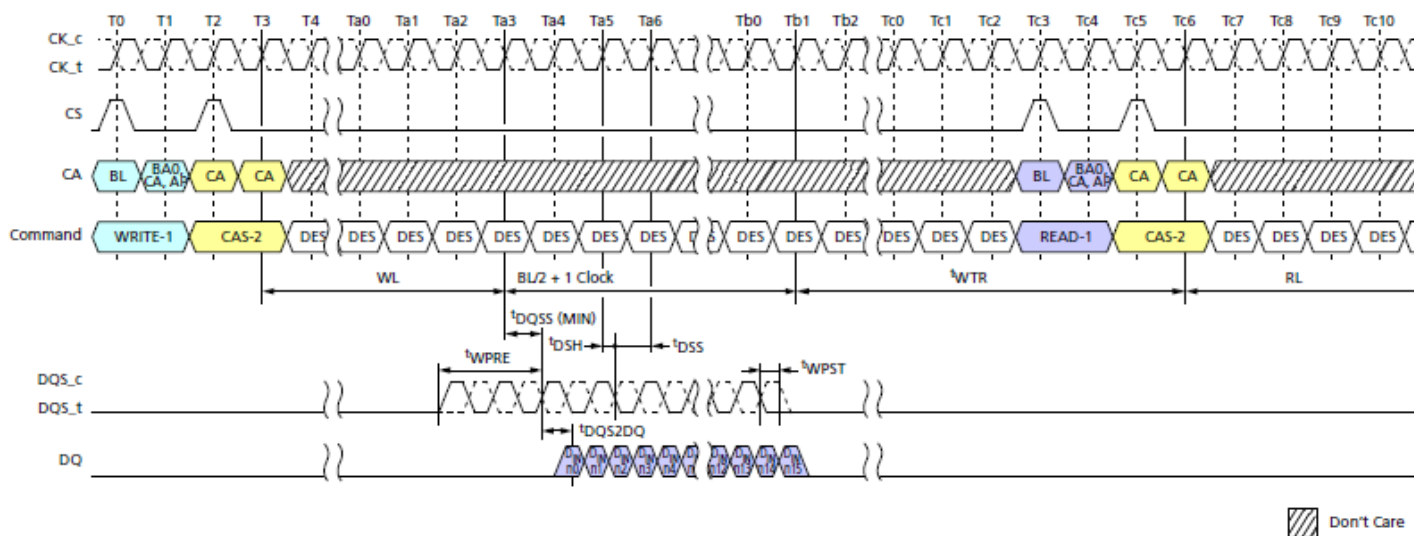
Figure 21. Burst Write Followed by Burst Read
