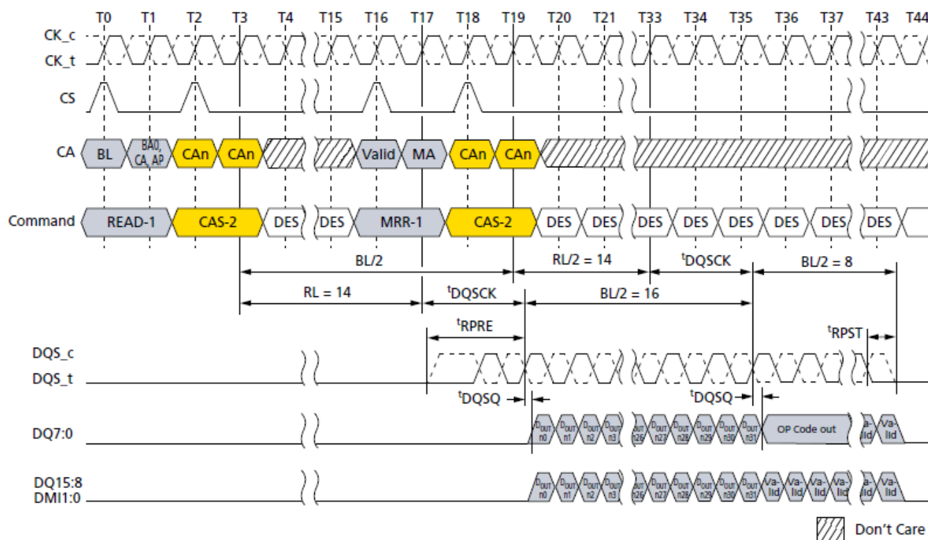
Figure 86. READ-to-MRR Timing
