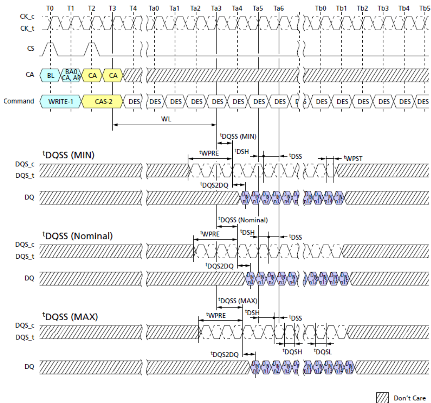
Figure 22. Write Timing
