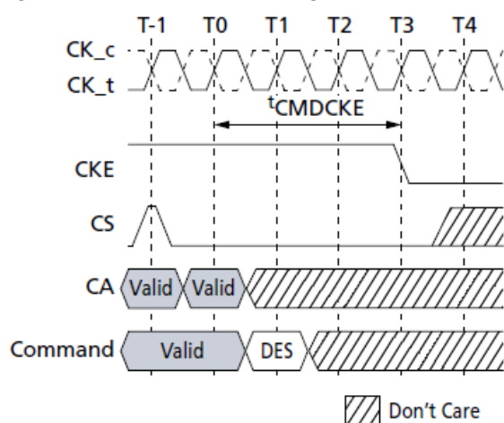
Figure 159. t_{CMDCKE} Timing
