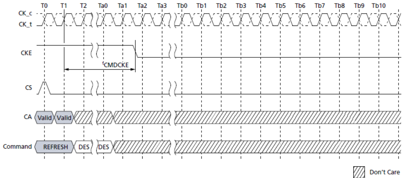
Figure 79. Refresh Entry to Power-Down Entry
