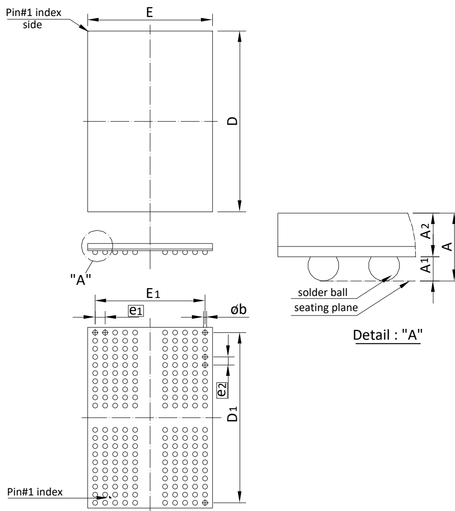
Figure 182. 200-BALL (10x14.5 mm)
