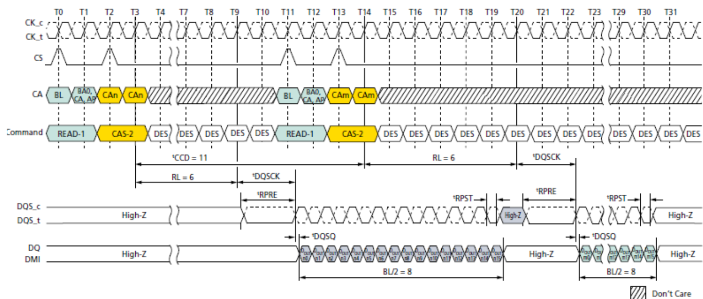
Figure 45. Consecutive READ: t_{CCD} = MIN + 3 , Preamble = Static, 0.5nCK Postamble
