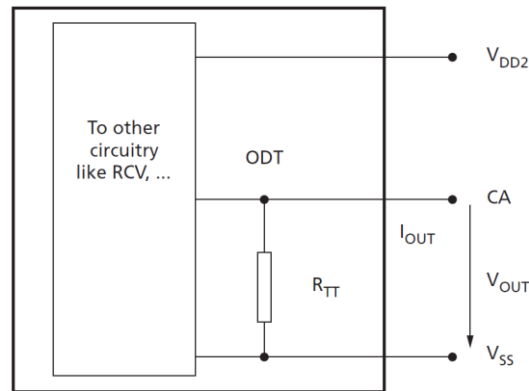
Figure 176. ODT for CA
