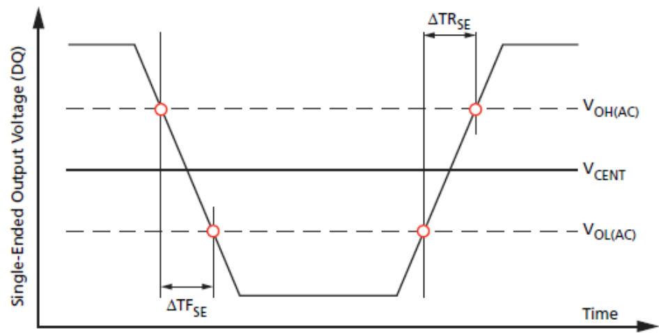
Figure 153. Single-Ended Output Slew Rate Definition
