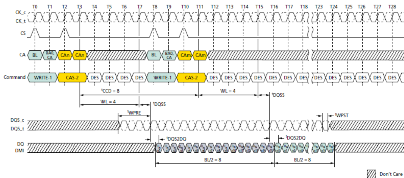
Figure 46. Seamless WRITE: t_{CCD} = \text{MIN}, 0.5n\text{CK} Postamble
