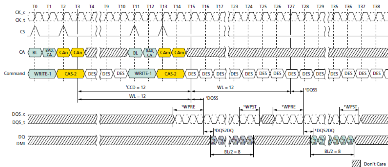
Figure 55. Consecutive WRITE: t_{CCD} = \text{MIN} + 4, 1.5nCK Postamble
