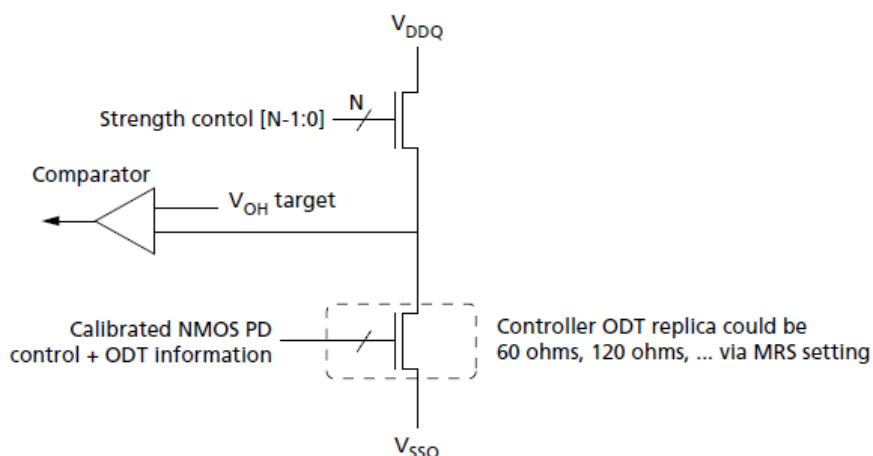
Figure 158. Pull-Up Calibration
