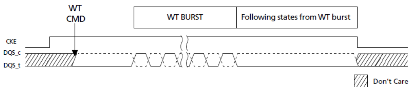
Figure 29. WDQS Control Mode 1
