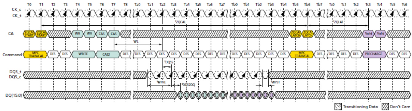
Figure 129. ZQCAL Timing
