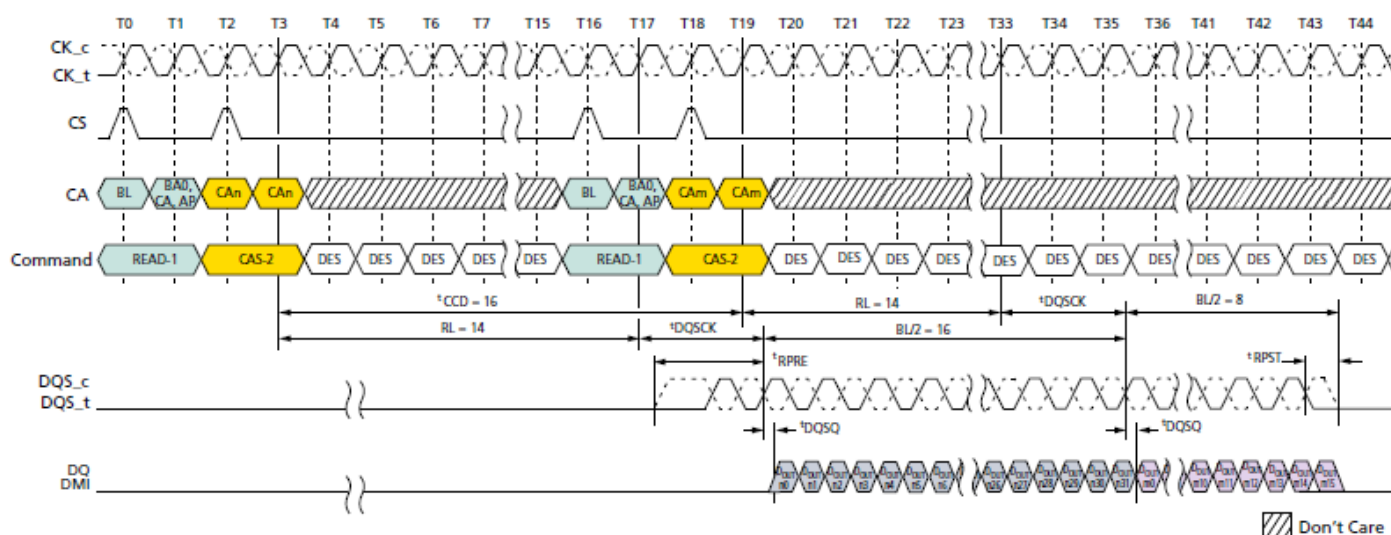
Figure 12. Burst Read Timing
