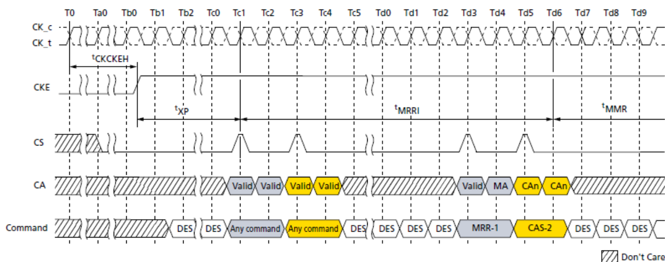
Figure 88. MRR Following Power-Down
