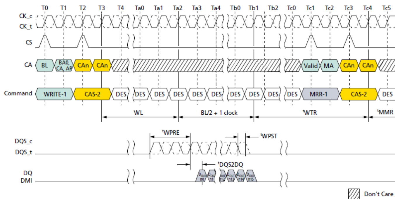
Figure 87. WRITE-to-MRR Timing
