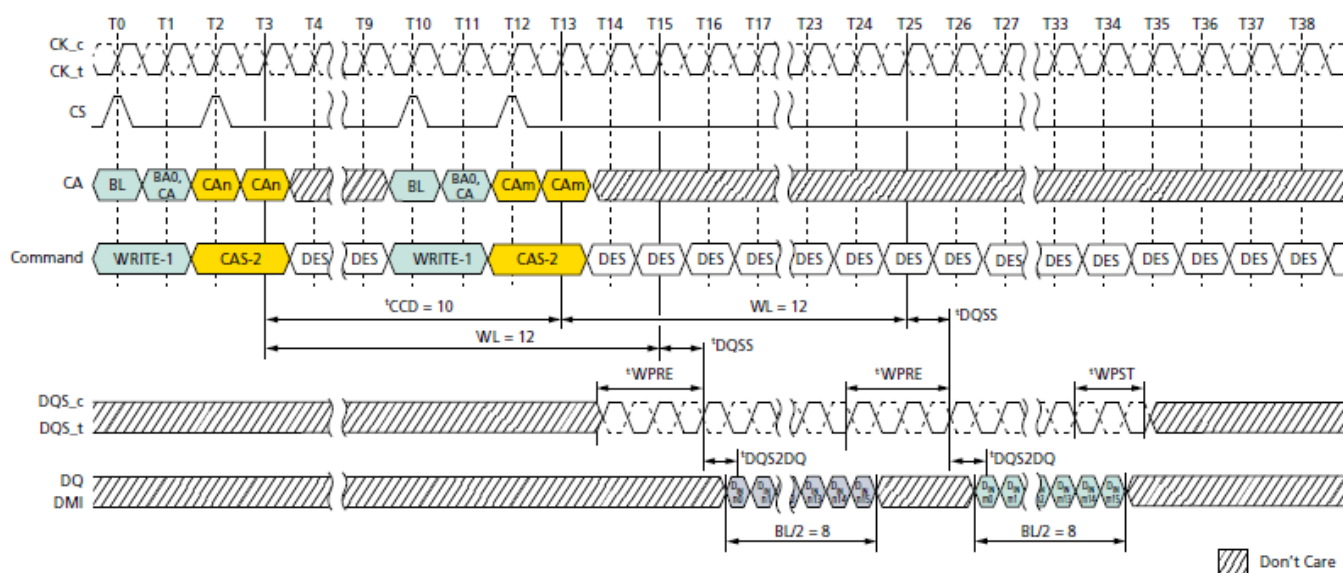
Figure 52. Consecutive WRITE: t_{CCD} = \text{MIN} + 2, 1.5nCK Postamble
