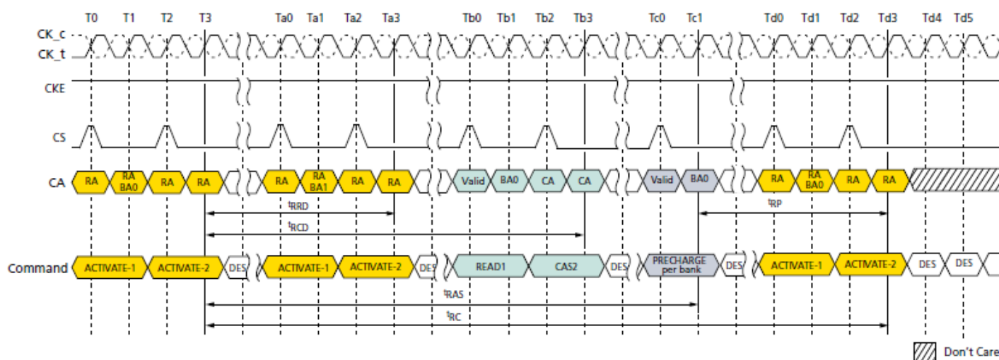
Figure 6. ACTIVATE Command
