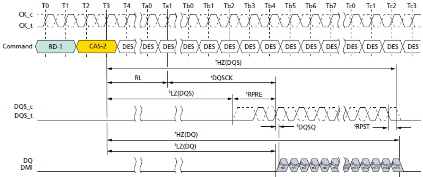
Figure 15. Read Timing
