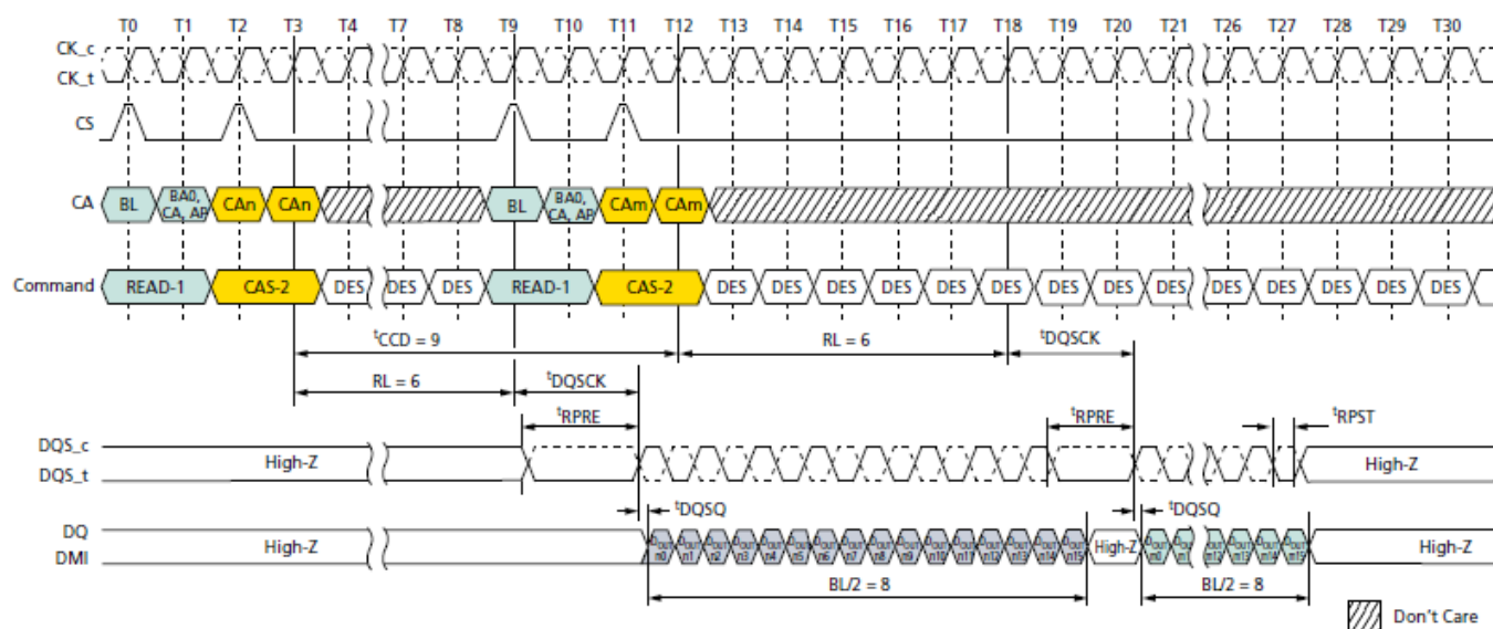
Figure 37. Consecutive READ: t_{CCD} = MIN + 1 , Preamble = Static, 0.5nCK Postamble
