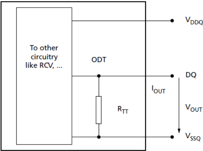
Figure 136. Functional Representation of DQ ODT
