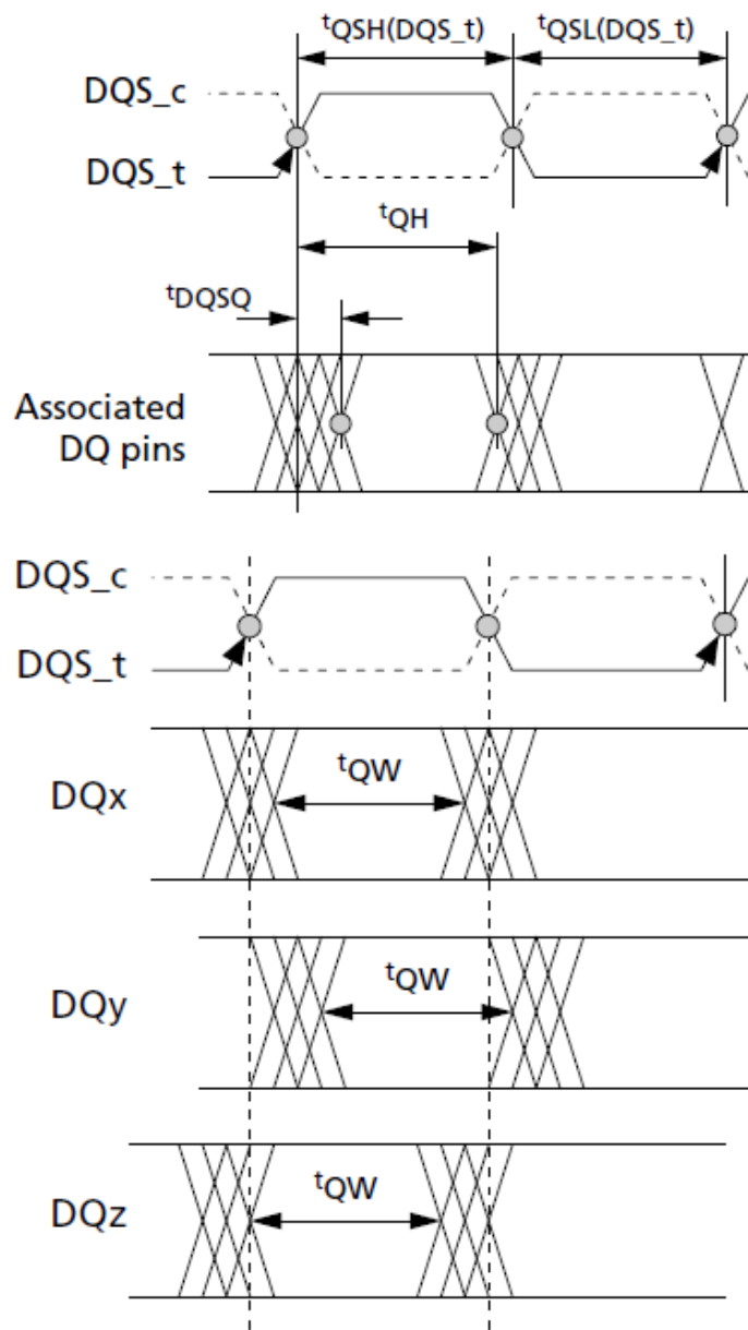
Figure 166. Read Data Timing Definitions – t_{QH} and t_{DQSQ} Across DQ Signals per DQS Group
