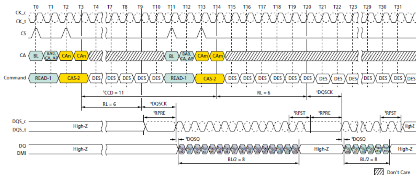
Figure 44. Consecutive READ: t_{CCD} = MIN + 3 , Preamble = Static, 1.5nCK Postamble
