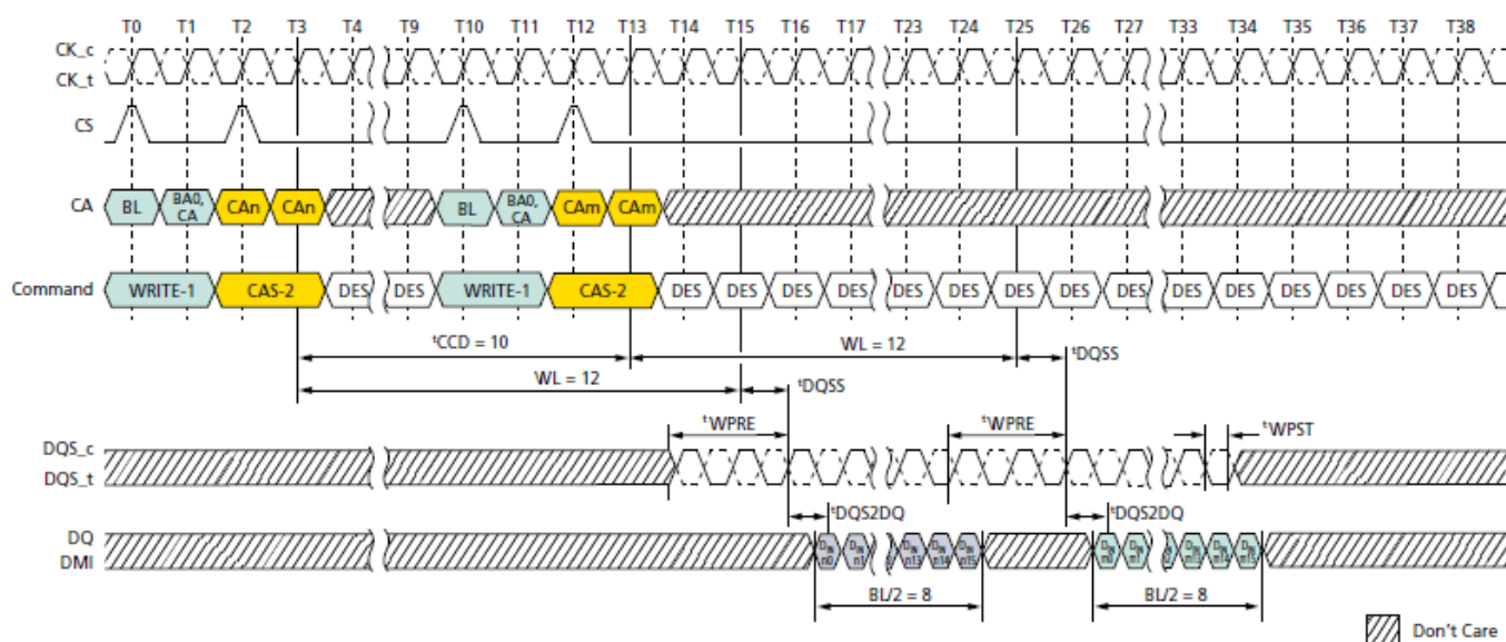
Figure 51. Consecutive WRITE: t_{CCD} = \text{MIN} + 2, 0.5nCK Postamble
