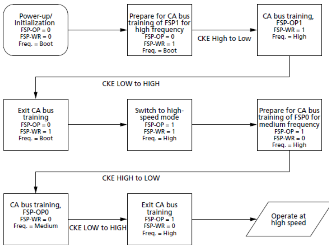
Figure 131. Training for Two Frequency Set Points
