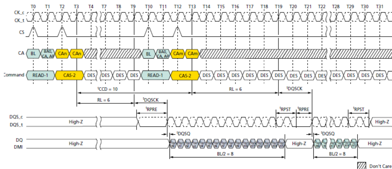
Figure 40. Consecutive READ: t_{CCD} = MIN + 2 , Preamble = Static, 1.5nCK Postamble
