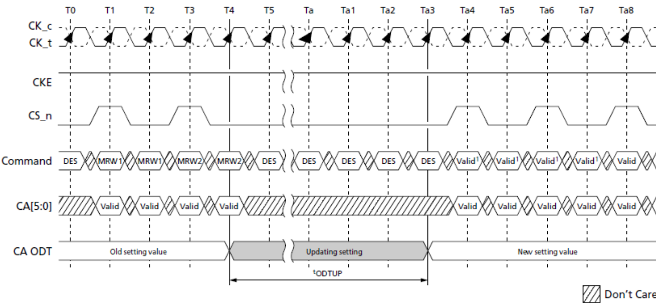
Figure 135. ODT for CA Setting Update Timing in 4-Clock Cycle Command
