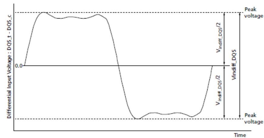
Figure 148. DQS Differential Input Voltage
