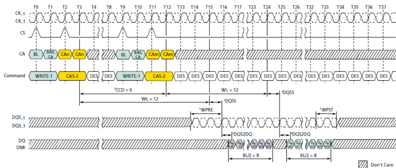
Figure 50. Consecutive WRITE: t_{CCD} = \text{MIN} + 1, 1.5nCK Postamble
