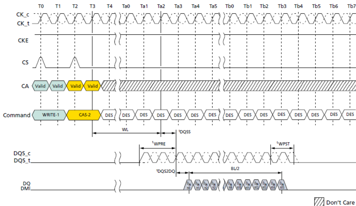
Figure 11. DQS Write Preamble and Postamble – 1.5nCK Postamble
