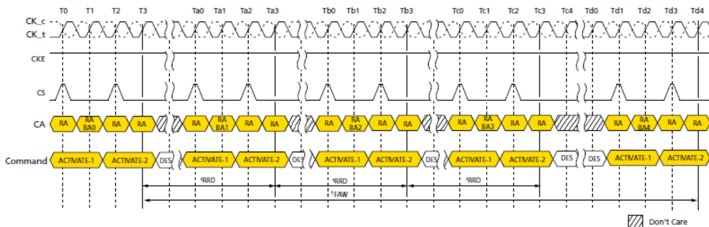
Figure 7. t FAW Timing
