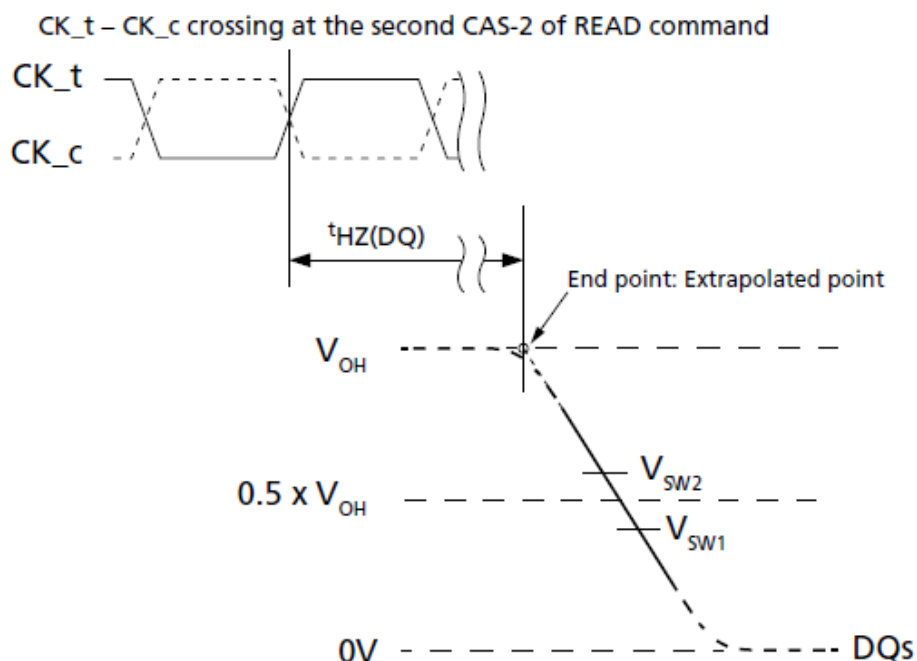
Figure 19. t_{\text{HZ}}(\text{DQ}) Method for Calculating Transitions and Endpoint
