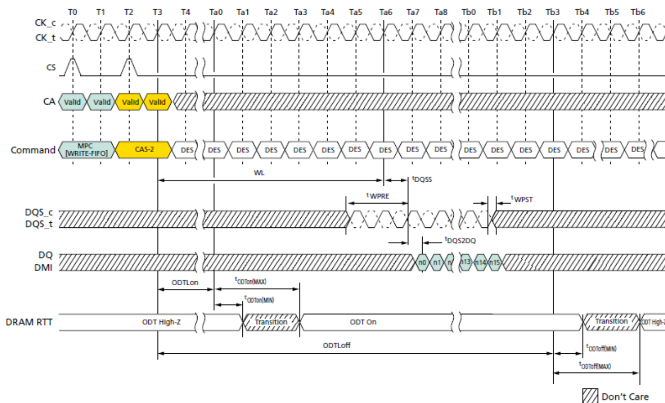
Figure 123. MPC[WRITE-FIFO] with DQ ODT Timing
