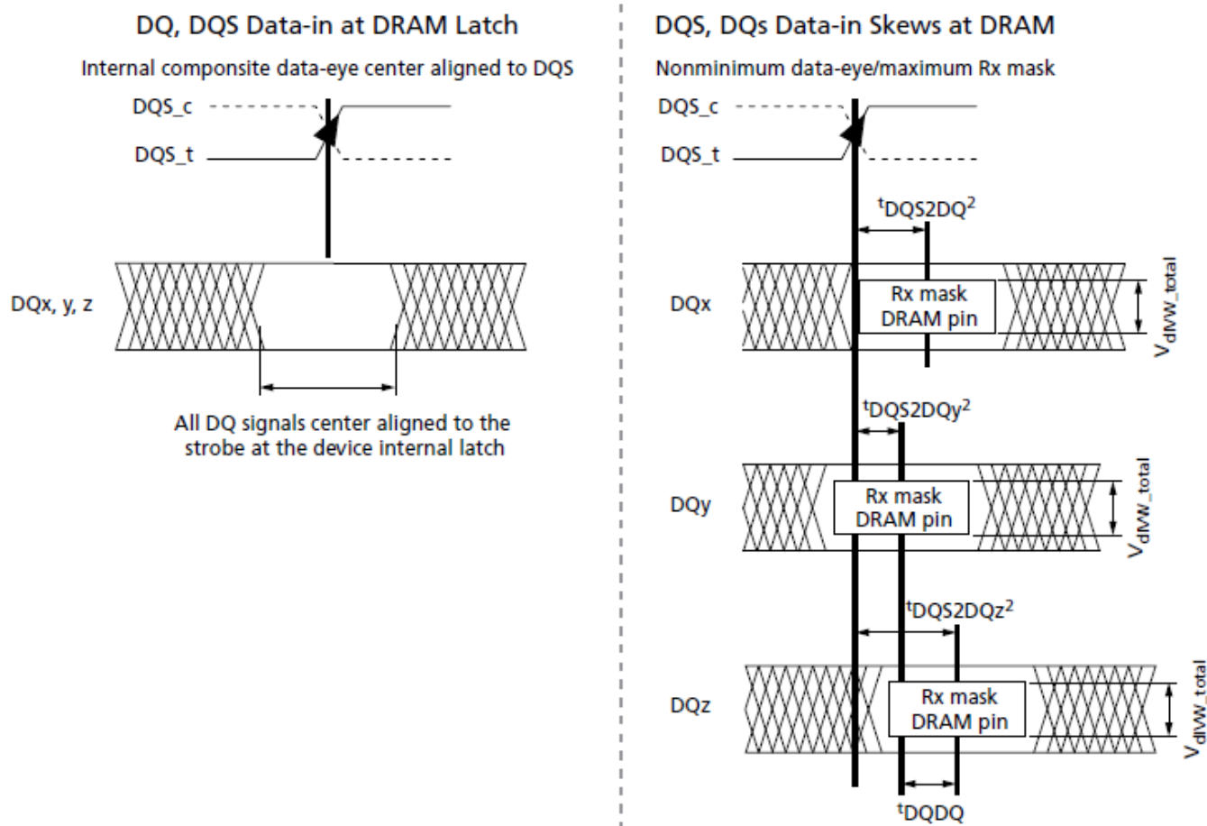
Figure 169. DQ-to-DQS t_{DQS2DQ} and t_{DQDQ}
