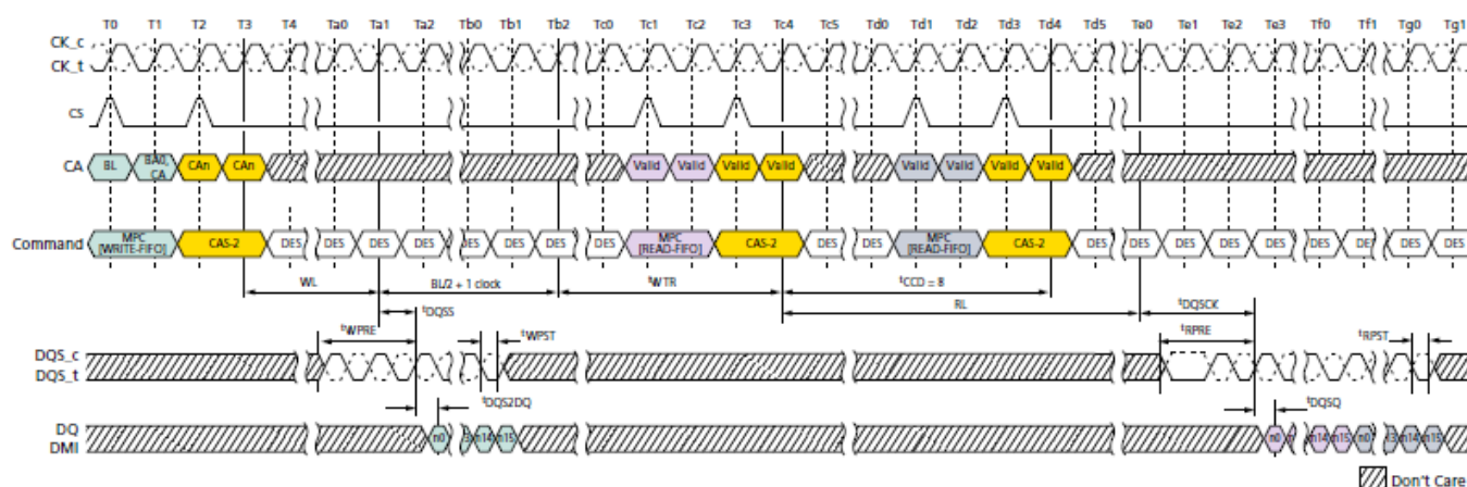
Figure 121. MPC[WRITE-FIFO]-to-MPC[READ-FIFO] Timing
