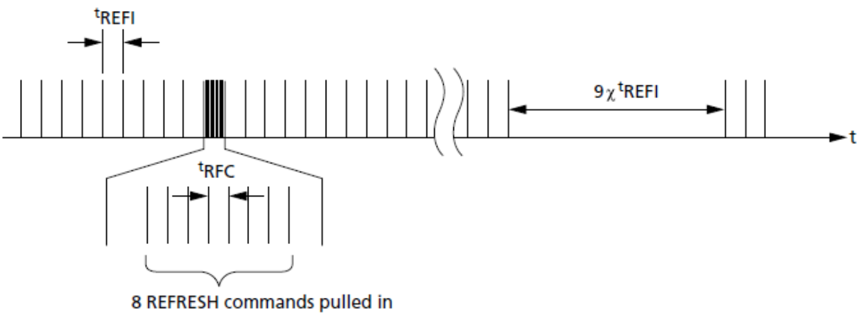
Figure 67. Pulling in REFRESH Commands (Example)
